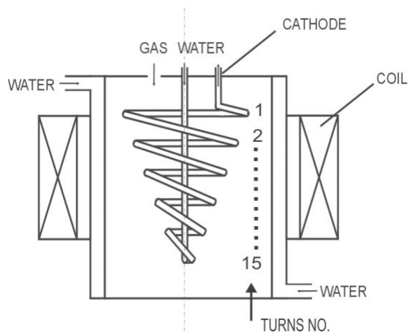
Fig. 4. The SPIRARC plasma reactor cross section
