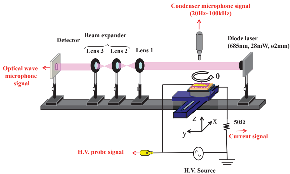
Fig. 3. Experimental setup to detect the sound of coplanar DBD using OWM-CT.
