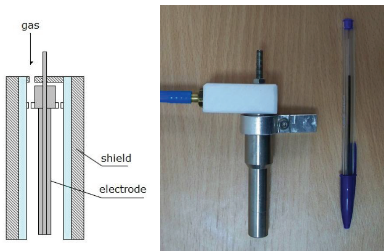
Fig.1. Schema and photo of atmospheric pressure plasma jet.
