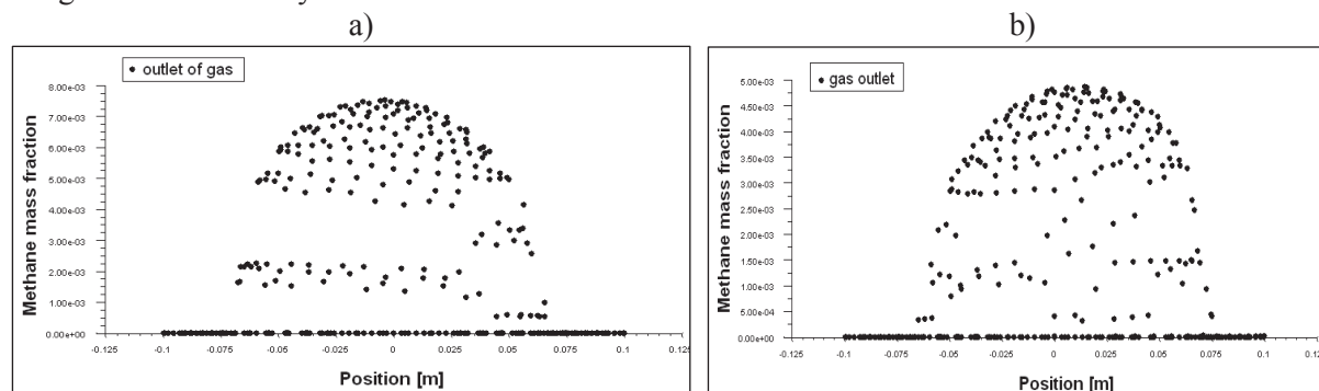
Fig.5 The distribution of methane mass fraction at the outlet of reactor calculated numerically including the methane oxidation: a) – methane was introduced through the outer nozzle; b) – methane was introduced through the central mixing nozzle.
