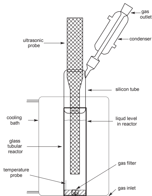
Figure 1: Reaction system setup (with high immersion level of the ultrasound probe into the liquid).
