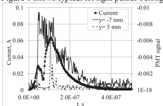
Figure 6. Current and IR light pulses in the positive half cycle at positions y = -7 mm and y = 5 mm.
