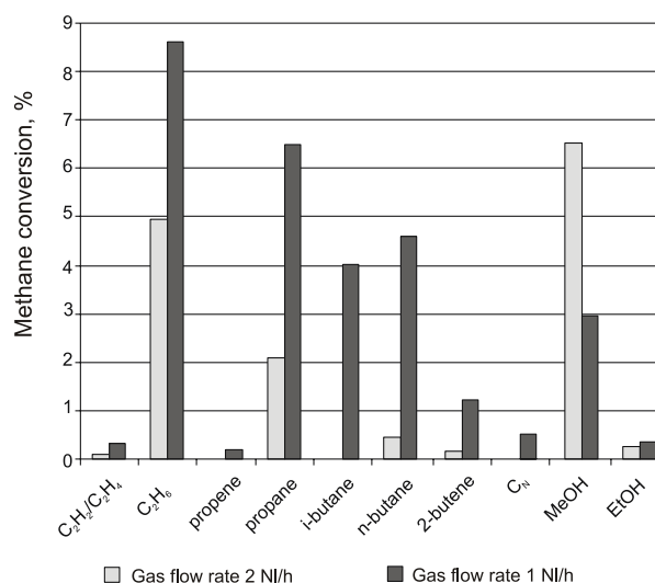
Fig. 6. Effect of the gas flow rate on conversion of methane to hydrocarbons and alcohols. Molar ratio [CH 4 ]: [O 2 ]=3:1, Power – 19 W, argon conc. 50%.
