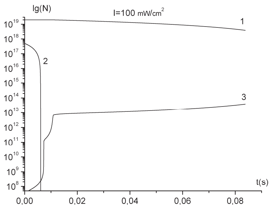
Fig.3 Time dependence of concentrations N(\text{cm}^{-3}) : 1- non injured nucleotides, 2-glutathione, 3- \bullet OH radicals. I=100 \text{ mW/cm}^2 .
