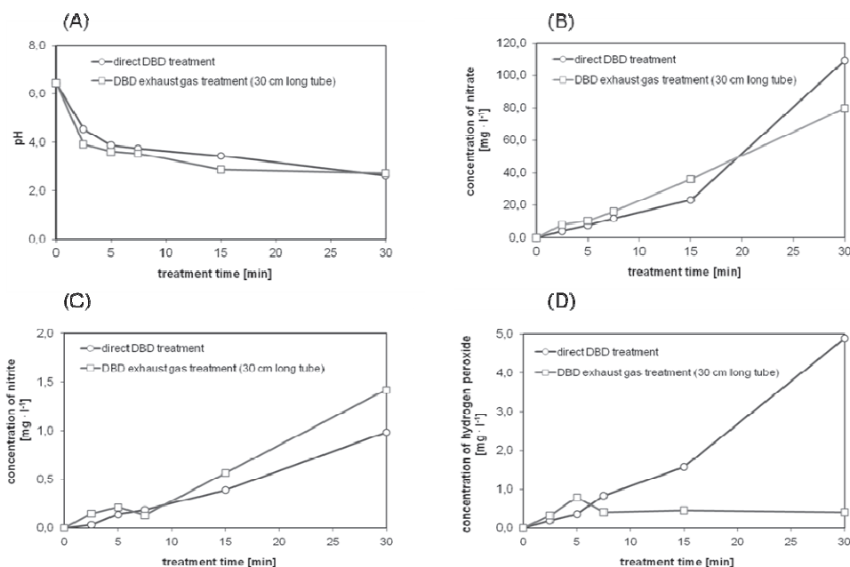
Fig. 5: Analytical results for pH (A), \text{NO}_3^- (B), \text{NO}_2^- (C) and \text{H}_2\text{O}_2 (D) in DBD treated water (-o-) or DBD exhaust gas treated water (-□-) in air.
