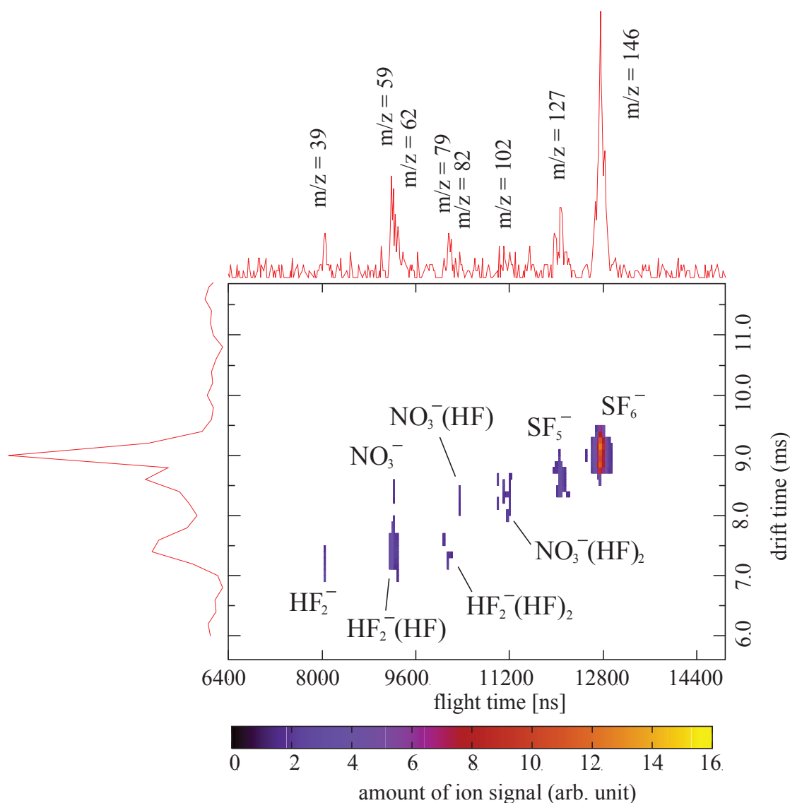
Fig. 1. Two dimensional IMS-MS map of negative ions observed in \text{SF}_6/\text{N}_2 mixture.
