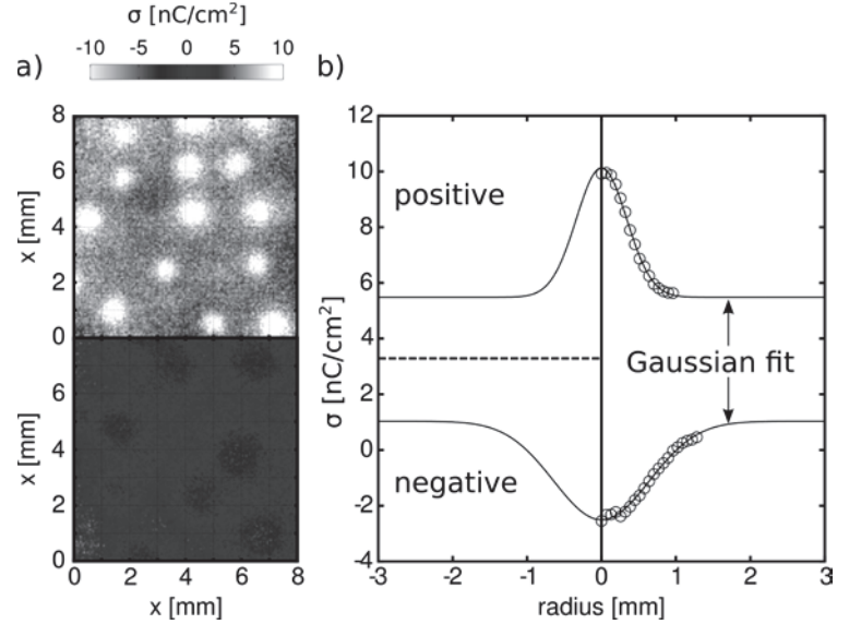
Fig. 5. Charge distribution in the filamentary mode (90vol.%He and 10vol.%N 2 mixture) of positive (bright spots) and negative surface (dark spots) charges in the positive and negative half-period, respectively. b) Radial profile of positive and negative surface charges, FWHM: \sigma_+ = 0.9 \text{ mm} and \sigma_- = 1.6 \text{ mm} , respectively. p = 500 \text{ mbar} , \nu = 2 \text{ kHz} , U = 0.91 \text{ kV} .
