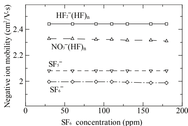
Fig. 4 Negative ion mobilities of \text{HF}_2^-(\text{HF})_n , \text{NO}_3^-(\text{HF})_n , \text{SF}_5^- , and \text{SF}_6^- against \text{SF}_6 concentration.
