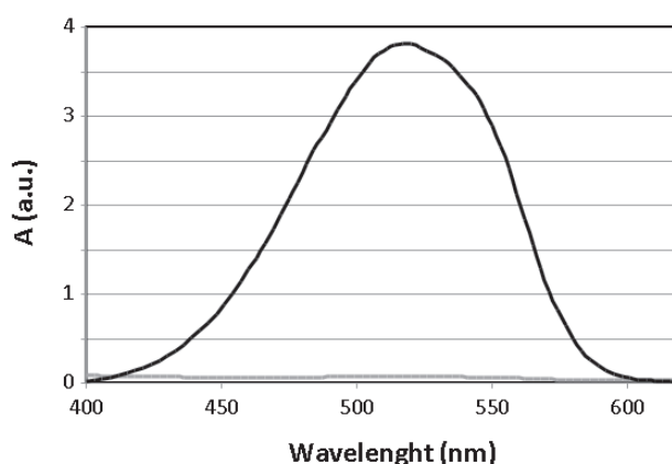
Fig. 2. The absorption spectra of methyl red (MR) in the spectral range 400-620 nm (black line – spectra of the untreated MR dye containing water solution, grey line – spectra of the discharge treated MR dye containing water solution).
