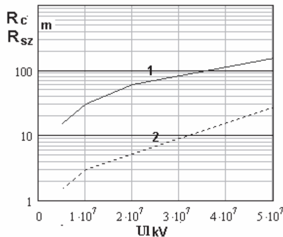
Fig.1 The calculated dependences R_{sz} (1) and R_c (2) from the potential of head.
