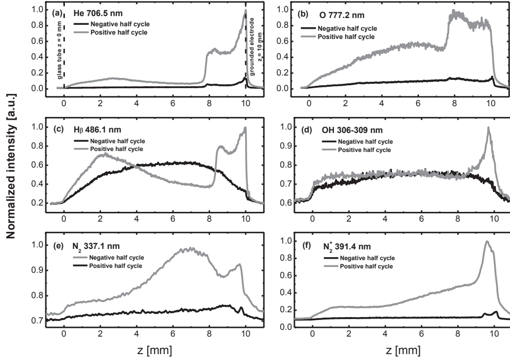
Fig. 4. Spatially resolved intensity distributions of various emissions for the positive and the negative current peaks of the jet.
