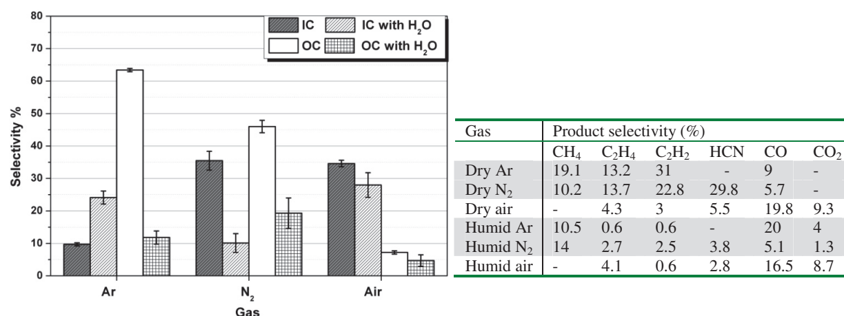
Fig 3. Dry and humid gas effect to the selectivity of inorganic (IC) and organic carbon (OC) end-products
