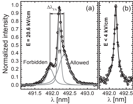
Fig. 6. Typical \pi -polarized spectra of He I 492.19 nm line recorded from the plasma jet for (a) positive and (b) negative current pulse.
