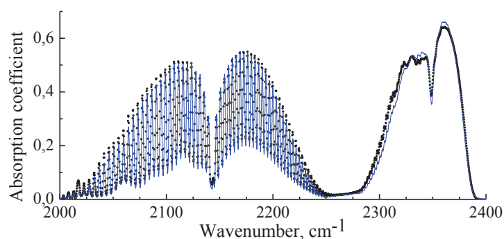
Fig. 4. Experimental (doted) and calculated (solid) absorption IR-spectra of CO and CO 2 .
