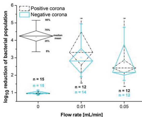
Fig. 6. Reduction of bacterial population on plastic samples by corona discharges with electro-spraying for different flow rates (exp. time - 2 min)
