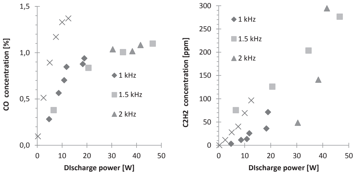
Fig. 8. Carbon monoxide concentration produced in \text{CH}_4:\text{CO}_2 (70%:30%) gas mixture as a function of discharge power for different AC sine frequency and for nanosecond negative pulses.
