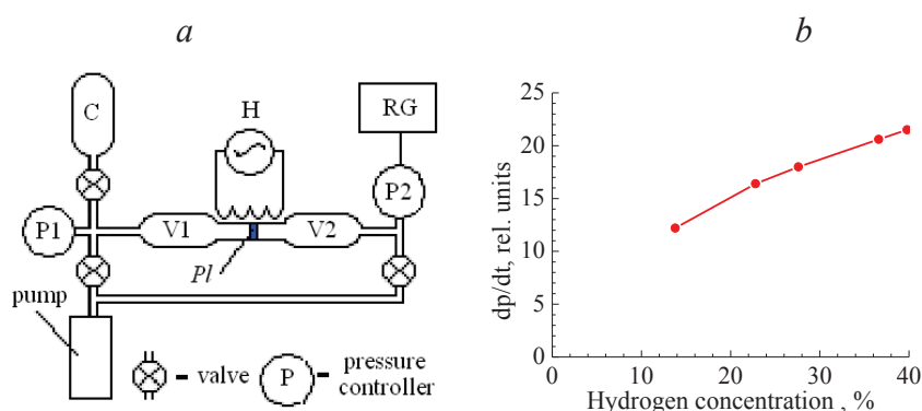
Fig. 2. Schematic of system for the hydrogen collection. PI – palladium inlet valve, V1 and V2 – volumes, C – cylinder, H – heater, RG – leakage recorder, PI – palladium membrane.
