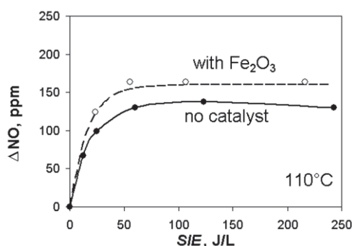
Fig. 3. The difference between inlet and outlet NO concentrations ( \Delta NO ) in hybrid plasma-catalytic reactor as a function of SIE at 110^\circ C if the concentration of NO at the inlet was 450 ppm.
