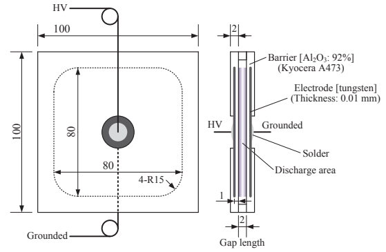
Fig. 2. DBD device.
