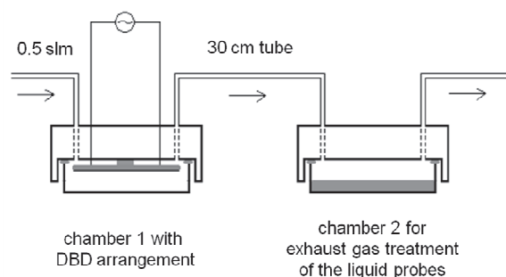
Fig. 3. Experimental setup of DBD exhaust gas treatment.
