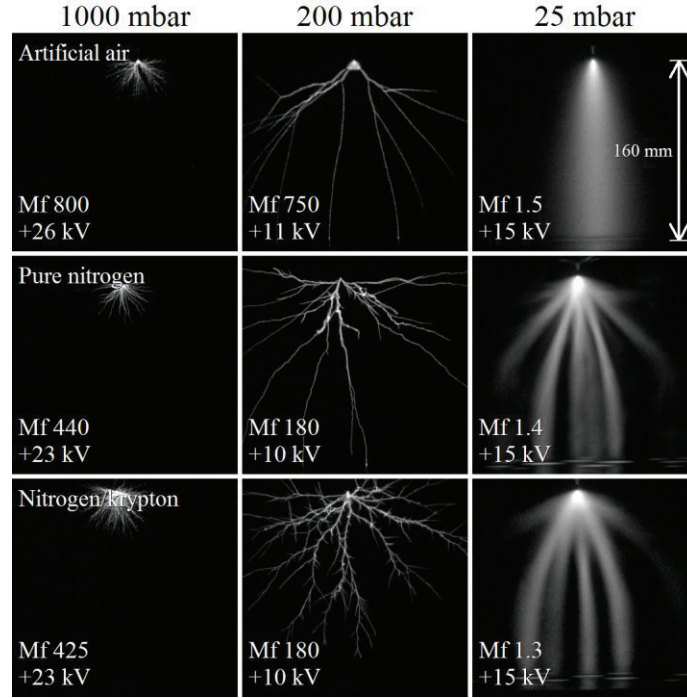
Figure 2. Overview of streamer discharges produced with the C-supply for our three gas mixtures (rows), at pressures of 1000, 200 and 25 mbar (columns) and 1 Hz repetition frequency. All measurements have a long exposure time and therefore show one complete discharge event, including transition to glow for 25 mbar. The multiplication factor (Mf) gives an indication of the real intensity of the discharge. The length scale is indicated with the arrow at the top right. Measurements in artificial air and nitrogen were previously published in [3].
