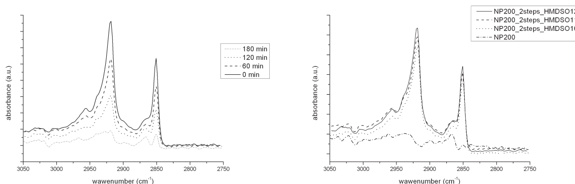
Fig. 4. FTIR spectra of C-H bonds in stearic acid: NP200_2steps_HMDSO10 on the left (a) and the comparison between the three composite films at 60 minutes of UV-light exposure on the right (b).
