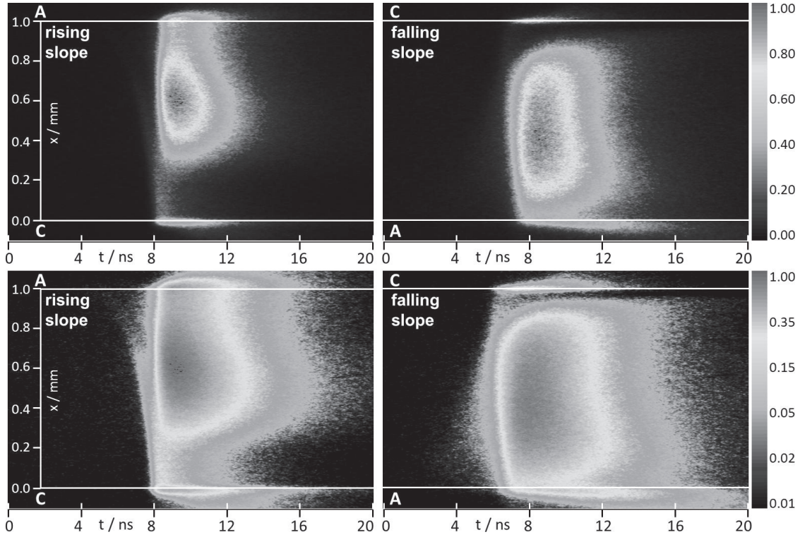
Fig. 3: Spatio-temporal development of MDs along the axis during rising and falling slopes (same conditions as in figure 2), accumulation of 1,000 MDs in linear (top row) and logarithmic intensity scale (bottom row).
