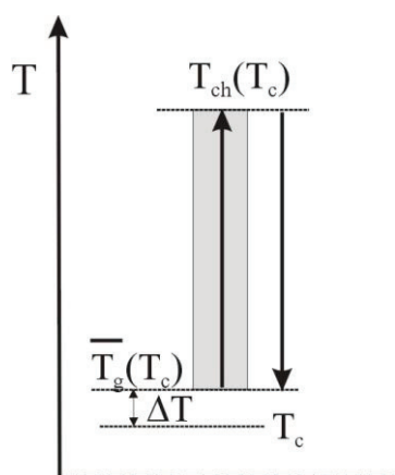
Fig. 3 (left). Schematic diagram of the temperatures in the microdischarge channel under stationary state conditions in the discharge gap ( T_c , P , V_0 = \text{const} ). The increase of temperature in the microdischarge channel has no influence on the average temperature of the gas T_g .
