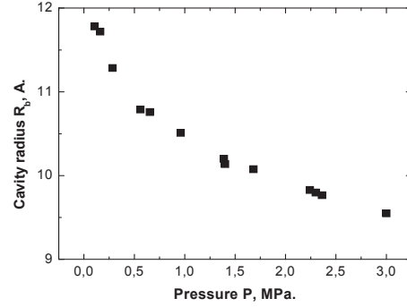
Fig. 4. Radius of cavities for different pressures recalculated from the experimental data for the line width (Fig. 2).
