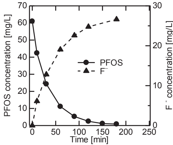
Fig. 4 Time variations in PFOS and \text{F}^- concentrations during oxygen plasma treatment.
