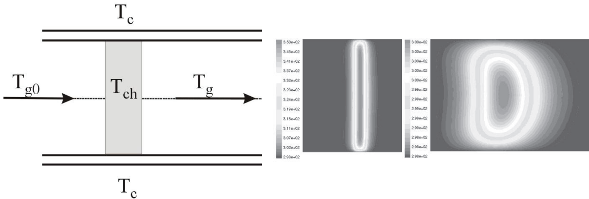
Fig. 5. Temperatures in the discharge gap according the model [1] (a) and calculated gas temperature fields after microdischarge decay: 0.1 ms (b) and 2 ms (c) [8,9]. The temperature scale is various. T_{g0} – inlet gas temperature, T_{ch} – temperature in discharge channel, T_g – temperature of a gas after microdischarge occurrence, T_c – cooling liquid temperature.
