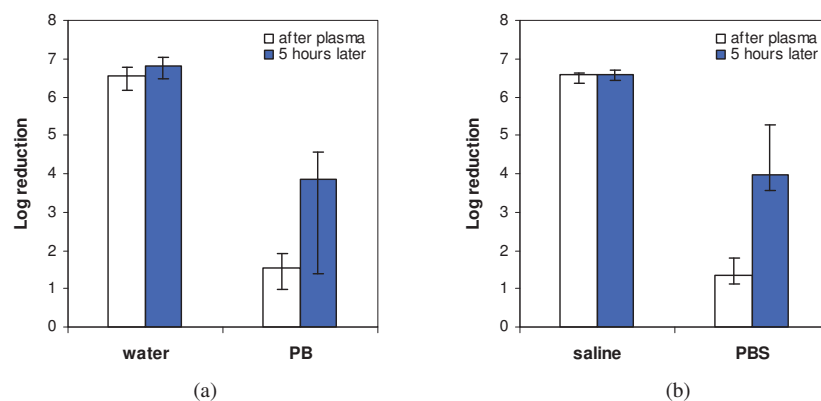
Fig. 4. E. coli inactivation of log reduction after plasma treatment and 5 h later obtained in: (a) water (pH~3.3 after plasma and ~3.4 5h later, respectively) and PB solutions (pH~6.2 and ~5.8, respectively); (b) saline solution (pH~2.8 after plasma and ~2.9 5h later, respectively) and PBS (pH~5.6). Medians with error bars showing 25 and 75 percentiles.
