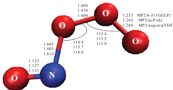
Transition State for NO + O 3 reaction
