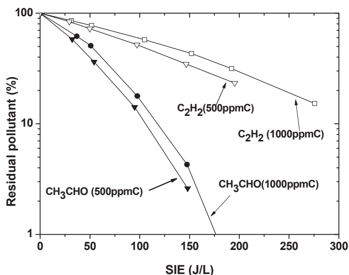
Fig. 3. Comparison of the degradation of both pollutants when individually dilute in a 94.5% N 2 /5%O 2 gas flow for two different initial concentrations (500 and 1000 ppmC).
