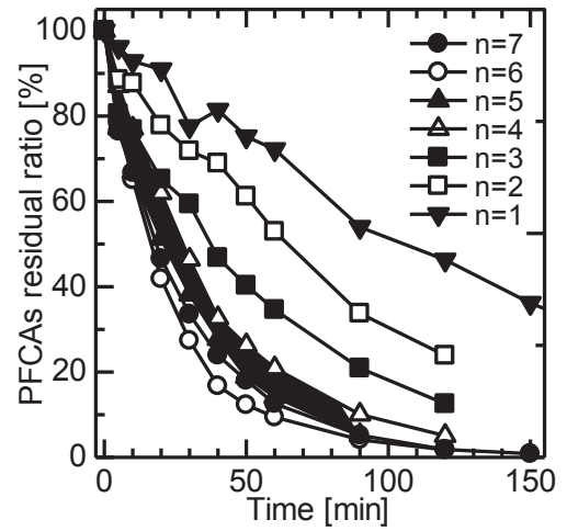
Fig. 5 Time variations in concentrations of PFCAs ( n = 1-7 ).
