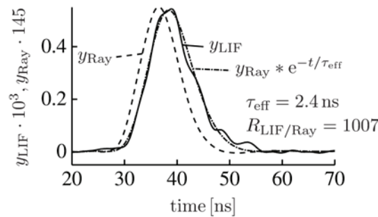
Fig. 2: Time dependent Rayleigh and LIF signal as well as the fitted convolution of the Rayleigh signal with an exponential decay to the LIF signal.
