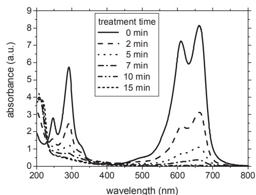
Fig. 4. UV-visible spectra of MB aqueous solution, untreated and treated by plasma up to 15 min.
