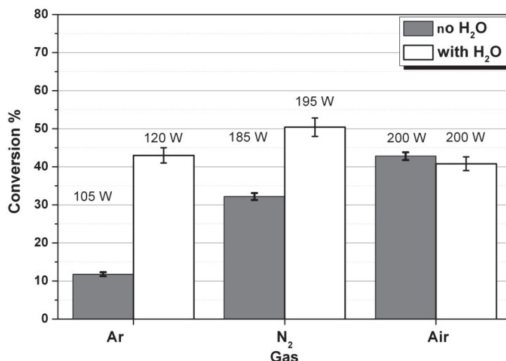
Fig 2. Dodecane conversion in dry and humid (RH=65%) argon, nitrogen and air gliding arc discharge
