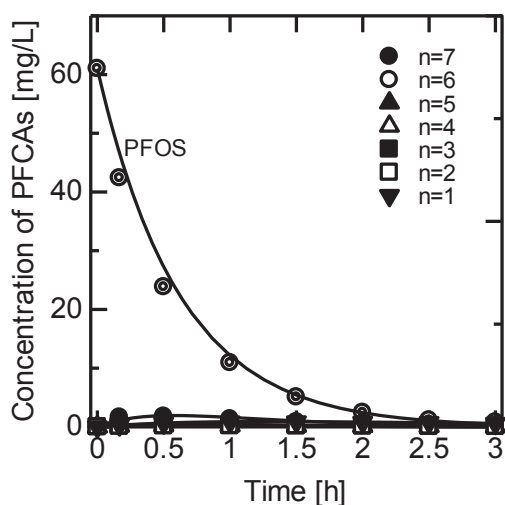
Fig. 6 Time variation in PFOS and PFCA concentrations and calculated PFOS concentrations (solid lines).
