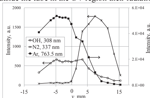
Figure 5. Intensity distribution of Ar line and OH, N_2 bandheads along the jet axis.
