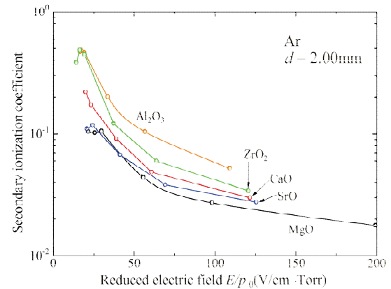
Fig. 15 Secondary ionization coefficient.
