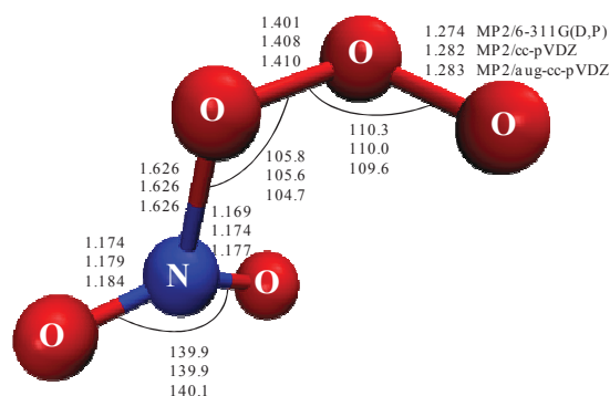
Transition State for NO 2 + O 3 reaction
