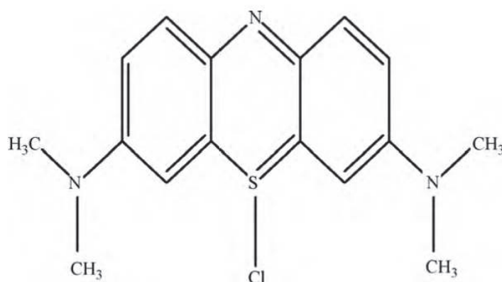
Fig. 1. Chemical structure of methylene blue molecule.
