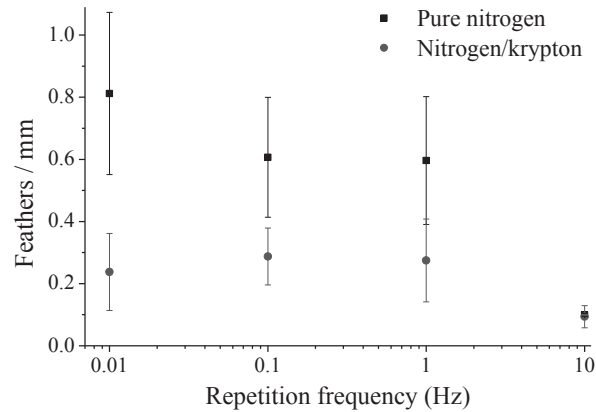
Figure 4. Feather density as function of repetition frequency in pure nitrogen and in the nitrogen/krypton mixture. Measurements are performed on discharges under the same conditions as shown in figure 3, but on channels extending further from the tip, outside the visible areas of figure 3 (to ensure a clean view of the channel). The measured values are the number of visible bumps, feathers, branches and all other irregularities per mm of streamer length and are not corrected for projection effects. The error bars give the standard deviation of the measurements.
