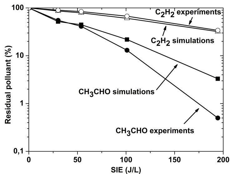
Fig. 4. Comparison between simulations and experiments for a mixture containing 500 ppmC of CH 3 CHO and 500 ppmC of C 2 H 2 .
