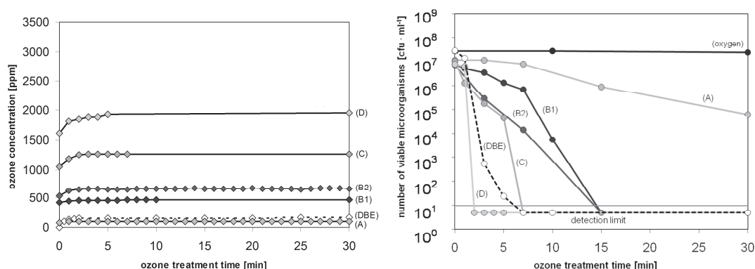
Fig. 4: left: \text{O}_3 concentrations in gas phase produced by ozoniser (A-D) and by surface DBD; right: Inactivation of E. coli suspensions by different \text{O}_3 concentrations compared to effect of DBD.
