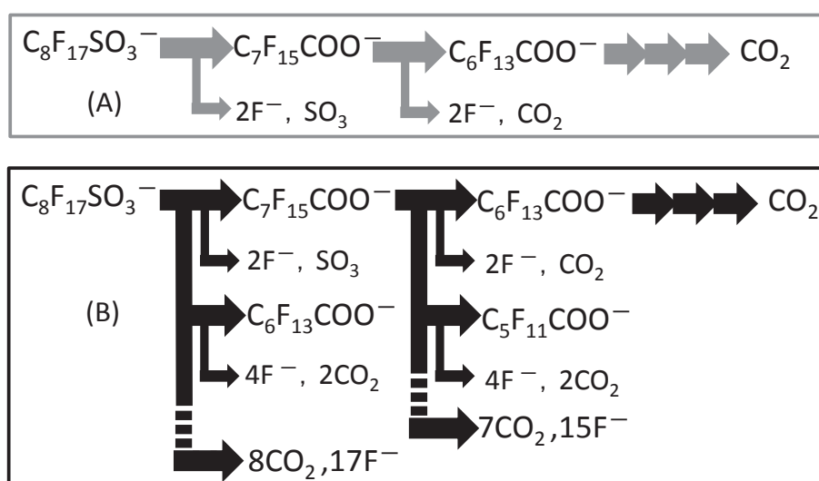
Fig. 8 Decomposition processes of PFOA: sequential decomposition (A) and simultaneous decomposition (B).
