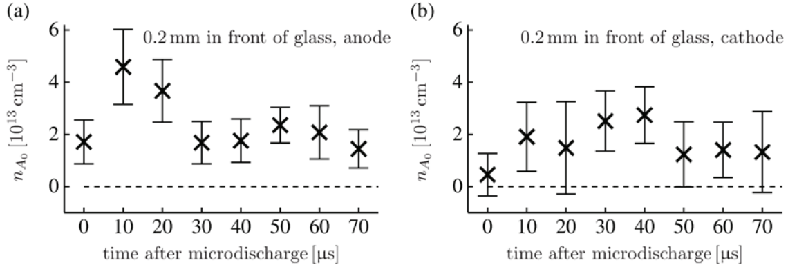
Fig. 3: Time dependence of the A^3\Sigma_u^+, v=0 density in the afterglow of a single microdischarge in front of the (a) anode and (b) cathode. 500 mbar, 2 kHz, 10.50 kV pp .
