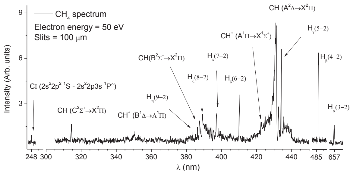
Fig. 1. Example of the measured spectrum. Some lines from Balmer's series as well as P, Q, and R branches of CH (A-X) and C (B-X) can be seen.
