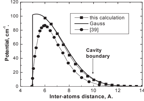
Fig. 3. Difference \Delta U(R) between potentials 3s^3S He* and 2p^3P He*(2p) calculated: Squares – this calculation. Circles – [39]. Line – fitting by Gauss curve Eq.(1).
