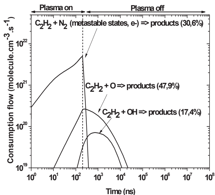
Fig. 6. Computed consumption flow of acetylene for an initial mixture containing 500 ppmC of acetaldehyde and 500 ppmC of acetylene in a 94.5% N 2 /5%O 2 gas flow
