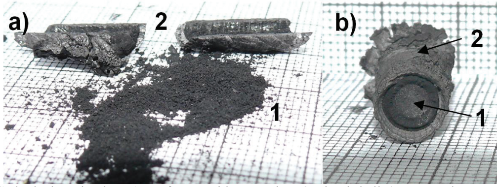
Fig. 1. Cathode deposit where 1 – soft core with nanotubes, 2 – hard shell a) separated parts of deposit b) deposit cross-section.
