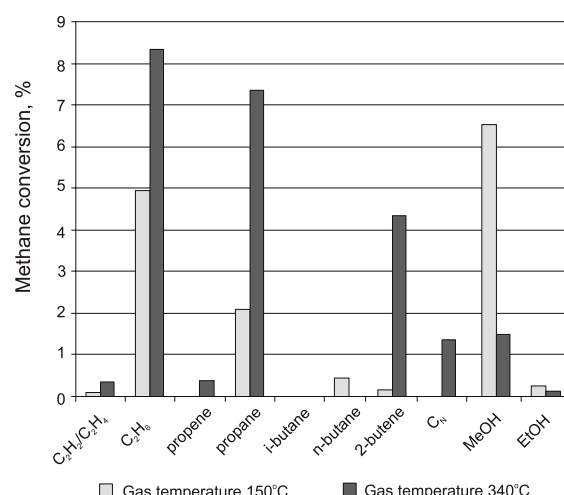
Fig. 4. Effect of temperature on methane conversion to hydrocarbons and alcohols. Power – 19 W, initial argon concentration 50%. Gas flow rate 2 NI/h.
