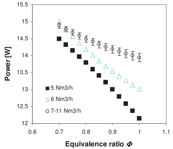
Fig. 4. TS power as a function of the equivalence ratio \Phi and gas flow rate Q .
