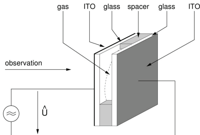
Fig. 1.: Schematic of the discharge cell. The glass plates with a thickness of 0.7mm are at a distance of 0.5 mm from each other. Both have been covered with an ITO layer, that acts as electrodes and allows the lateral observation in current flow direction.
