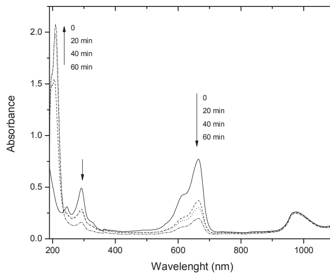
Fig. 5. Absorbance spectra of methylene blue solution after treatment in AC corona reactor. Reactor 1.
