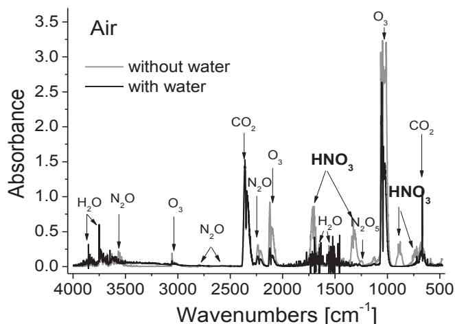
Fig. 4. FTIR spectra of air treated in water falling film reactor without water and with water
