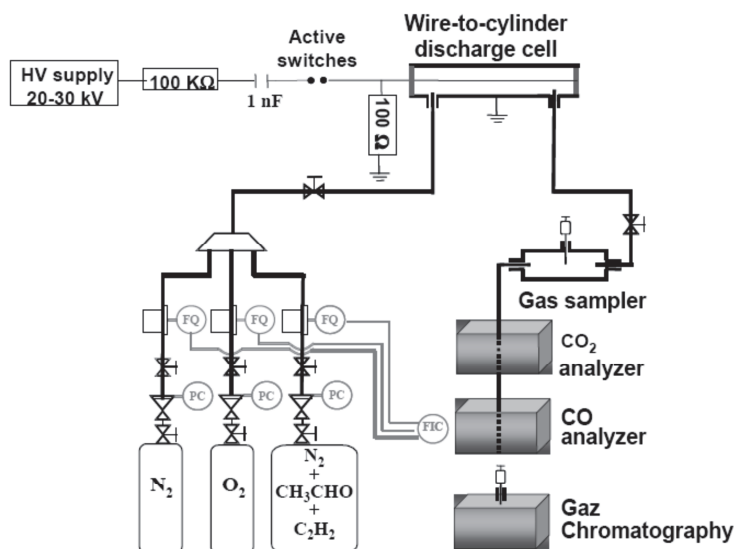
Fig. 1. Experimental set-up for investigation of mixture oxidation in WTC corona discharge.
