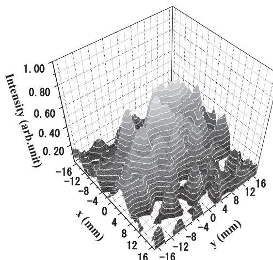
Fig. 6. Reconstructed distribution of the discharge sound in the x-y plane at 10 kHz.
