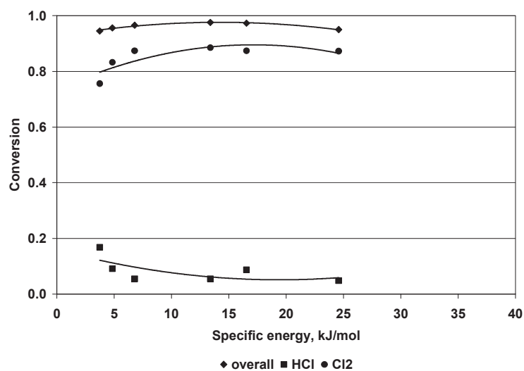
Fig. 5. The dependence between the \text{CHCl}_3 conversion and specific energy
