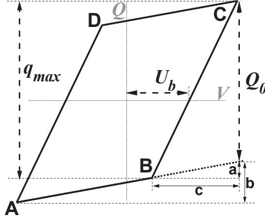
Figure 2. Schematic presentation of Q-V plot from classical electrical theory of ozonizers
