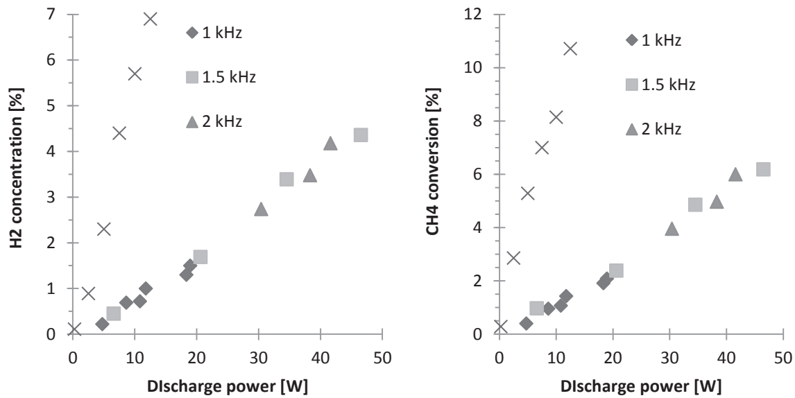
Fig. 5. Hydrogen concentration and methane conversion in CH 4 :CO 2 (70%:30%) gas mixture as a function of discharge power for different AC sine frequency and for nanosecond negative pulses.
