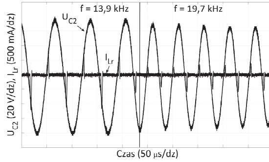
Fig. 5. The output voltage and current (primary high voltage transformer side) response to sudden resonant circuit parameter change.
