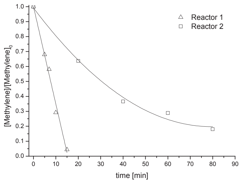
Fig. 4. Methylene blue decoloration efficiency in each reactor type. Reactor 1 – wire-to-mesh. Reactor 2 – wire-to-plate configuration.
