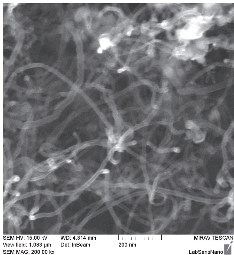
Fig.4. SEM image of deposited CNTs. The substrate temperature at deposition was 750°C.
