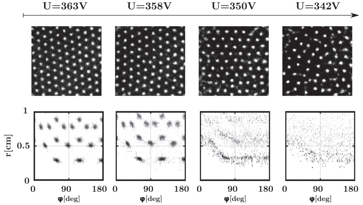
Fig.3.: Upper row: Light density distribution images at voltages close to the bifurcation point. Lower row: Triple correlation functions of the corresponding light density distribution. f = 80 kHz sinusoidal, Helium, without gas flow, exposure time 200 \mu s.
