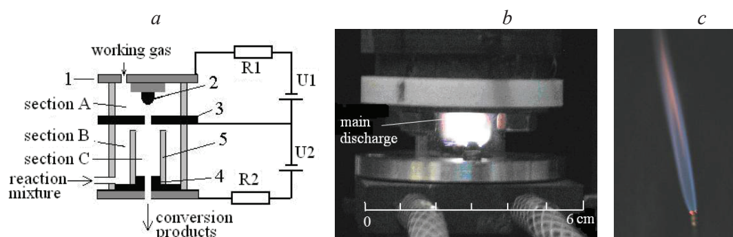
Fig. 1. Schematic of plasmachemical reactor (a) and photos of discharge during ethanol conversion (b) and flame at the reactor output (c).
