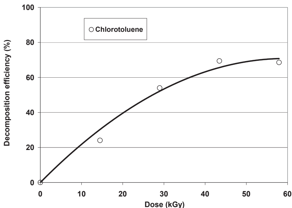
Fig. 1. A dependence of the removal efficiency of 4-chlorotoluene on the dose absorbed under EB radiation (initial concentration of 4-chlorotoluene was 51.9 ppm)
