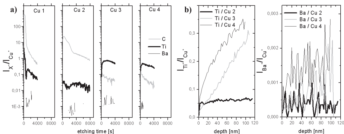
Fig. 1. The results of the SIMS profile analysis presented as ratio of ion current to the currents of the copper ion: a) versus the etching time (0-3 microns), b) versus the depth of etching (0-100 nm).
