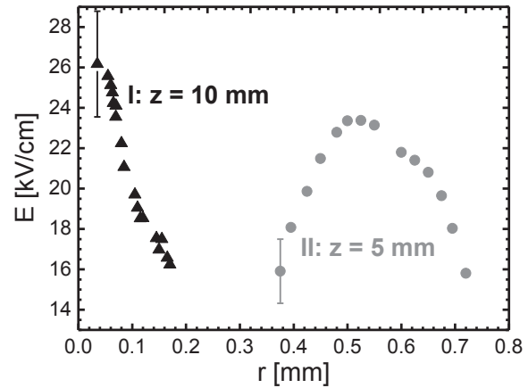
Fig. 7. Radial distribution of the axial electric field in the plasma jet at two characteristic axial positions.
