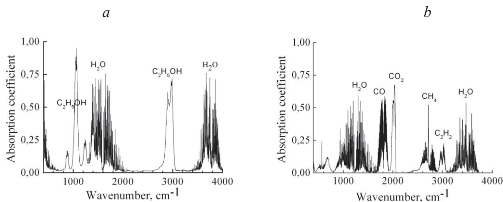
Fig. 3. Absorption IR-spectra of mixtures at the inlet (a) and outlet (b) of plasma reactor.
