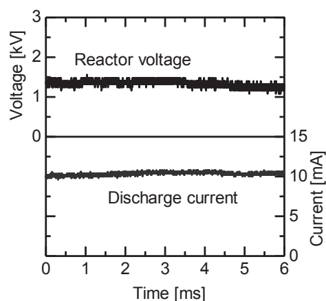
Fig. 2 Voltage and current waveforms.
