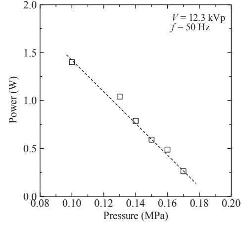
Fig. 6. Power dissipated in DBD device.
