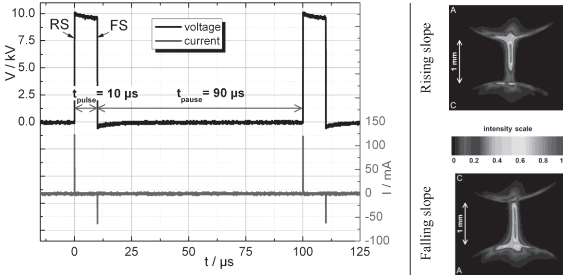
Fig. 2. Electrical characteristics of a pulsed DBD (left) and iCCD-photos (right; accumulation of 1,000 MDs; A= anode, C= cathode) at V_{\text{pulse}} = 10 kV with D = 10% at 0.1 vol% O 2 in N 2 .
