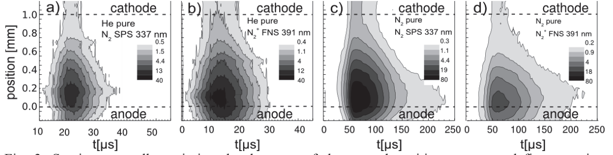
Fig. 3. Spatio-temporally emission development of the second positive system and first negative system in the diffuse helium and nitrogen BD.
