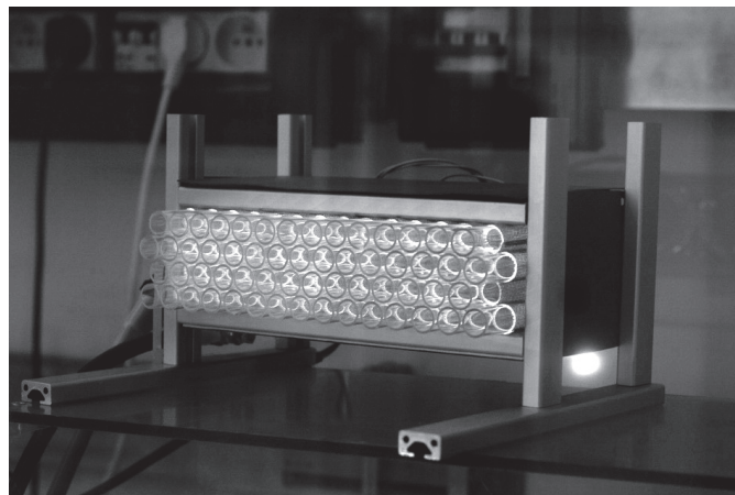
Fig. 1. The laboratory DBD reactor construction used for experiments.
