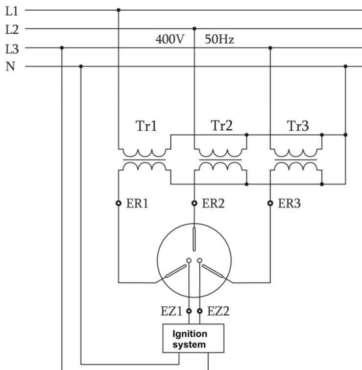
Fig. 3. Power system of GlidArc reactor
