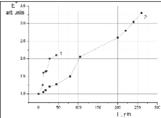
Fig.6. Maximum values of E^* as a function of the jut height for smooth (1) and rough (2) Piroceramics barriers
