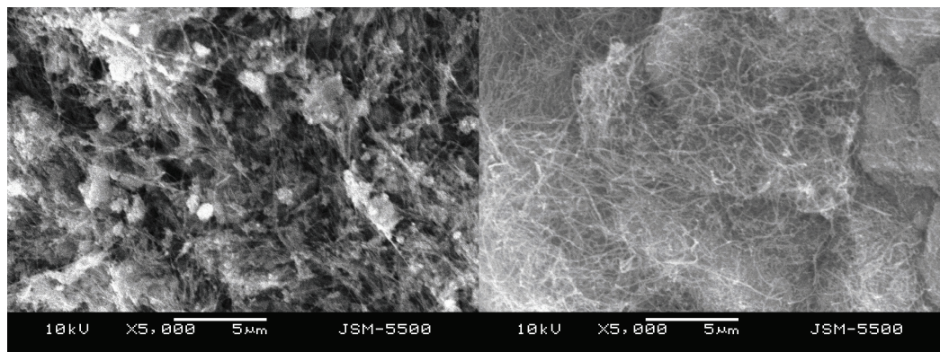
Fig. 6. - MWNTs nanotubes before pretreatment (left hand side) and after (right hand side)
