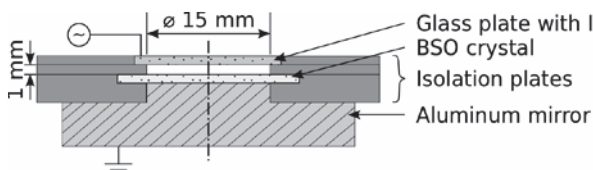
Fig. 1. Side-view of the discharge cell configuration.
