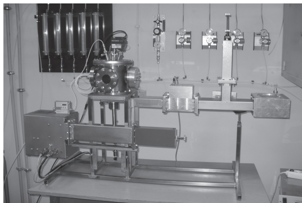
Fig. 1 Microwave plasma set up
