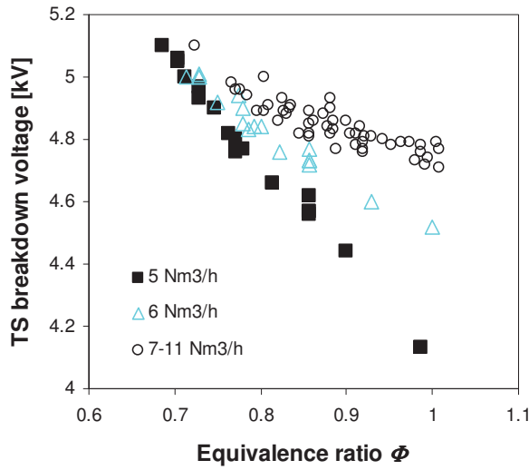
Fig. 3. TS breakdown voltage U_{TS} as a function of the equivalence ratio \Phi and gas flow rate Q .
