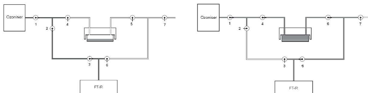
Fig. 2: Left: Adjustment of the ozoniser produced ozone, monitored by FT-IR (valves 1, 2, 3 open); Right: Gassing with adjusted O 3 concentration, monitored by FT-IR (valves 1, 4, 5 and 6 open).
