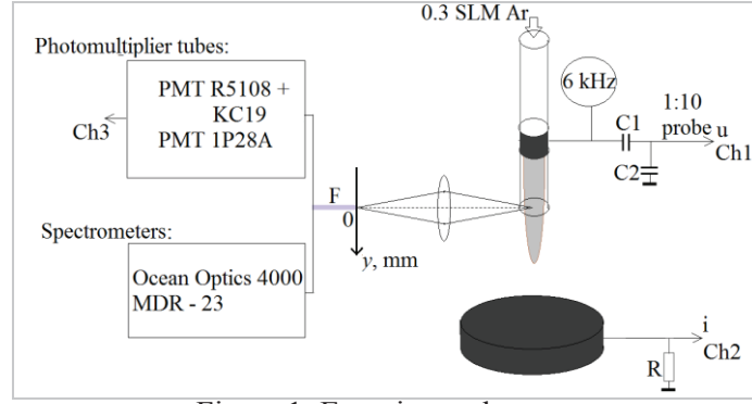
Figure 1. Experimental setup.
