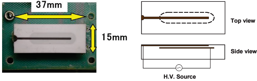
Fig. 4. Photo and schematic of the electrodes module.
