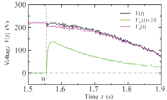
Fig. 9 Enlarged in the vicinity of B of Fig. 5(b) of voltage waveforms.
