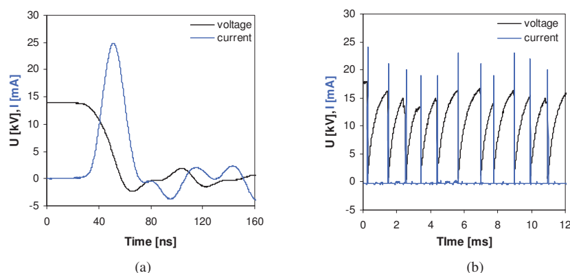
Fig. 3. Typical voltage and current waveforms of TS discharge with electro-spray of water in (a) ns time scale – one pulse, and (b) ms time scale – several pulses, 10 mm gap.
