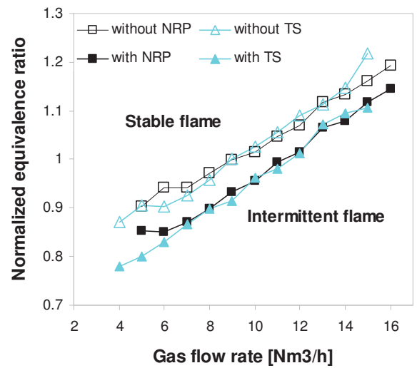
Fig. 7. Comparison of the stabilizing effect of NRP and TS discharges on lean \text{CH}_4 -air flame.
