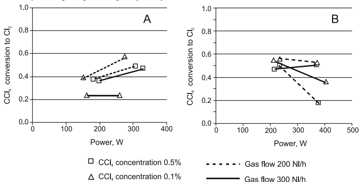
Fig. 4. Effect of gas flow rate and \text{CCl}_4 concentration on conversion of \text{CCl}_4 into \text{Cl}_2 . A – homogeneous system, B - plasma catalytic system with \text{V}_2\text{O}_5 /diatomite.
