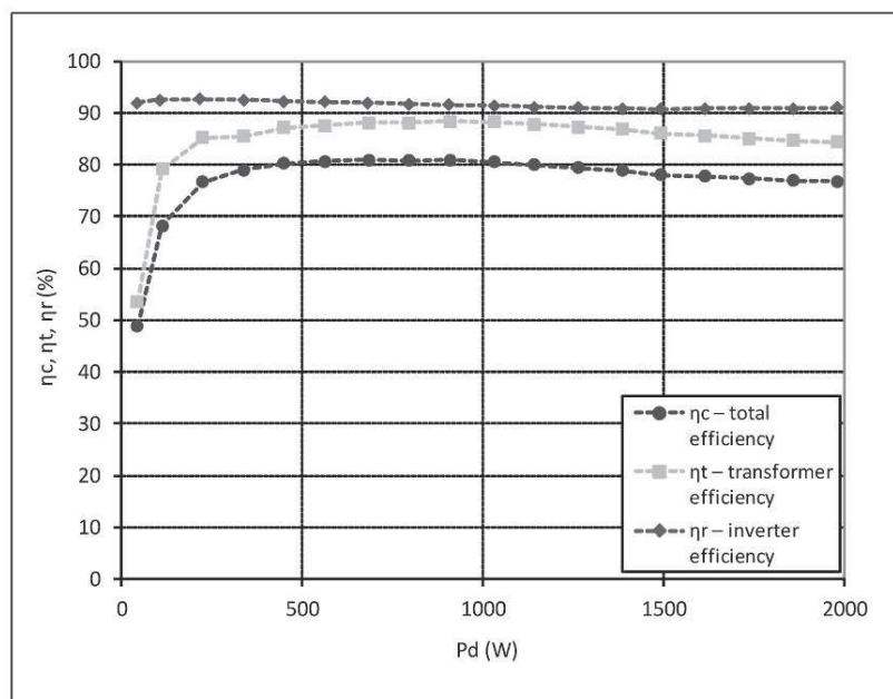
Fig. 9. Efficiency measurements of proposed power electronic supply construction and its main components.
