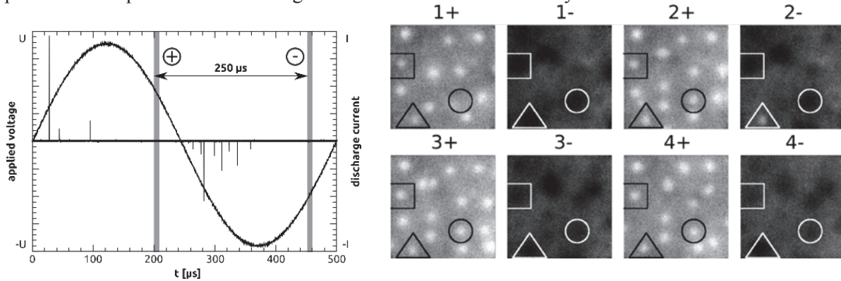
Fig. 6. Left: Timing of the surface charge measurement. At the end of each half period, when no discharge occurs, a record is made. The sign “+” or “-” given in the right image depicts the polarity of the voltage as indicated above. Right: Four consecutive periods. Surface charge measurement at fixed phase positions in the positive (200 \mu s) and negative 450 \mu s half period. Positive surface charges: bright spots, negative ones: dark spots. \square : long-living filament, \Delta : filament misses one or a few driving periods, and \circ : generating a filament in discharge free area.
