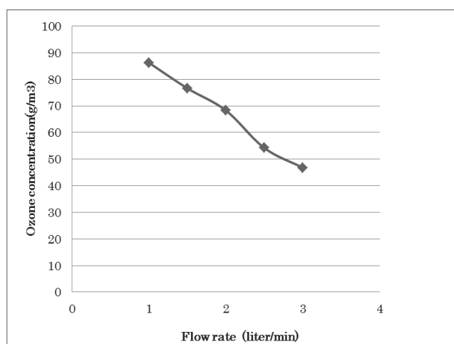
Fig.2 Ozone concentration characteristics of ozonizer.
