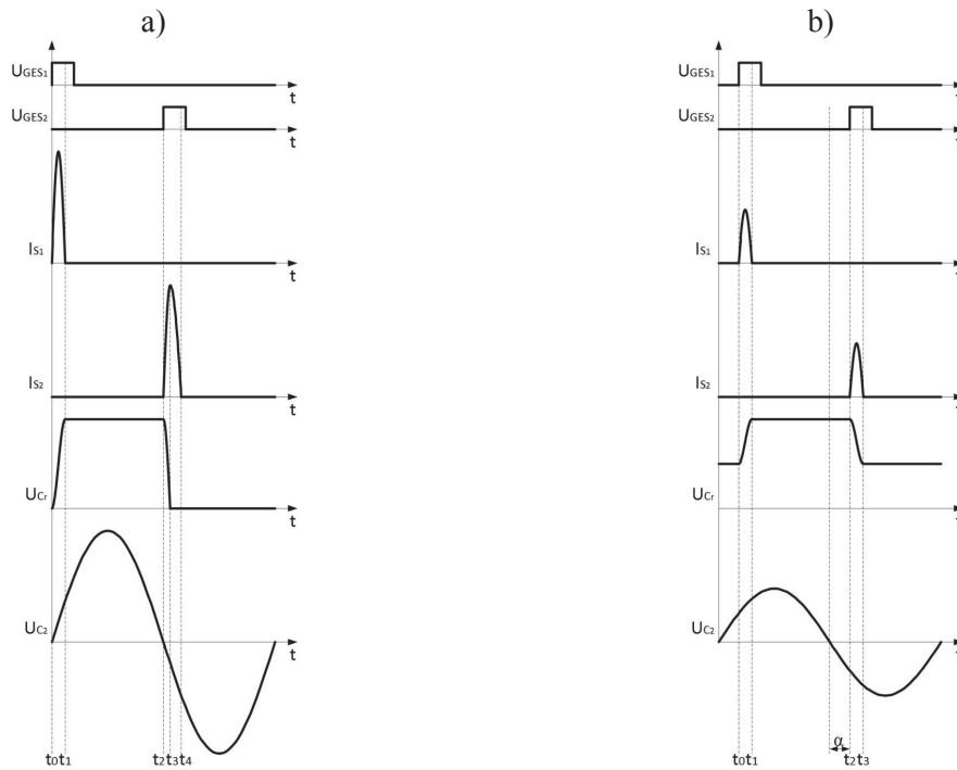
Fig. 4. Basic electrical waveforms during power supply system operation.
