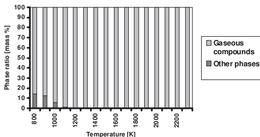
Fig.3. Phase ratio of methanol during its thermal decomposition
