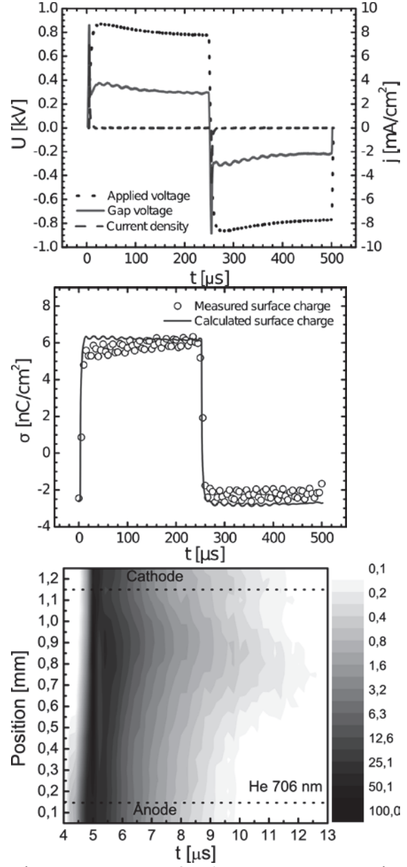
Fig. 5. Rectangle feeding voltage shape in a pure helium BD. Top: electrical characterization including applied voltage, gap voltage and net current. Centre: surface phase resolved charge measurement over one period. Bottom: emission development of helium at \lambda = 706 nm . Intensity maximum in front of the cathode. Voltage amplitude: 0.9 kV. pressure: 500 hPa, frequency: 2 kHz.
