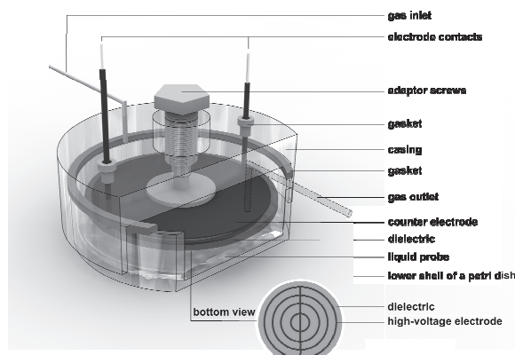
Fig. 1. Schematic drawing of the indirect surface DBD arrangement.
