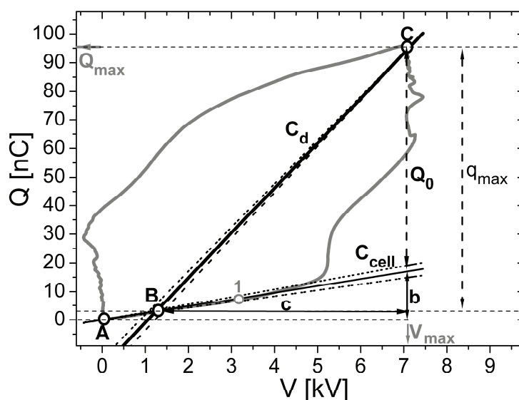
Figure 3. Q-V plot measured under pulsed excitation (data taken from in [7]).
