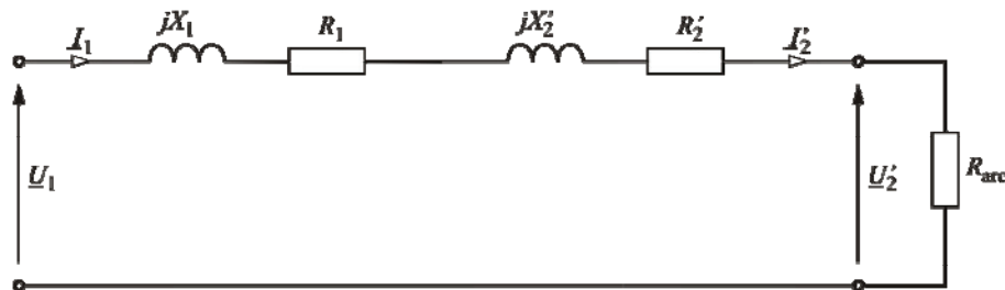
Fig. 1. Simplified equivalent scheme of loaded transformer.
