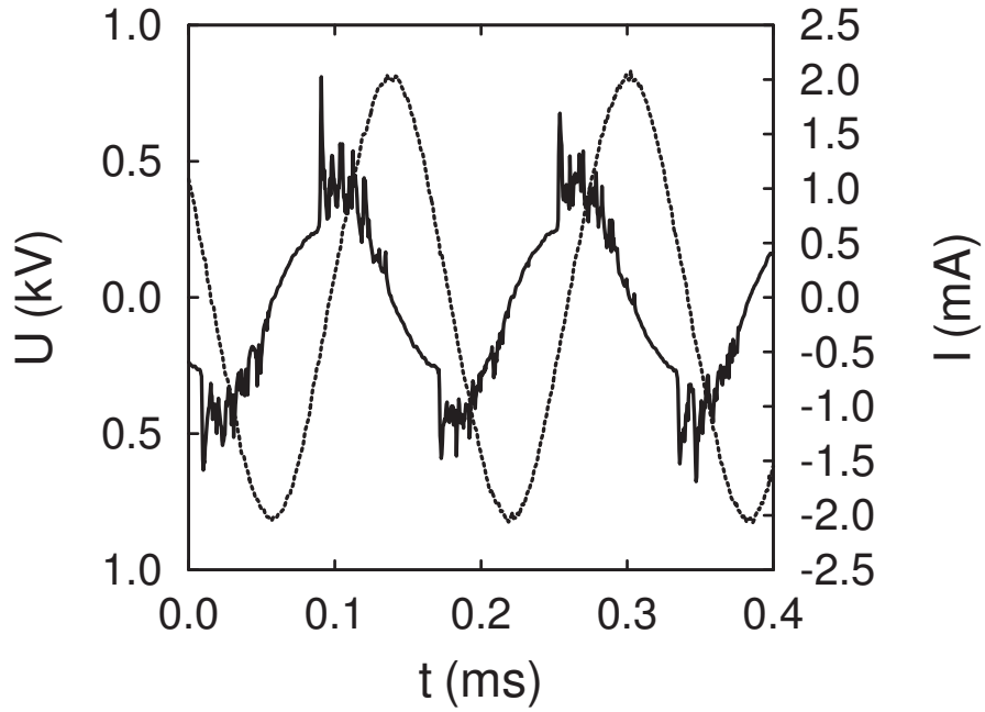
Fig. 2. The time dependence of applied voltage and discharge current in APGD in argon with 0.41% admixture of acetylene. Full line – discharge current, dotted line – applied voltage.
