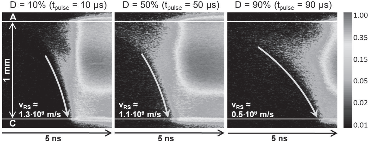
Fig. 4. Comparison of the change of the velocity of the cathode directed streamer at rising slope by changing the duty cycle D = 10\% ; 50\% ; 90\% (logarithmic intensity scale).
