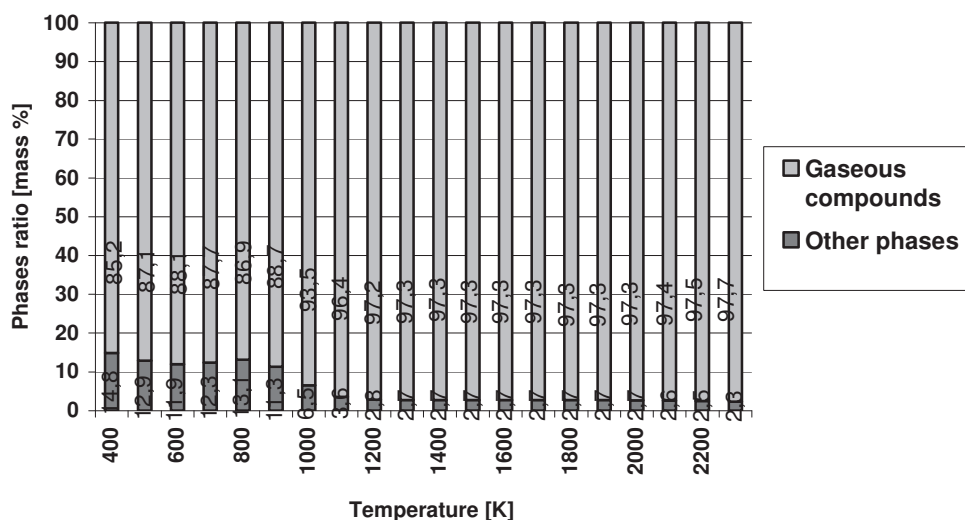
Fig.5 Phase ratio of methanol (66%) admixed with carbon tetrachloride (34%) during thermal decomposition
