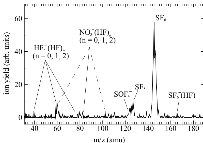
Fig. 2. Mass spectrum observed by TOFMS.
