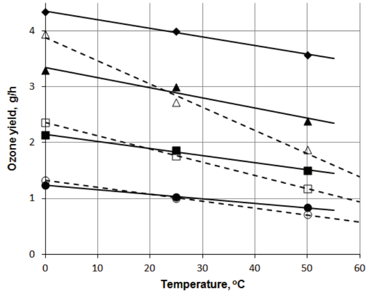
Fig. 3. Maximum ozone yields vs. temperature of cooling liquid; actuator (solid lines), metal mesh-dielectric system (dashed lines); oxygen flow-rates: ○, ● – 10 Ndm 3 /h, □, ■ – 20 Ndm 3 /h, △, ▲ – 40 Ndm 3 /h, ◆ – 80 Ndm 3 /h.
