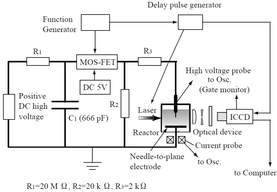
Fig. 1. Electrical circuit for generating pulsed high-voltage.
