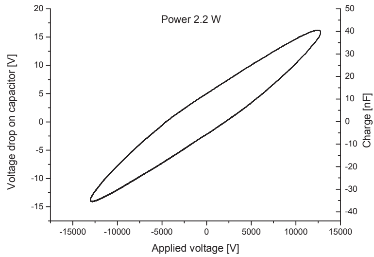
Fig. 3. Standard Lissajous curve for discharge power measurement.
