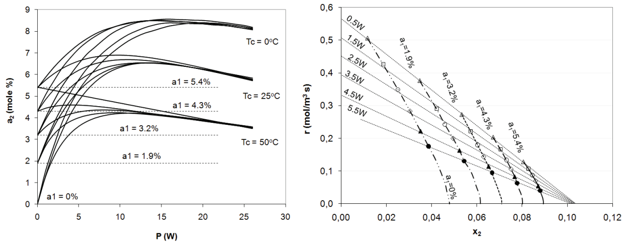
Fig. 2. Outlet ozone content a_2 vs. initial ozone content a_1 and active power; temperature of cooling liquid T_c = 0, 25 and 50^\circ\text{C} (left); Ozone synthesis process rate vs. conversion degree and low powers (right); temperature of cooling liquid T_c = 25^\circ\text{C} ; initial ozone content a_1 = 0, 1.9, 3.2, 4.3 and 5.4\% .
