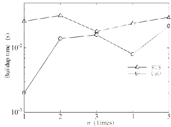
Fig. 12 Variation of rise time by repeated measurement.
