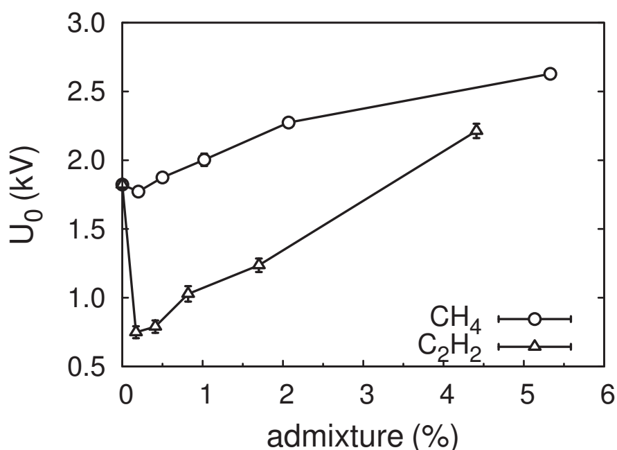
Fig. 1. The dependence of ignition voltage U_0 on admixture concentrations.
