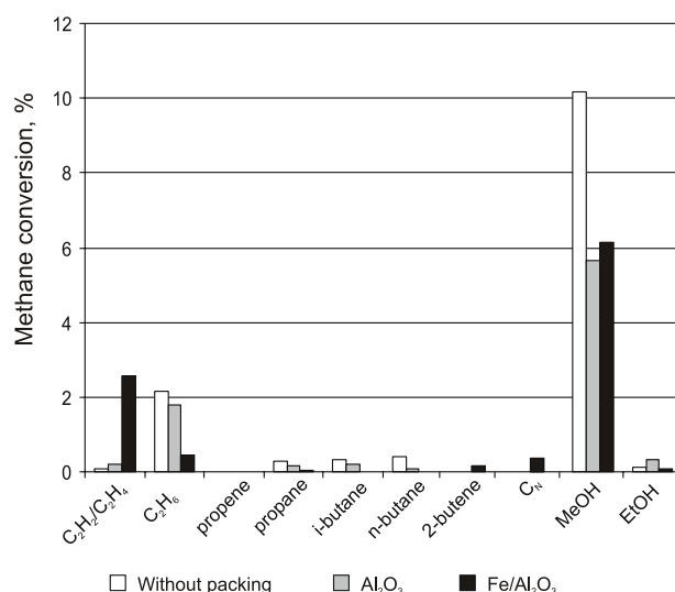
Fig. 10. Effect of the packing of discharge gap on methane conversion to hydrocarbons and methanol and ethanol. Molar ratio [CH 4 ]: [O 2 ]=3:1, Power – 15 W. Argon conc. 25%. Gas flow rate 2 NI/h.
