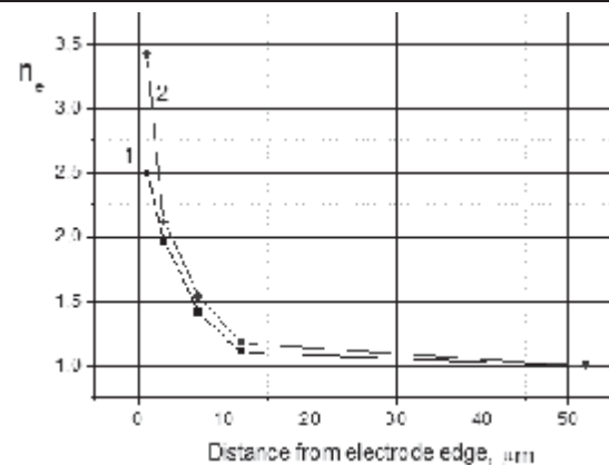
Fig.8. Number of electrons created near one jut at different distances from electrode edge. 1-Alumina without cover, 2-with a layer of Al_2O_3
