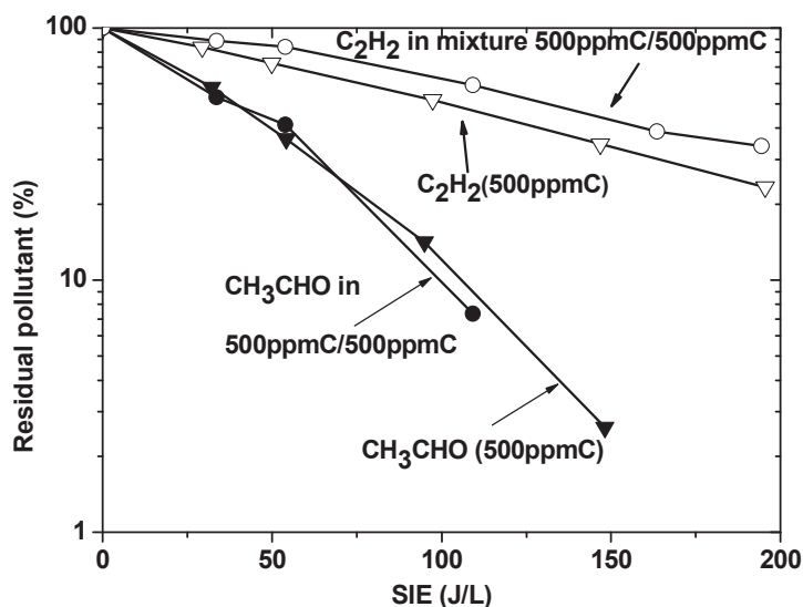
Fig. 2. Comparison of degradation of 500 ppmC of acetaldehyde and 500 ppmC of acetylene alone and in mixture in a 94.5% N_2/5\%O_2 gas flow.
