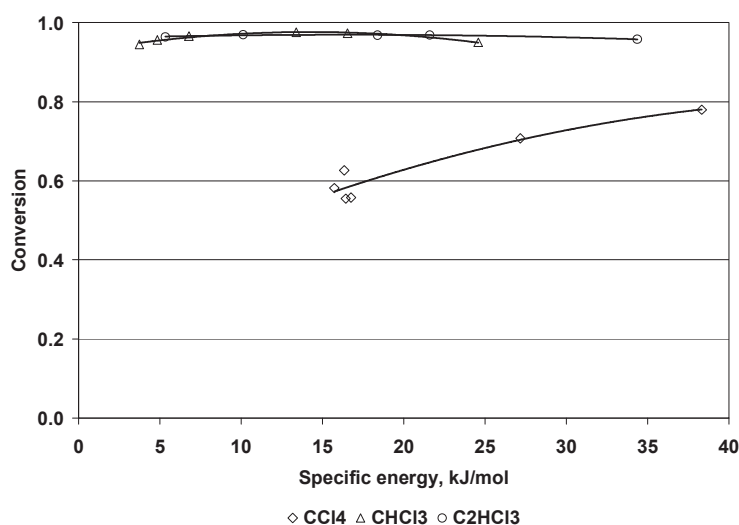
Fig. 3. The dependence between type of VOCs and overall VOCs conversion
