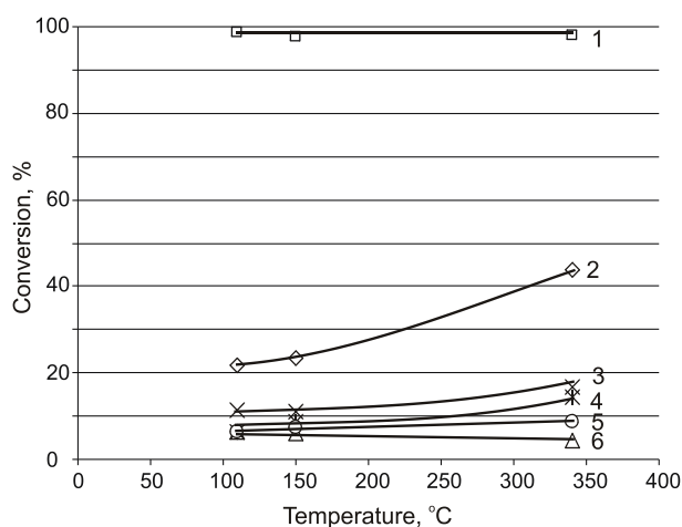
Fig. 7. Effect of temperature on overall conversion of methane (2) and oxygen (1) and conversion of methane to CO (3), H 2 (4), H 2 O (5) and CO 2 (6). Molar ratio [CH 4 ]: [O 2 ]=3, Power – 15 W, argon conc. 25%. Gas flow rate 2 NI/h.
