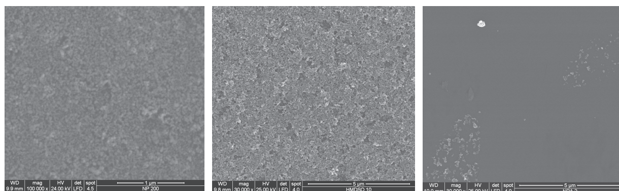
Fig. 1. SEM images of: (a) dip coated NP200 sample, (b) two-steps composite coating obtained with HMDSO, (c) NP_A sample: one-step composite coating.
