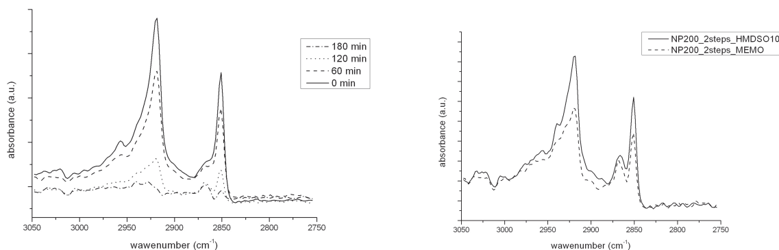
Fig.6. FTIR spectra of C–H bonds in stearic acid: NP200_2steps_MEMO6 on the left (a), and the comparison between NP200_2steps_HMDSO10 and NP200_2steps_MEMO6 at 120 minutes of UV-light (b).
