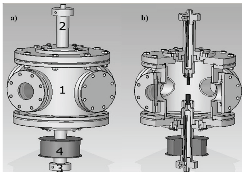
Fig.2. Reaction chamber (left hand side – a) and view inside the chamber (right hand side – b) (1 – chamber, 2 – anode, 3 – cathode, 4 – magnetic coil).
