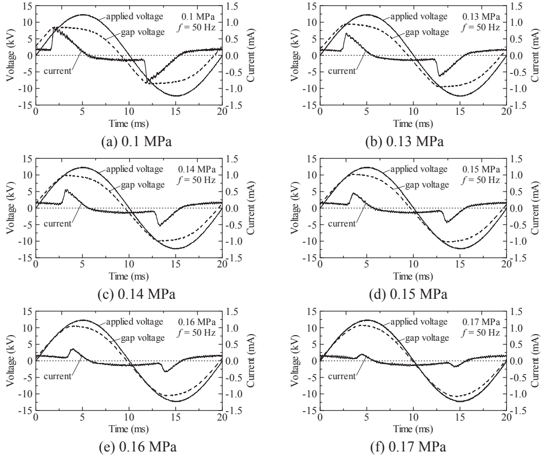
Fig. 3. Applied voltage, gap voltage and current waveforms.
