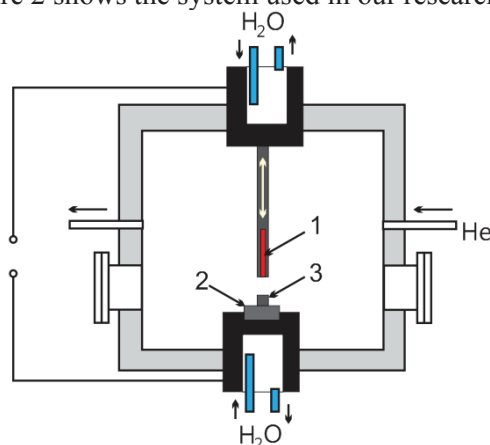
Fig.2. System for arc carbon nanotubes synthesis – 1 – anode with catalyst, 2- cathode, 3 – deposit
