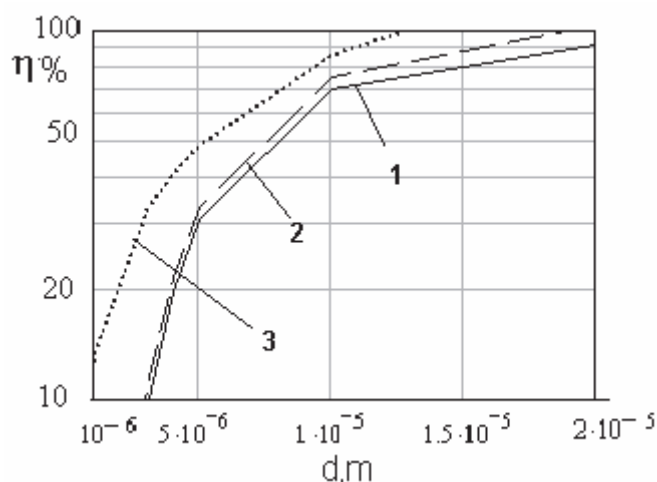
Figure 2 Dependence of air cleaning degree from dust ( \eta ) at the size of dust ( d ) for different charged combinations of the water drops ( D = 5\text{mm} ) and dust
