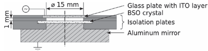
Fig. 1. Side-view of the discharge cell configuration.
