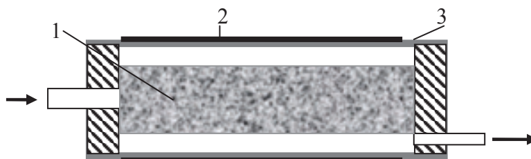
Fig. 1. Schema of reactor. 1 – high-voltage electrode, 2 – grounded electrode, 3 – dielectric barrier.
