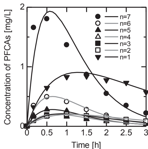
Fig. 7 Measured and calculated concentrations of PFCAs as a function of operating time.
