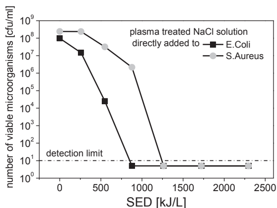
Fig. 6. Inactivation of E. coli and S. aureus in indirect plasma treatment as a function of SED
