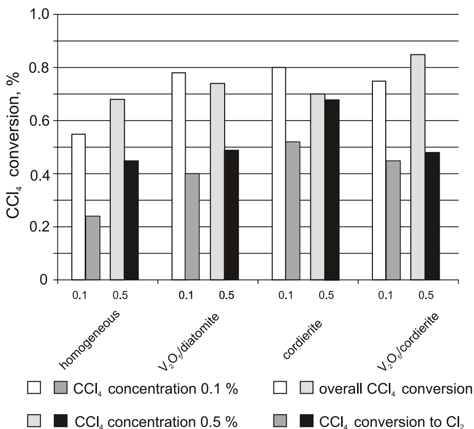
Fig. 5. Effect of catalysts on \text{CCl}_4 decomposition. Gas flow 300 Nl/h, discharge power 300W.
