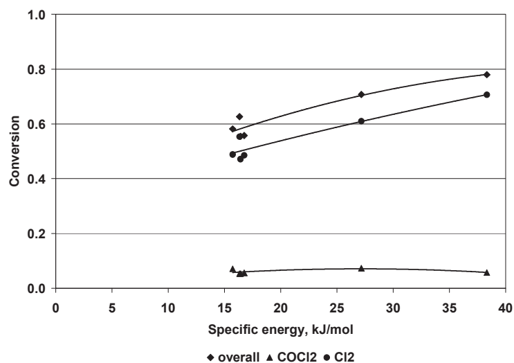
Fig. 4. The dependence between the \text{CCl}_4 conversion and specific energy
