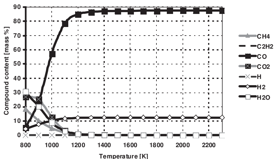
Fig. 4 Thermal decomposition of methanol gaseous fraction
