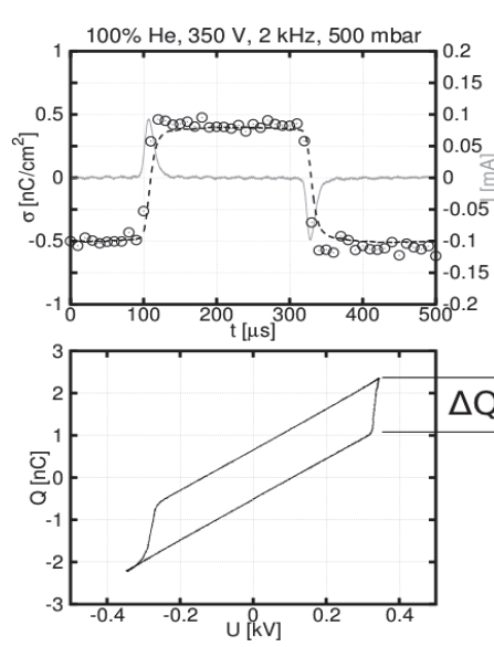
Fig. 4. Phase resolved surface charge from the electro-optic measurement (circles) with the corresponding net current (solid line) and the temporally integration of the net current (dashed line).
