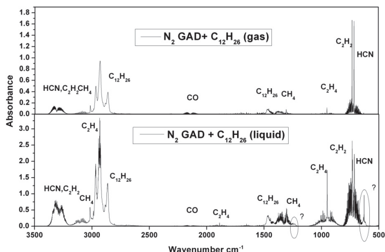
Fig 4. Comparison between the FTIR absorption spectra of the gaseous products after nitrogen gliding arc plasma treatment of dodecane in vapour and liquid phase in maximum achievable input power, P=185\text{W} and P=200\text{W} respectively. The spectra resolution is 1\text{ cm}^{-1} .
