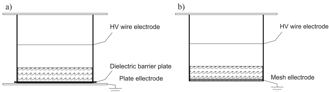
Fig. 2. Reactor schematics - a) reactor 1 – wire-to-plate configuration, b) reactor 2 – wire-to-mesh configuration.
