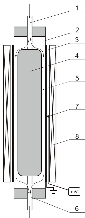
Fig. 1. Reactor for methane conversion. 1 – gas inlet, 2 – quartz tube, 3 – grounded electrode, 4 – high voltage electrode, 5 – discharge gap, 6 – gas outlet, 7 – thermocouple, 8 – heater.
