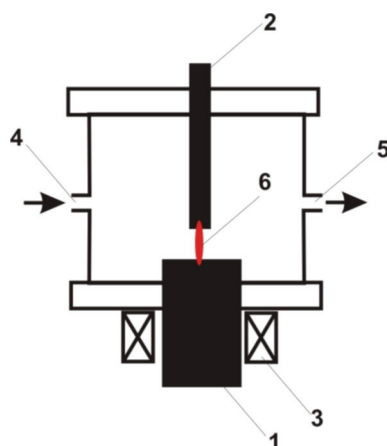
Fig. 1. Concept of reactor (1 – cathode, 2 – anode, 3 – magnetic coil, 4 - gas inlet, 5 – gas outlet, 6- electric arc)
