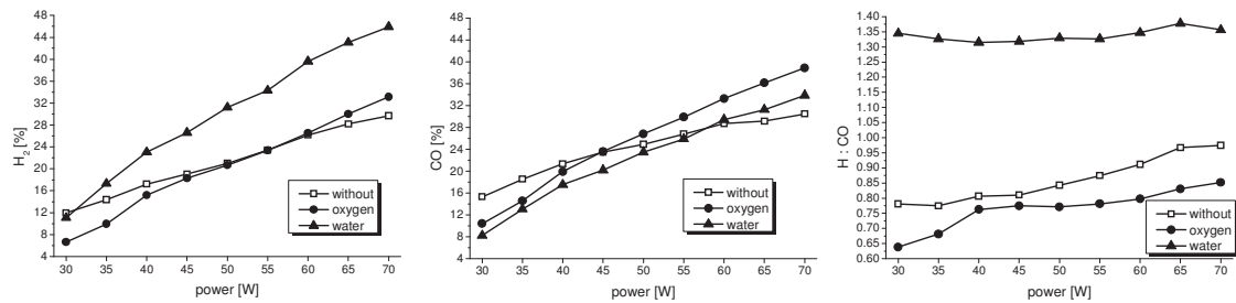
Fig. 2. Hydrogen (left) and carbon monoxide (middle) yield and its ratio (right) as a function of the power and different additives.
