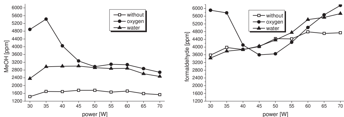
Fig. 3. Concentration of methanol (left) and formaldehyde (right) as a function of the power and different additives.
