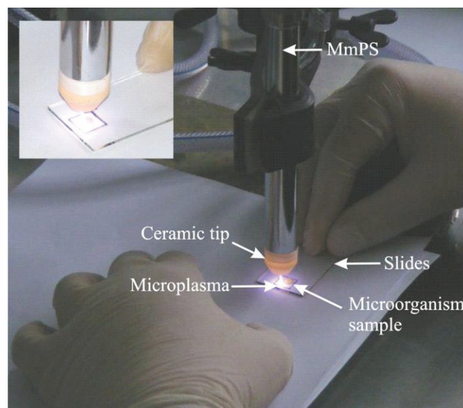
Fig. 2. Microwave microplasma sample treatment
