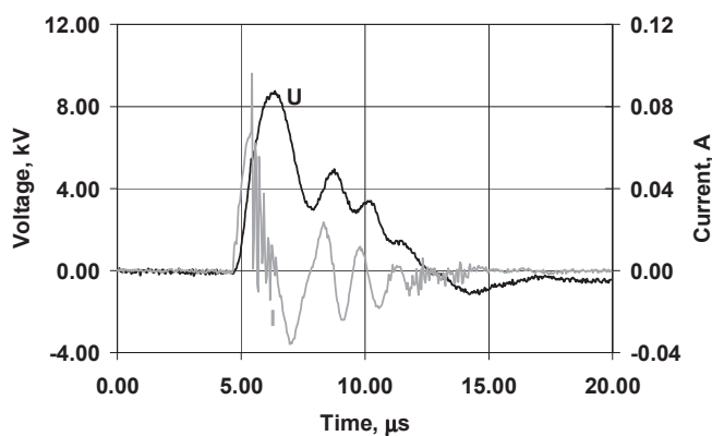
Fig. 3. Traces of pulses voltage and current for pulsed of low frequency (<1 kHz) power supply system.
