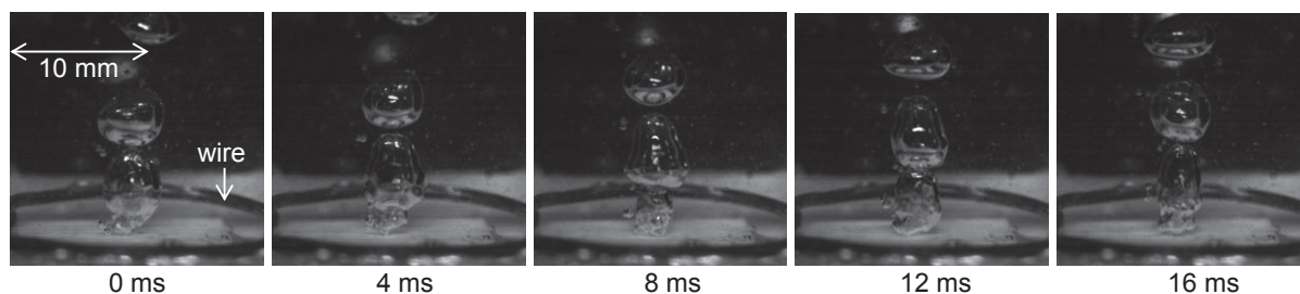
Fig. 3 Time-varying oxygen bubbles at a flow rate of 100 sccm into a 50 mg/L PFOS.
