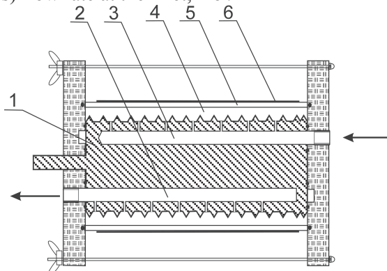
Fig. 1. Schema of reactor. 1 – high-voltage electrode, 2, 3 – internal channels, 4 – discharge zone, 5 – dielectric barrier, 6 – grounded electrode.
