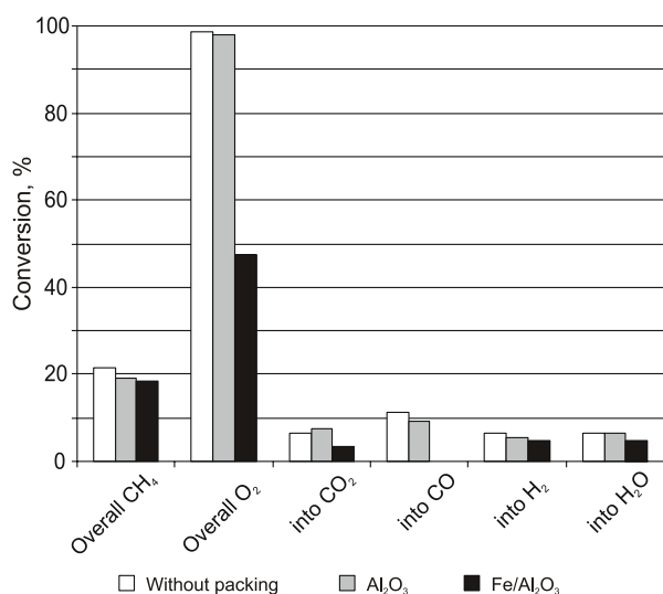
Fig. 9. Effect of the packing of discharge gap on overall conversion of methane and oxygen and conversion of methane to H 2 , CO, CO 2 , and H 2 O. Power – 15 W. Argon conc. 25%. Gas flow rate 2 NI/h.
