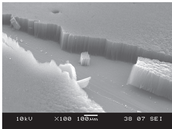
Fig. 2 SEM photo of MWNTs forest
