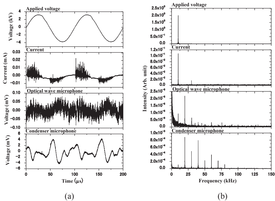
Fig. 5. Voltage waveforms (a) and FFT results (b) obtained from high voltage probe, shunt resistance, OWM and condenser microphone. The frequency of applied voltage is 10 kHz.
