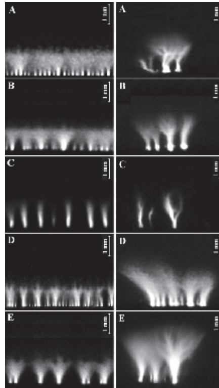
Fig. 1. Images of discharge across barriers with films of Alumina (left) and rough Pyroceramics (right). A - without a film, B – BST film, C – TiO 2 film, D – Al 2 O 3 film, E – SiO 2 film.
