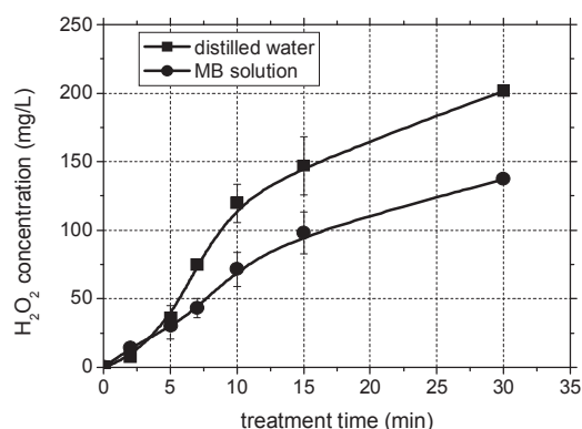
Fig. 3. Concentration of \text{H}_2\text{O}_2 generated in water and in the MB solution as a function of plasma treatment time.
