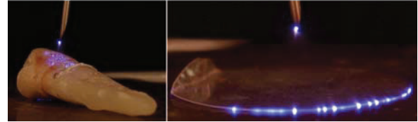
Fig. 3. The oscilloscopic record of the current of negative Trichel pulses ( U = 6.88 kV, f = 550 kHz, I_{\max} = 0.17 mA) and the related photos on teeth and plastic surfaces
