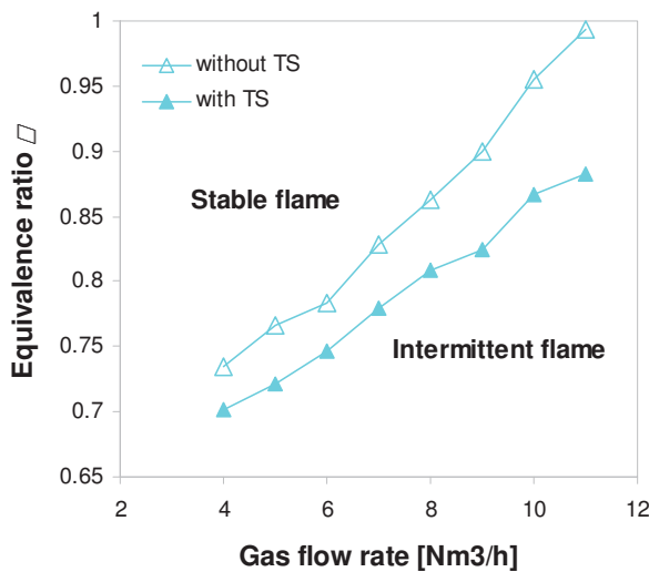
Fig. 6. Stabilizing effect of TS discharge on lean \text{CH}_4 -air flame.
