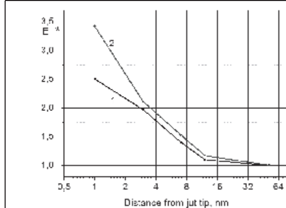
Fig.7. Influence of a Al_2O_3 layer on the field distribution near the gut tip. 1- Alumina without a cover, 2 - with a layer of Al_2O_3
