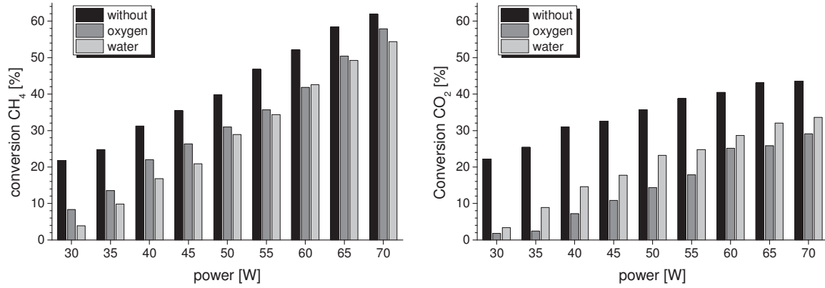
Fig. 1. Conversion of methane (left) and carbon dioxide (right) as a function of power and different additives.
