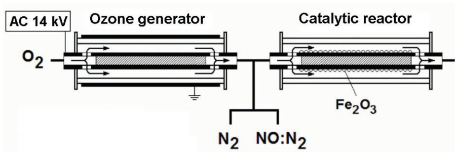
Fig. 1. Sketch of the ozone injection reactor.
