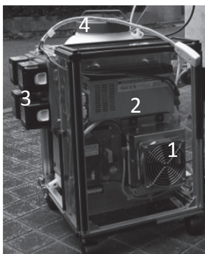
Fig.1 Ozone-mist sterilization system
