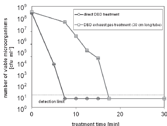
Fig. 6: Inactivation kinetics of E. coli by direct DBD treatment (-o-) and by DBD exhaust gas treatment (-□-) in air.
