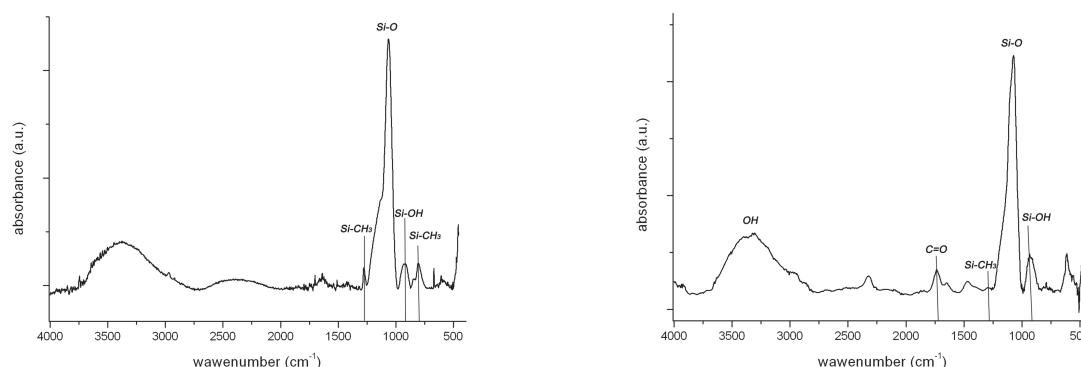
Fig. 3. Typical FT-IR spectra of HMDSO coating on the left (a) and MEMO coating on the right (b).
