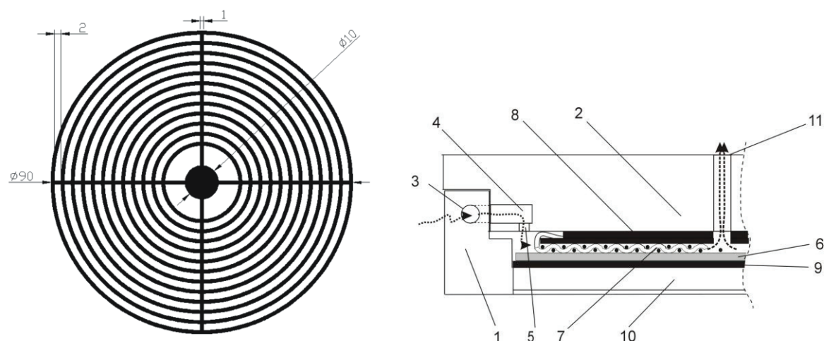
Fig. 2. Discharge elements: a) concentric strip electrode on the actuator surface, b) scheme of reaction space operating with mesh-ceramic plate system. The arrows depicts a way of the gas flow; 1 – main body of the reactor, 2 – reactor lid, 3 – gas inlet channels, 4 – collecting ring, 5 – openings through which the gas enters the reaction space, 6 – ceramic plate, 7 – mesh, 8 – metal plate, 9 – wall of the cooling chamber, 10 – cooling chamber, 11 – outlet of the post-reaction gas.
