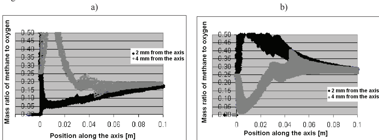
Fig.3 The variation of mass ratio of methane to oxygen along the axis of the reactor calculated numerically in the distance from the axis of reactor of 2 mm and 4 mm. The methane was introduced into the reactor applying: a- the second method, b – the first method (methane oxidation was not considered).
