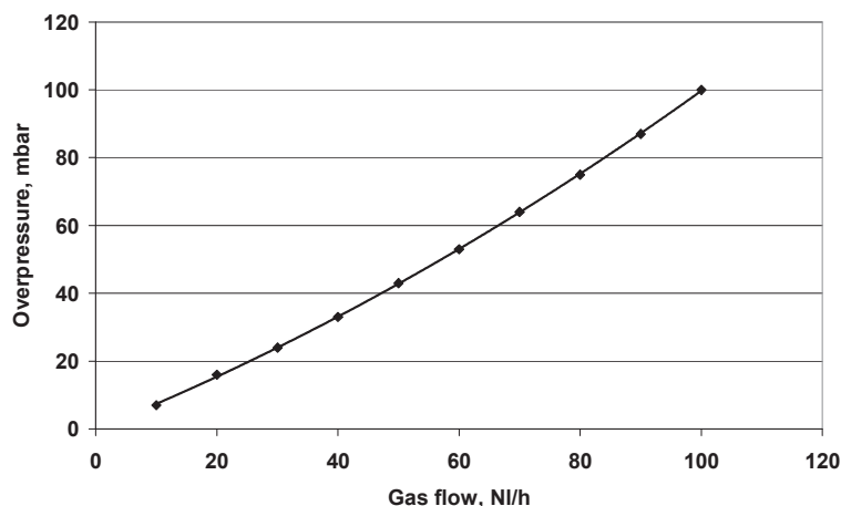
Fig. 2. Influence of gas flow on the gas pressure
