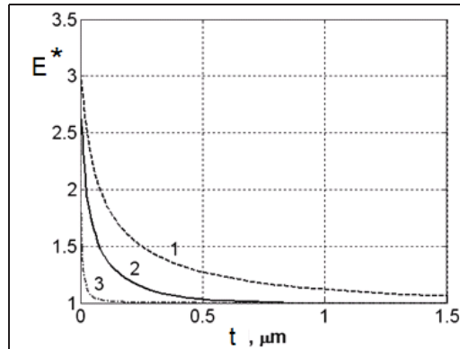
Fig.5. Field distribution neat a single jut as a function of the distance from the jut tip. 1- rough Pyroceramics, 2 – Alumina, 3 – smooth Pyroceramics
