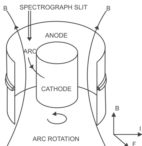
Fig.3 ROTARC plasma reactor principle
