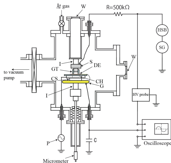
Fig. 1 Schematic diagram of experimental setup. SG: Signal generator, HSB: High-speed bipolar power supply, S: Stainless steel electrode, DE: Dielectric electrode, CH: Ceramic heater, CS: Ceramic spacer, G: Gold film electrode, I: Insulator, W: Quartz window, GT: Glass tube, P: Power supply for ceramic heater.
