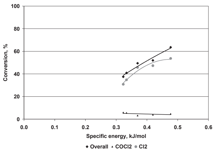
Fig. 6. The dependence between the \text{CCl}_4 conversion and specific energy for pulsed of low frequency (<1 kHz) power supply system.
