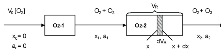
Fig 1. Idea of determining the differential reaction rate of ozone synthesis.
