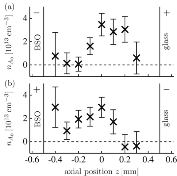
Fig. 6: Axial A^3\Sigma_u^+, v=0 density profiles for the (a) positive and (b) negative half cycle in the diffuse mode at 500 mbar, 2 kHz, 8.00 kV pp , and 125 μs after zero-crossing of the voltage.
