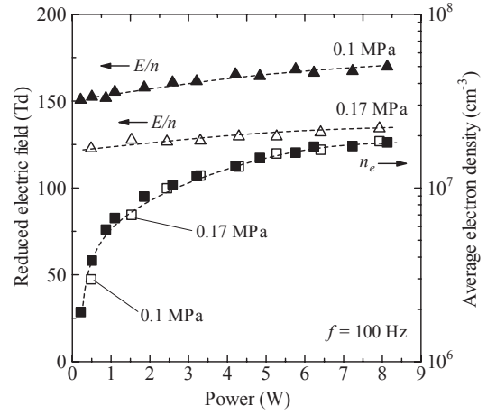
Fig. 8. E/n vs. n_e (effect of power).
