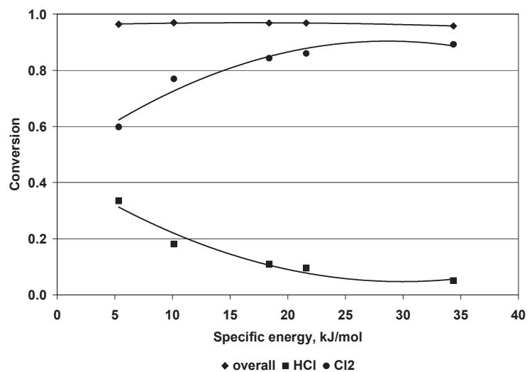
Fig. 6. The dependence between the \text{C}_2\text{HCl}_3 conversion and specific energy
