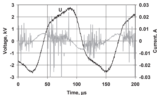
Fig. 2. Traces of pulses voltage and current for AC power supply system.
