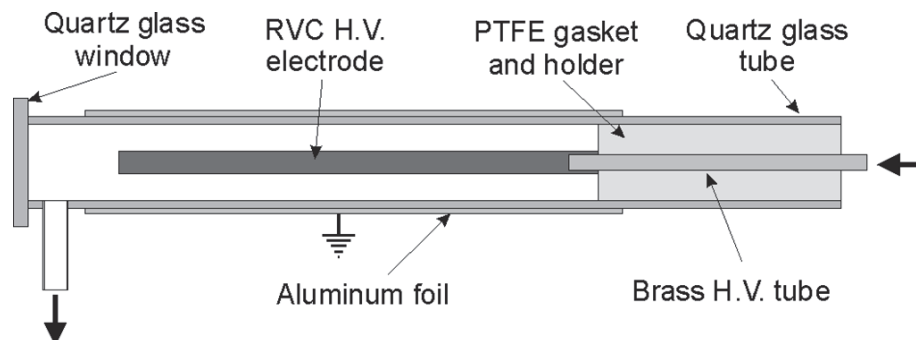
Fig. 1. DBD reactor with RVC electrode.
