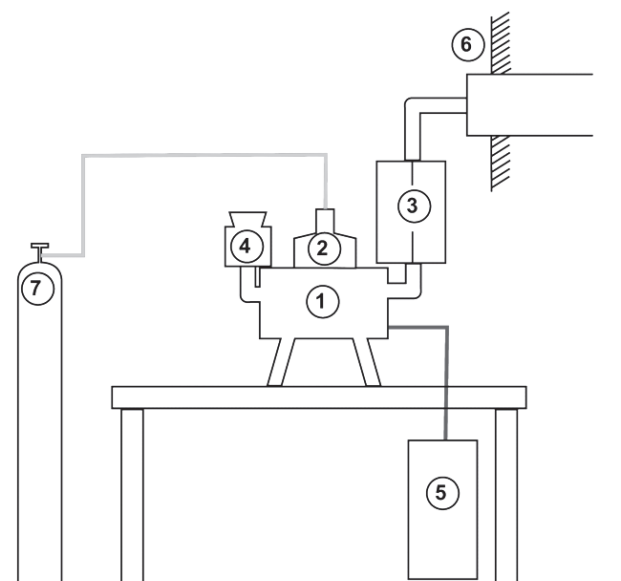
Fig. 1. PDUCR installation (parts numbered described in the text)
