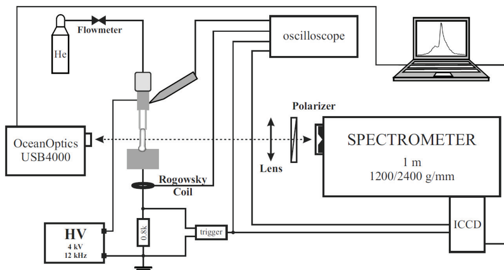
Fig. 1. Experimental set-up.
