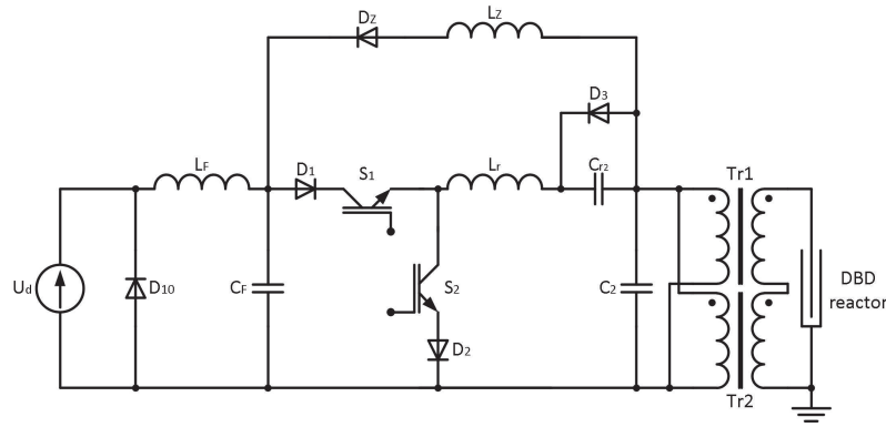
Fig. 3. The topology of power electronic, resonant supply suitable for continuous resonant frequency tracking.
