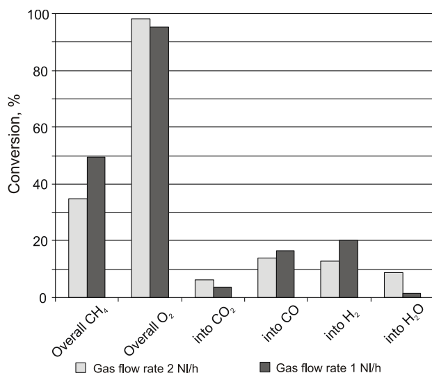
Fig. 5. Effect of the gas flow rate on overall conversion of methane and oxygen and conversion of methane to H 2 , CO, CO 2 , and H 2 O. Power – 19 W, argon conc. 50%.
