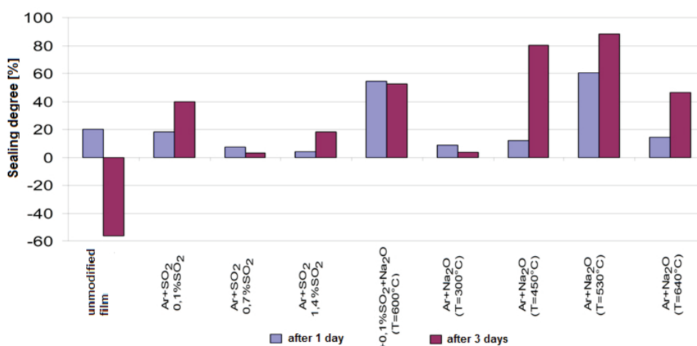
Fig. 6. Dependence of the sealing degree of the film towards water vapor on the type of modification; modification time of particular films = 6 min.
