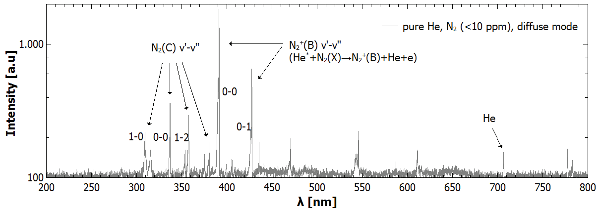
Fig. 3. Overview spectrum in pure helium, sinusoidal feeding voltage signal.
