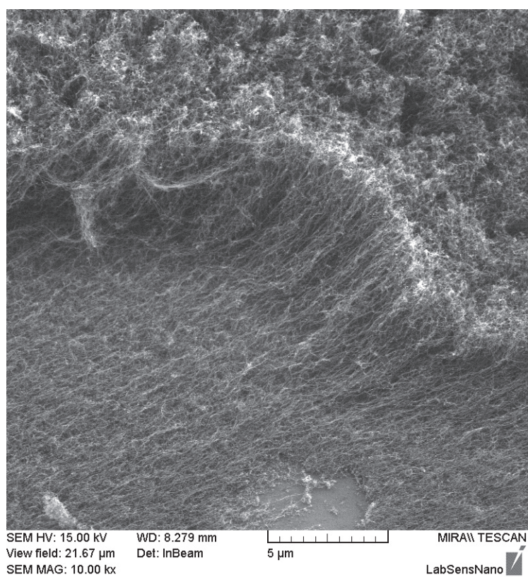
Fig 5. SEM image of deposited CNTs. Side view from the scratch in the CNTs layer.
