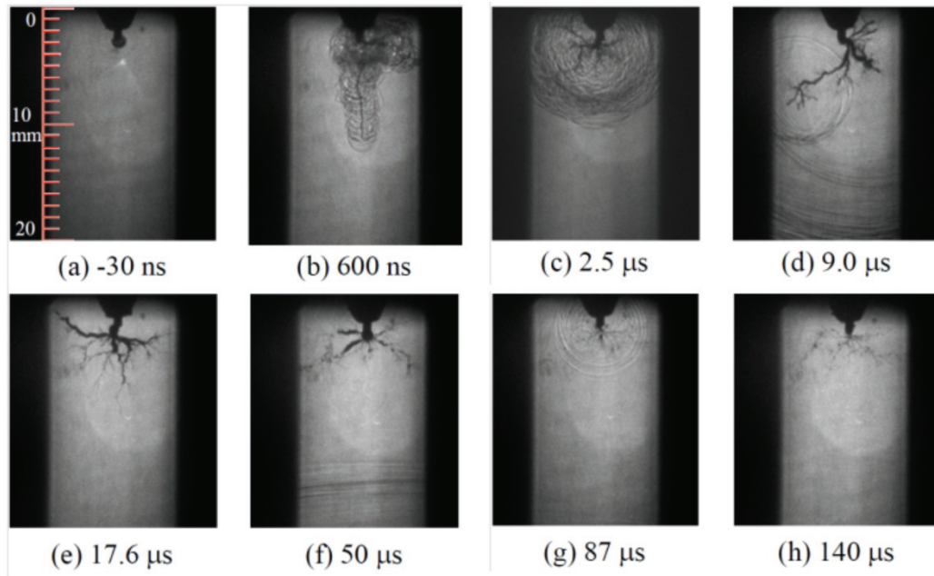
Fig. 4. Time evolution of Schlieren images. (applied voltage: 23 kV, pulse duration: 10 \mu s, discharge current: 4-6 A, needle-to-plane electrode, gap: 40 mm, distilled water).
