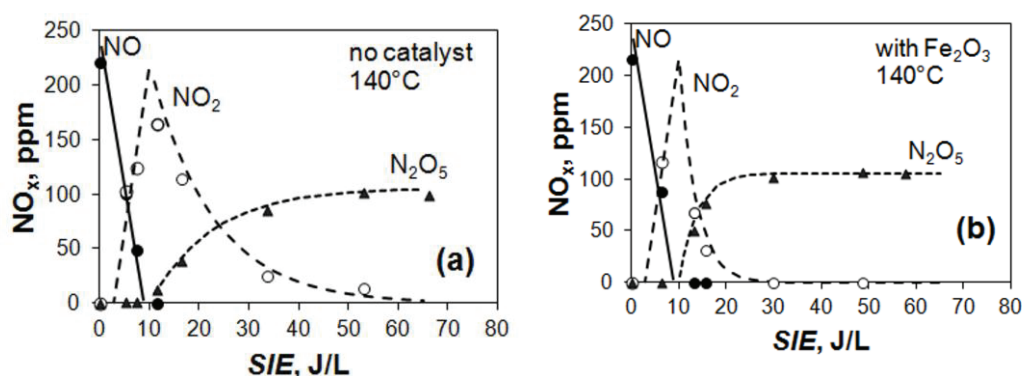
Fig. 4. The oxidation of NO to NO_2 and N_2O_5 in ozone injection reactor at 140^\circ C (a) without catalyst and (b) with Fe_2O_3 . Circles and triangles mark experimental points.
