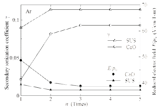
Fig. 14 Variation of secondary ionization coefficient by repeated measurement.
