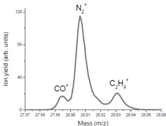
Fig. 1: Analysis of cigarette smoke with a PTR-TOF 8000 instrument equipped with SRI+ after [13].
