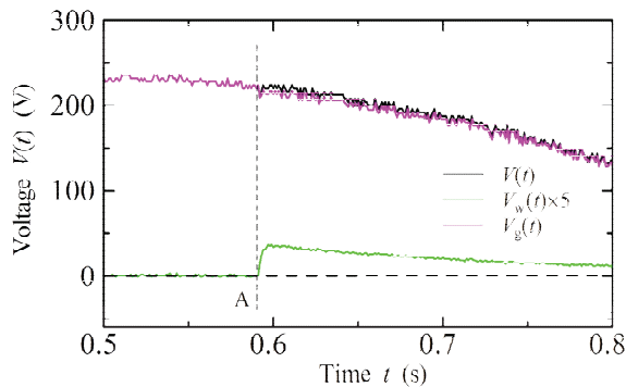
Fig. 3 Enlarged in the vicinity of A of Fig. 2(b) of voltage waveforms.
