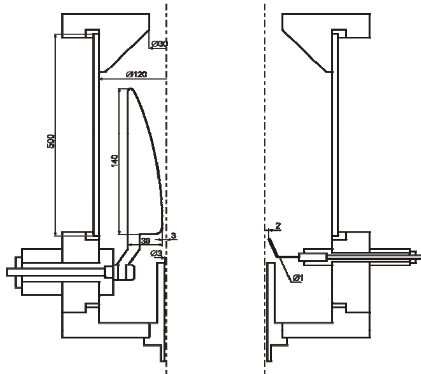
Fig. 2. Geometry of plasma reactor electrodes; a) basic dimensions of discharge chamber with working electrodes; b) ignition electrode
