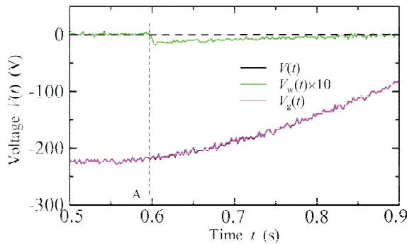
Fig. 8 Enlarged in the vicinity of A of Fig. 5(b) of voltage waveforms.
