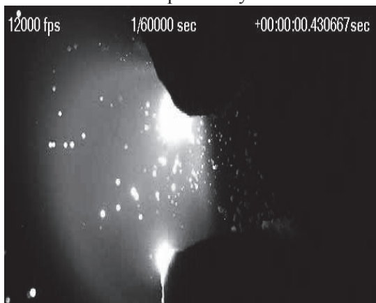
Fig. 5 The immersed arc in IAF
