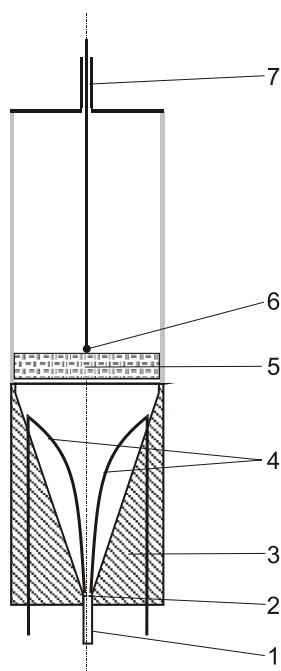
Fig. 1. Gliding discharge reactor for \text{CCl}_4 decomposition with stationary bed. 1 – gas inlet, 2 – nozzle, 3 – ceramic body, 4 – electrodes, 5 – catalyst bed, 6 – thermocouple, 7 – gas outlet.
