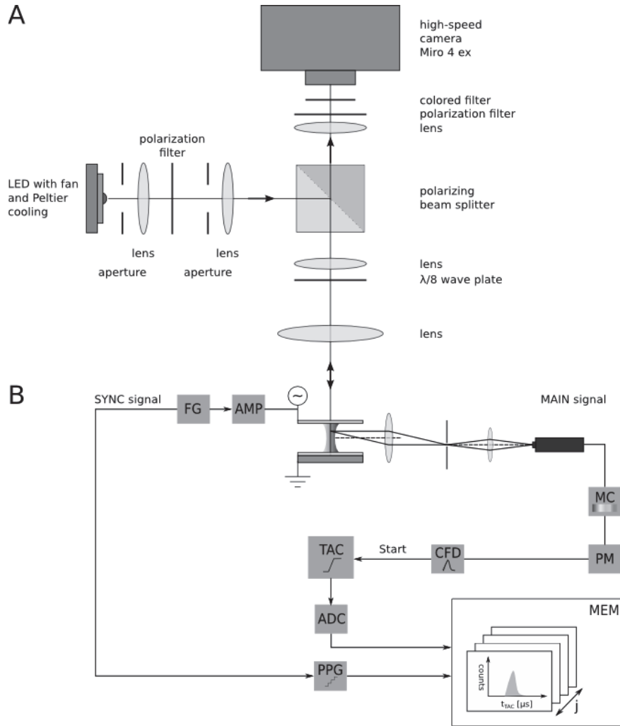
Fig. 2. Experimental set-up for surface charge measurements (A) and spatio-temporally resolved spectroscopic measurements in the volume (B). CCS set-up with PC pattern generator (PPG) triggering: PM - photomultiplier, MC - monochromator, CFD - constant fraction discriminator, TAC - time to amplitude converter, ADC - analogue-digital converter, PPG - pattern generator, MEM - memory.
