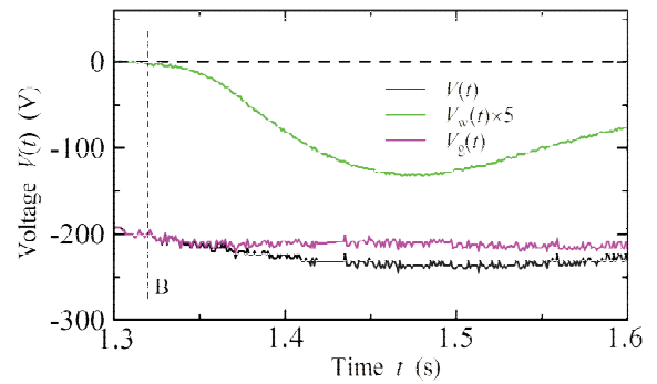
Fig. 4 Enlarged in the vicinity of B of Fig. 2(b) of voltage waveforms.
