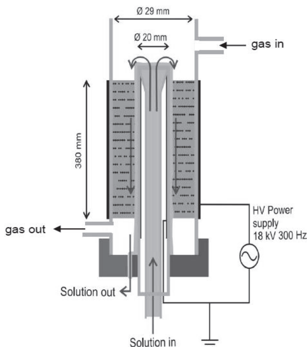
Fig. 1. Coaxial water falling film DBD
