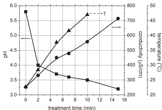
Fig. 2. Conductivity, pH and temperature of the MB solution as a function of plasma treatment time.
