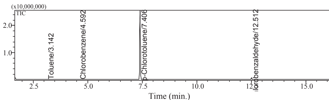
Fig. 2a A GC-MS chromatogram of gas phase by-product of 4-chlorotoluene degradation in air mixture
