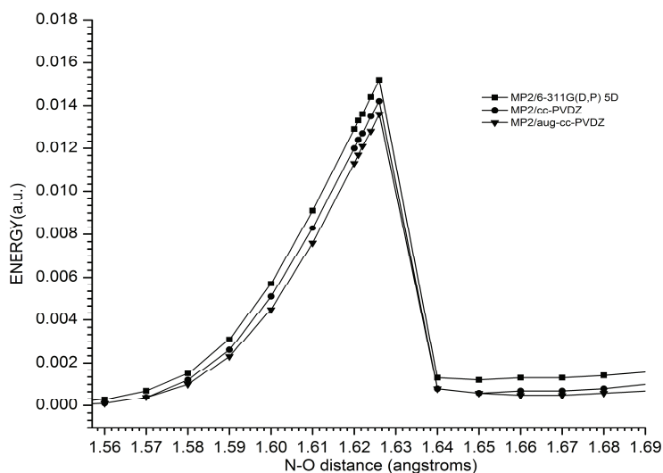
Figure 4. Potential energy vs. N-O distance for the reaction of O_3 with NO_2 modeled using the MP2 level of theory with three basis sets, 6-311G(d,p), cc-pVDZ and aug-cc-pVDZ.
