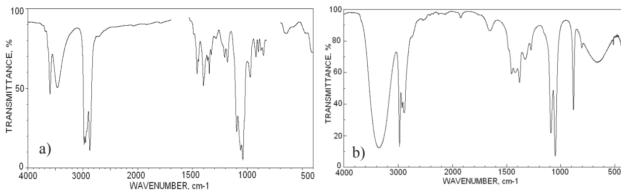
Fig. 2. The IR spectra of a) tetrahydrofurfuryl alcohol [5]; b) ethyl alcohol [5].
