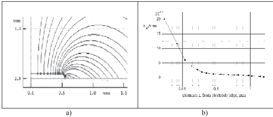
Fig. 3. Distribution of the applied electric field force lines (a) and normal component values E_n at the barrier surface. The electrode thickness is 10 \mu\text{m} .
