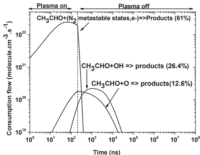
Fig. 5. Computed consumption flow of acetaldehyde for an initial mixture containing 500 ppmC of acetaldehyde and 500 ppmC of acetylene in a 94.5% N 2 /5%O 2 gas flow
