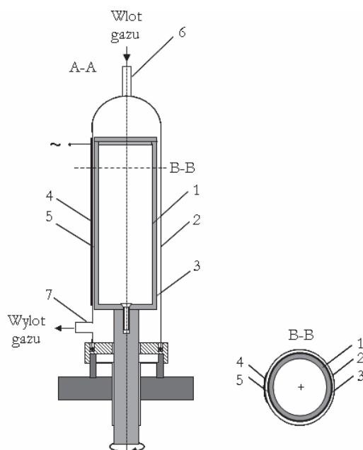
Fig.1. Scheme of the reactor [7] A-A vertical section, B-B horizontal section; 1 – rotating electrode, 2 – glass body, 3 – film, 4 – HV electrode, 5 – discharge gap (2 mm) 6, 7 – inlet and outlet pipes, respectively
