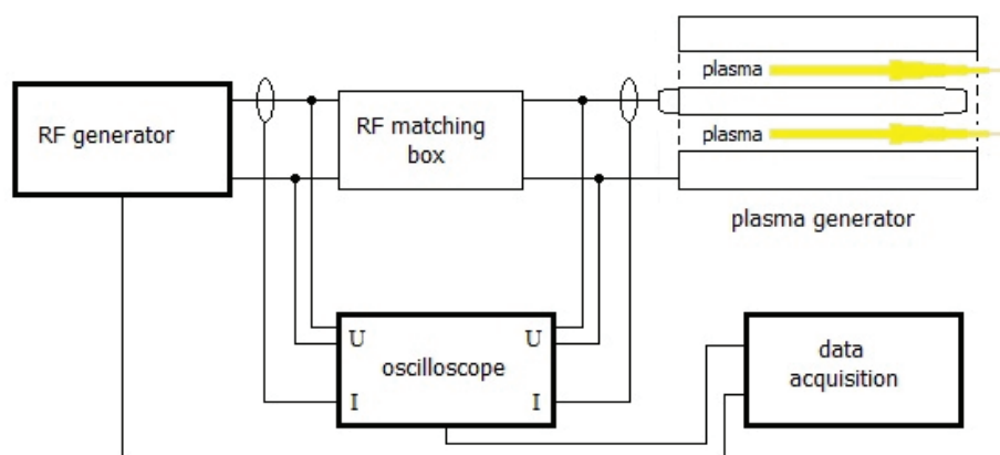
Fig.2. Electrical supply of APPJ.
