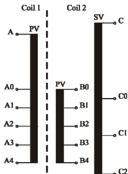
Fig. 4. Position of transformer's windings
