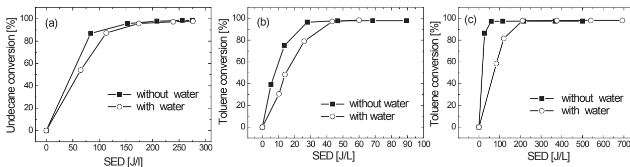
Fig. 2. Conversion efficiency of: a) undecane, b) 20 ppm toluene, c) 40 ppm toluene with and without water film in the reactor
