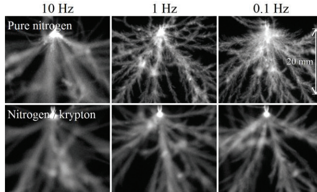
Figure 3. Zoomed images around the cathode tip of repetitive streamer discharges created with the Blumlein pulser (pulse length 130 ns) at 25 kV at three different pulse repetition frequencies in pure nitrogen and the nitrogen/krypton mixture.
