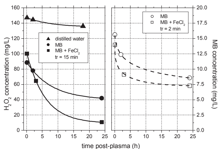
Fig. 5. Post-plasma evolution of the H_2O_2 and MB concentrations (tr – plasma treatment time).
