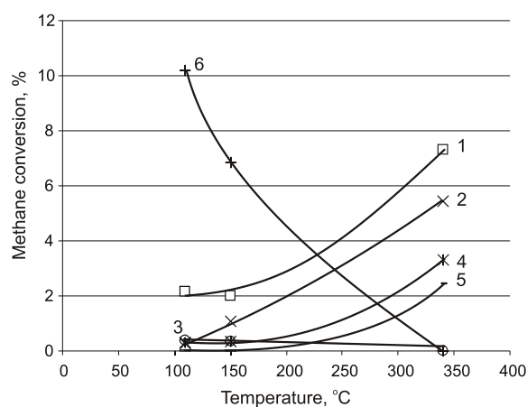
Fig. 8. Effect of temperature on methane conversion to hydrocarbons (1- C 2 H 6 , 2- propane, 3 - n-butane, 4 - i-butane, 5 - 2-butene) and methanol (6). Molar ratio [CH 4 ]: [O 2 ]=3:1, Power – 15 W, argon conc. 25%. Gas flow rate 2 NI/h.
