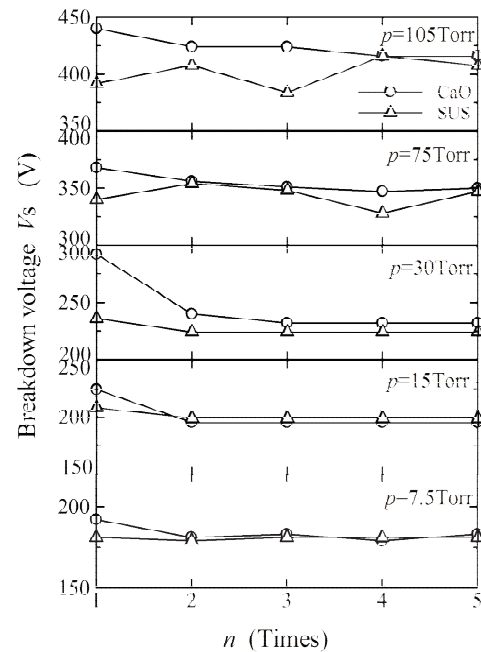
Fig. 11 Variation of breakdown voltage by repeated measurement.
