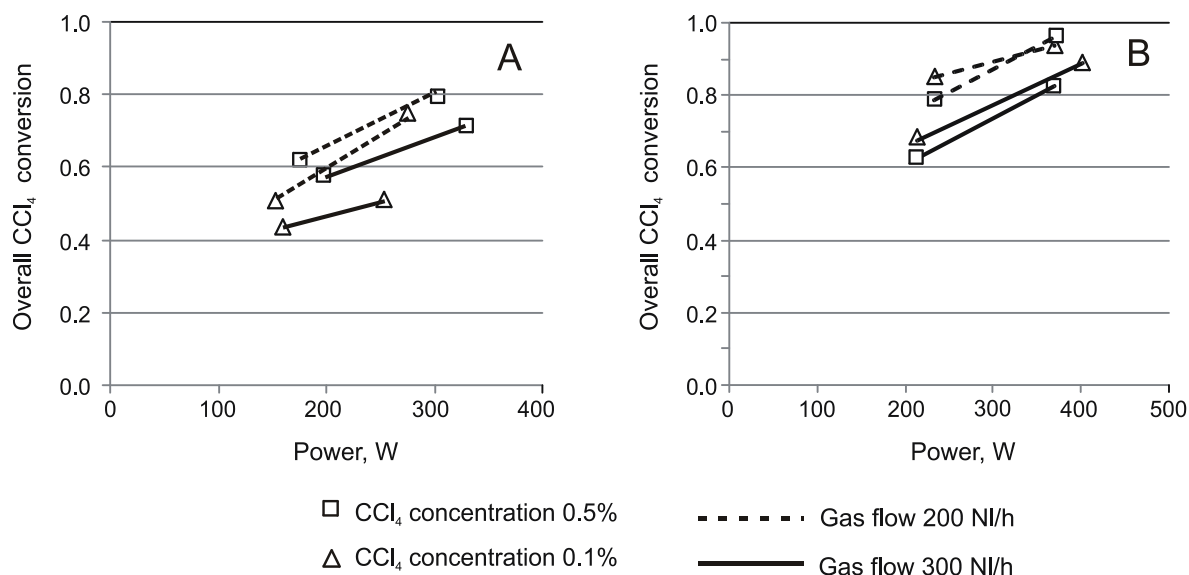
Fig. 3. Effect of gas flow and \text{CCl}_4 concentration on overall \text{CCl}_4 conversion. A – homogeneous system, B - plasma catalytic system with \text{V}_2\text{O}_5 + \text{K}_2\text{O} /diatomite.
