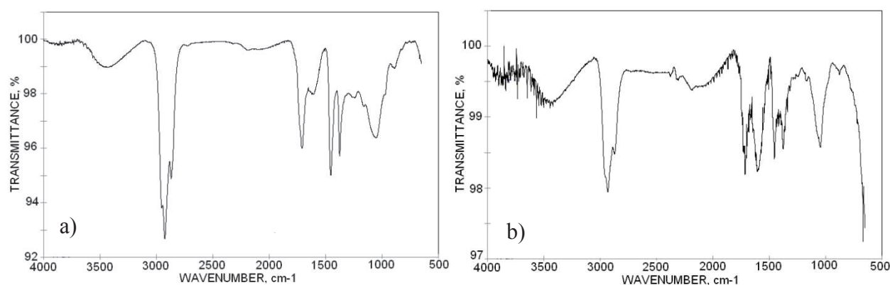
Fig. 3 The IR spectra of the layers obtained on the copper substrate: a) the sample after processing with the use of the first stage of the method I - Cu 5, b) the sample after processing with the use of both stages of method I -Cu 3.
