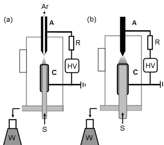
Fig. 1. The experimental set-up for the APGD system containing a) argon microjet-liquid cathode and b) solid anode-liquid cathode (A-anode, C-cathode, R-ballast resistor, HV-high voltage direct current power supply, S-initial solution, W-water solution treated by the discharge).
