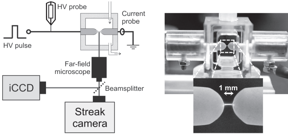
Fig. 1. Experimental set-up with diagnostic (left) and photos of the discharge cell with MD (right).
