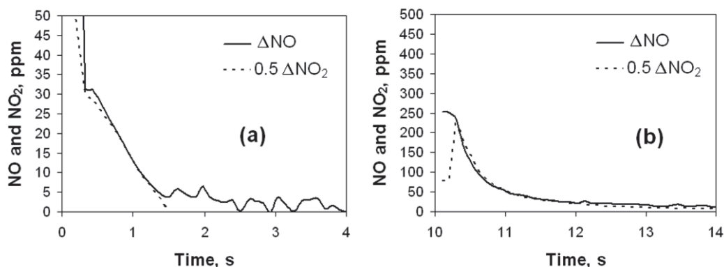
Fig. 6. Time-dependences of outlet values of \Delta\text{NO} and \Delta\text{NO}_2 (a) at the switch-on and (b) after the switch-off of the ozone generator.
