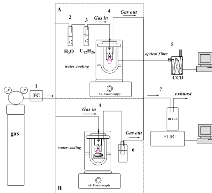
Fig 1. Schematic diagram of experimental configuration for experiments A) in the gas phase and B) in the liquid phase: 1) mass flow controller, 2) bubbler with water, 3) bubbler with dodecane, 4) AC GAD reactor, 5) Optical emission spectrograph, 6) liquid N 2 cold trap, 7) gas FTIR sample inlet
