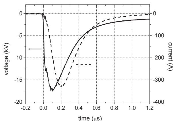
Fig. 1. Waveforms of the discharge voltage and current after 2 min plasma treatment.
