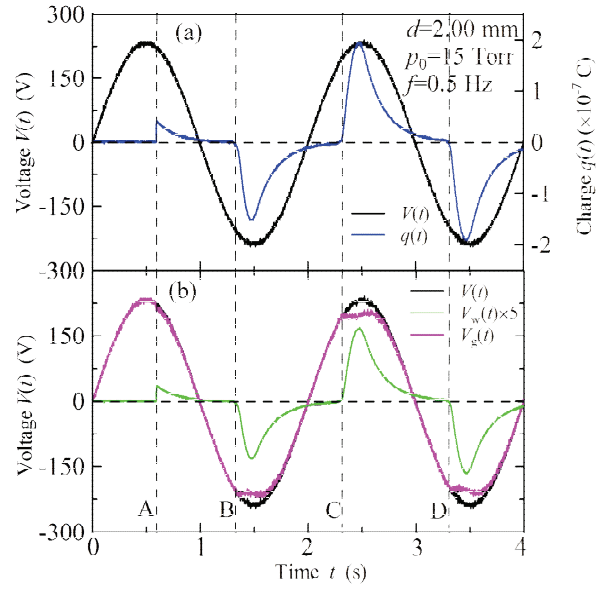
Fig. 2 Voltage and charge waveforms. ( d = 2.00 mm, p_0 = 15 Torr, f = 0.5 Hz)
