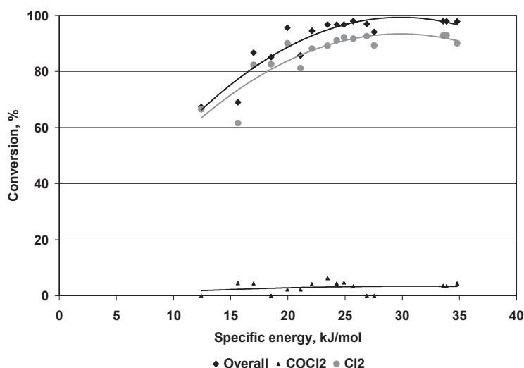
Fig. 5. The dependence between the \text{CCl}_4 conversion and specific energy for AC power supply system.
