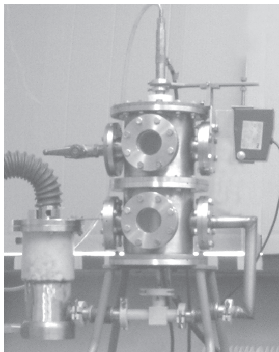
Fig. 2. Photo of parts of system (reactor with actuator and catalytic oxidizer).
