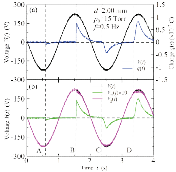
Fig. 7 Voltage and charge waveforms. ( d = 2.00 mm, p_0 = 15 Torr, f = 0.5 Hz)
