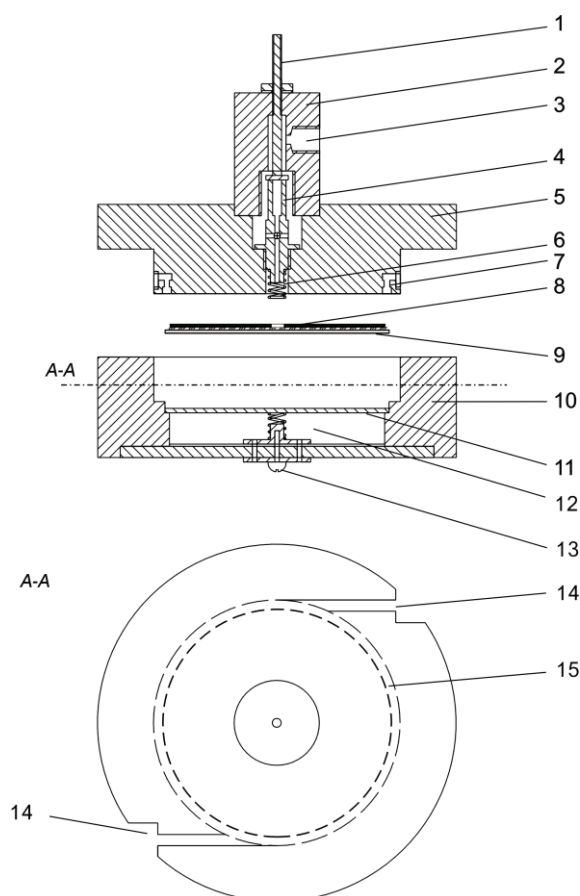
Fig 1. Cross-section of the ozonizer. In the A-A cross-section the idea of gas feeding system is presented; 1 – high voltage clamp, 2 – insulator, 3 – outlet of the post-reaction gas, 4 – gas ejector and voltage supply element, 5 – reactor lid, 6 – contact spring, 7 – openings through which the gas enters the reaction space, (8+9) – removable discharge element, 8 – sputtered electrode or metal mesh, 9 – ceramic plate, 10 – main body of the reactor, 11 – wall of the cooling chamber, 12 – cooling chamber, 13 – grounding clamp, 14 – gas inlet channels, 15 – collecting ring.
