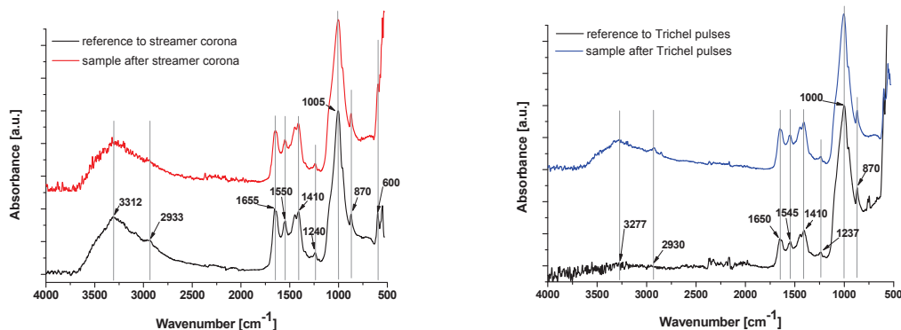
Fig. 7. ATR FTIR spectra of the tooth samples after: a) positive streamer corona b) negative Trichel pulses with their respective references (black).
