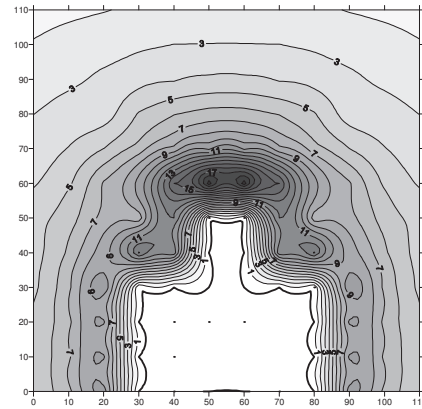
Fig. 4. Magnetic field around the cathode (in mT). Isolines show the location of the same field strength).
