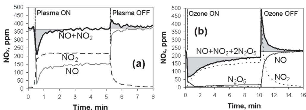
Fig. 5. Time-dependence of NO, \text{NO}_2 , \text{N}_2\text{O}_5 and \text{NO}_x concentration in (a) hybrid reactor and (b) ozone injection reactor with \text{Fe}_2\text{O}_3 catalyst at room temperature.
