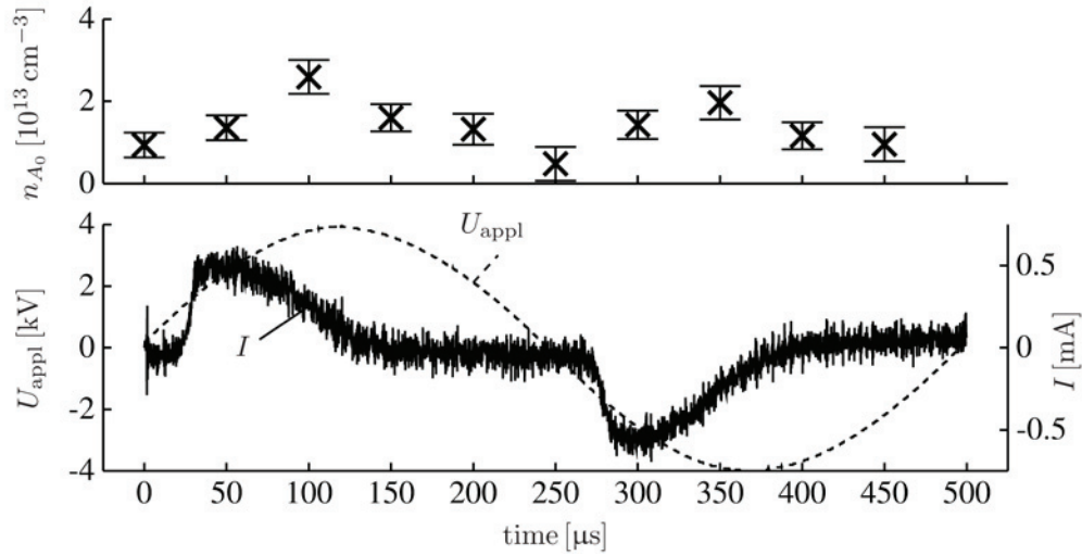
Fig. 5: Time dependent A^3\Sigma_u^+, v=0 density in the centre of the diffuse discharge configuration at 500 mbar, 2 kHz, and 8.00 kV pp .
