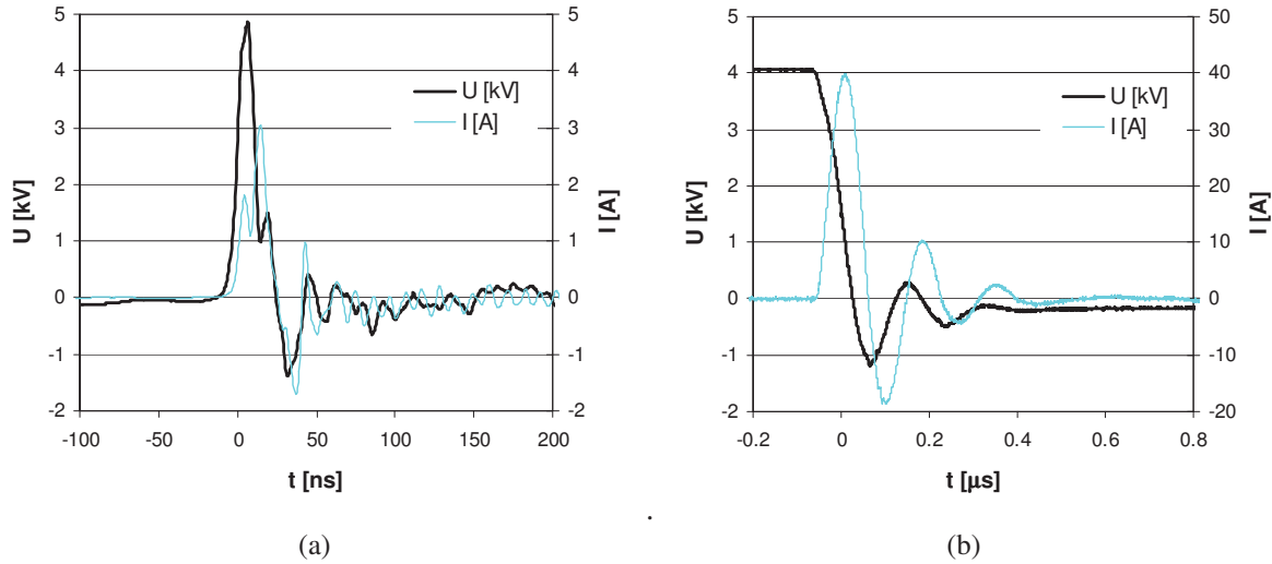
Fig. 2. Typical voltage and current pulse waveforms of (a) NRP discharge and (b) TS operated in the CH_4 -air premixed flame at total gas flow Q=4 Nm 3 /h and \Phi=0.8 .
