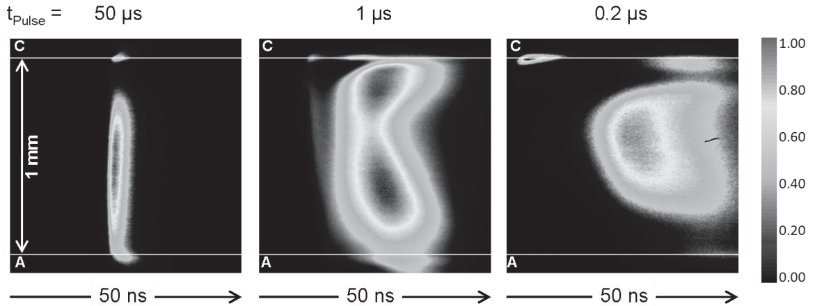
Fig. 5. MD development at falling slope by changing D resp. t_{\text{pulse}} (accumulation of 1,000 MDs, linear intensity scale).
