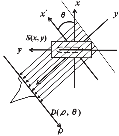
Fig. 2. Top view of electrodes module and relation between the coordinates of (x, y) and (x', y') .
