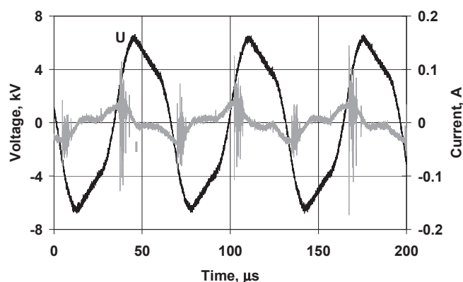
Fig. 4. Traces of pulses voltage and current for pulsed current of 15 kHz frequency power supply system.
