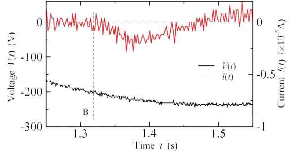
Fig. 6 Current in the vicinity of A of Fig. 2.
