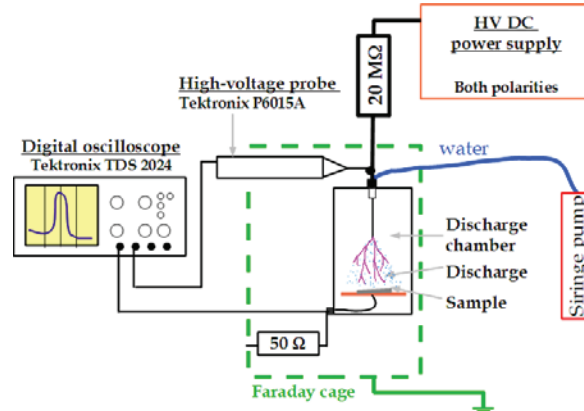
Fig. 1. Schematic of discharge set-up for corona on teeth or plastic surfaces.
