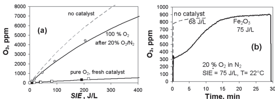
Fig. 2. Ozone concentration in the outlet of the hybrid plasma-catalytic reactor. (a) Stabilized values when ozone was produced from pure O 2 either in the presence of the fresh catalyst (Fe 2 O 3 ) or in the presence of catalyst, which was previously exposed to discharge in the mixture of 20% O 2 /N 2 . (b) Time dependence of the ozone concentration produced from 20% O 2 /N 2 mixture without the presence of catalyst (dashed line) and in the presence of Fe 2 O 3 catalyst (solid line).
