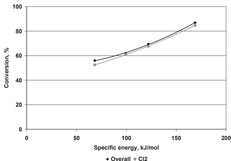
Fig. 7. The dependence between the \text{CCl}_4 conversion and specific energy for pulsed current of 15 kHz frequency power supply system.
