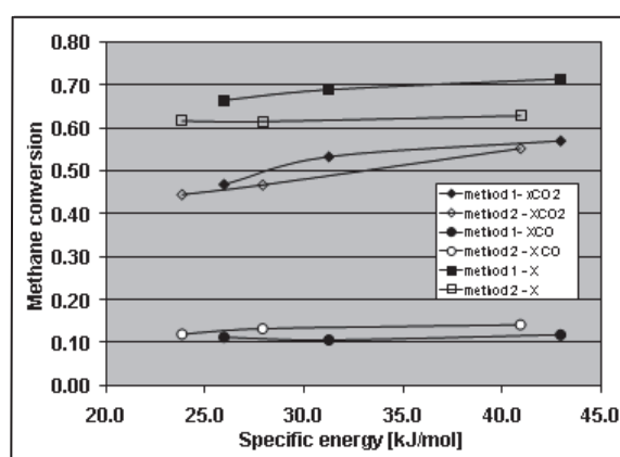
Fig 6. Methane conversion vs. specific energy of the total flow of all gases introduced into the reactor for two methods of the mixture of methane and argon introduction into the reactor: 1- through the mixing nozzle; 2- through the outer nozzle. The experiments conditions were as follows: 1- an initial concentration of methane in the mixture of input gases was 3.15 \pm 0.09 vol.% and 2- the total flow of input gases was 3.45 \div 7.50 \text{ Nm}^3/\text{h} .
