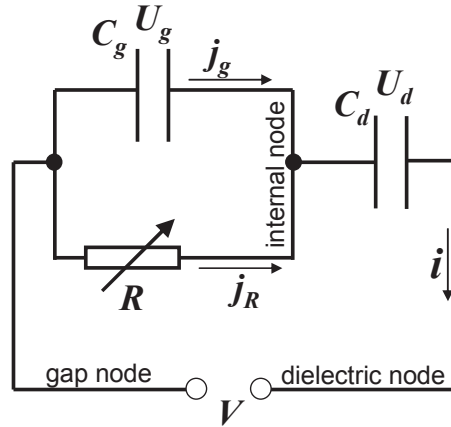
Figure 1. Simplest equivalent circuit of a DBD.
