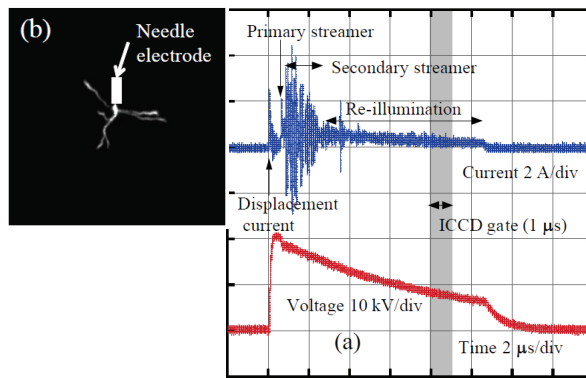
Fig. 3. (a) Applied voltage and current waveforms. (b) Corresponding secondary streamer image captured by light emission through the re-illumination stage (gray colored period in figure (a)).
