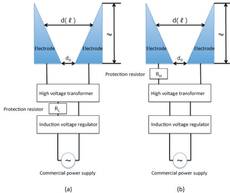
Fig.1. Gliding arc discharge system
