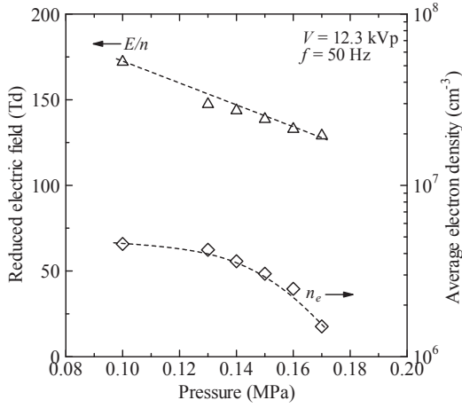
Fig. 7. E/n vs. n_e (effect of gas pressure).
