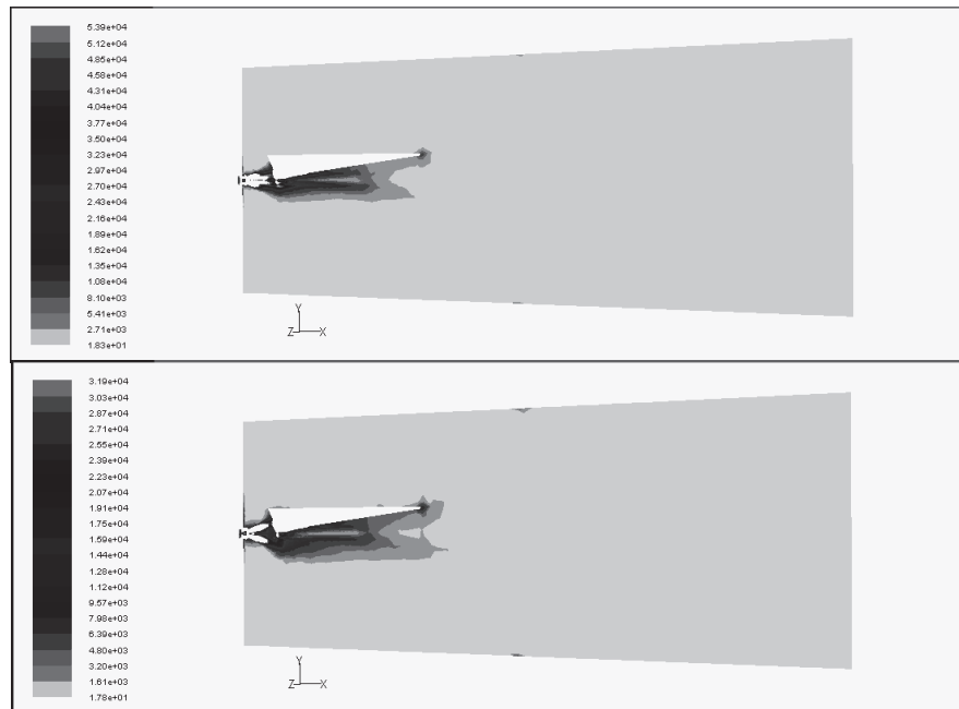
Fig.4 The distribution of shear stresses in the stream of gases in the plane of symmetry. The mixture of methane and argon was introduced into the reactor using: a - the first method, b – the second method (methane oxidation was considered).
