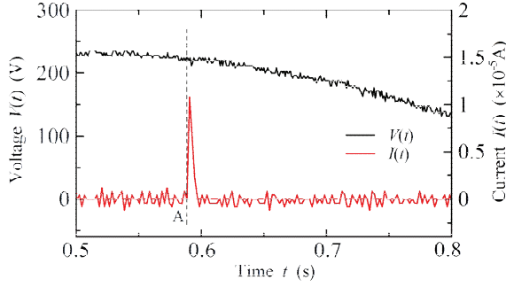
Fig. 5 Current in the vicinity of A of Fig. 2.
