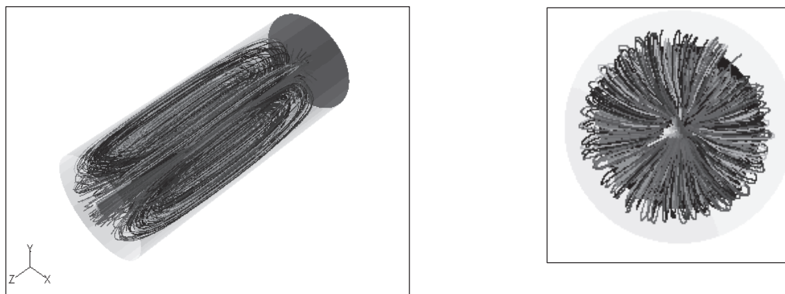
Fig. 2 Runs of stream lines in the reactor. Methane oxidation was not considered.
