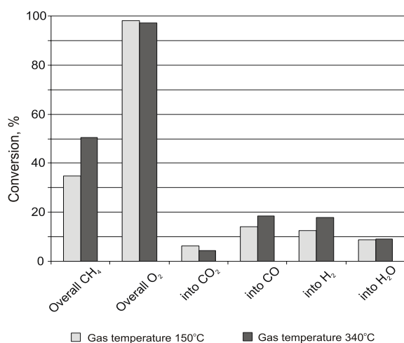
Fig. 3. Effect of temperature on overall conversion of methane and oxygen and conversion of methane to H 2 , CO, CO 2 , and H 2 O. Power – 19 W, initial argon concentration 50%. Gas flow rate 2 NI/h.
