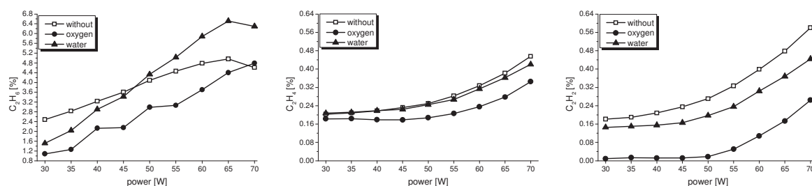
Fig. 4. Amount of the C2 hydrocarbons as a function of the power and different additives (ethane (left), ethene (middle), and ethine (right)).
