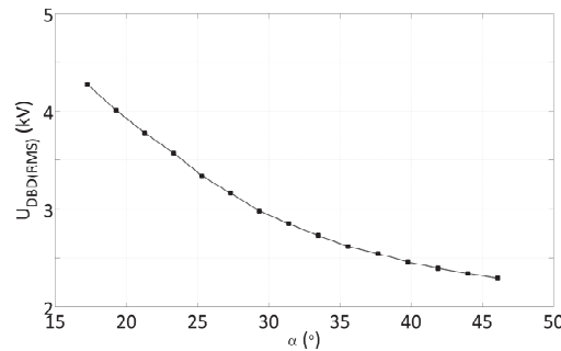
Fig. 6. The output voltage – control pulse phase delay (with respect to U_{C2} zero point crossing) dependency.
