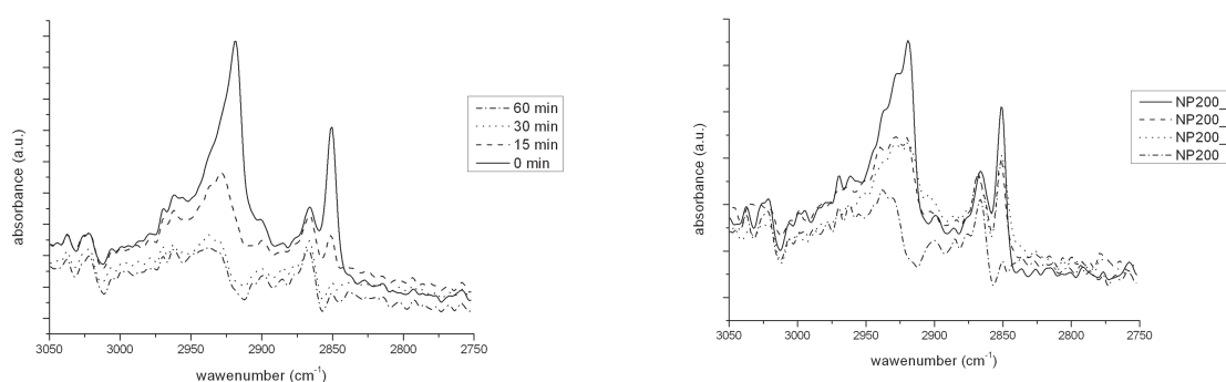
Fig. 2. FTIR spectra of C–H bonds in stearic acid of NP200 at three different exposure times (a), and the comparison of the photoactivity at 30 minutes of UV-light exposure, after three different plasma treatments (b).
