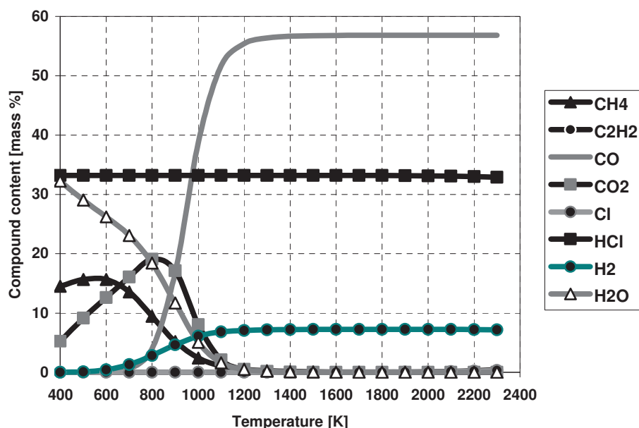
Fig. 6 Thermal decomposition of gaseous fraction of methanol and carbon tetrachloride mix (66%/34%)
