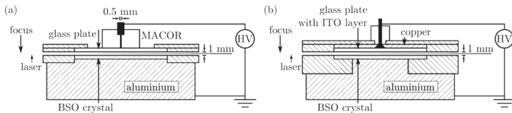
Fig. 1: Cross section of the discharge cells used for the (a) filamentary and (b) diffuse discharge mode.
