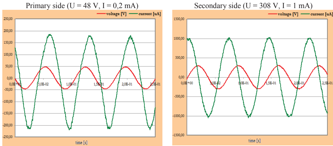
Fig. 4. Voltage/current characteristics
