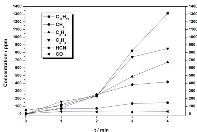
Fig 5. Gaseous products distribution during nitrogen gliding arc plasma-liquid treatment of dodecane
