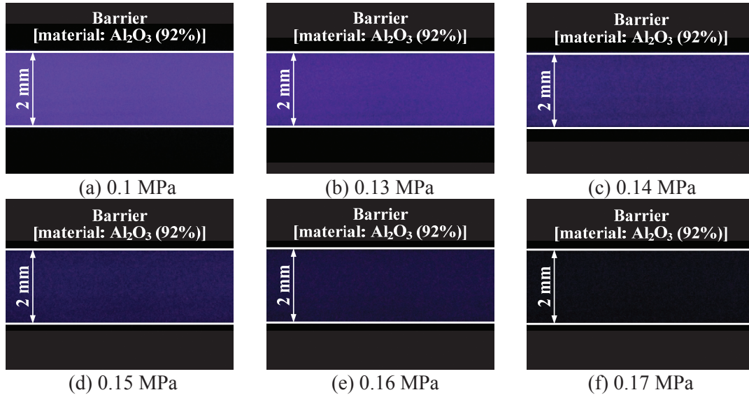
Fig. 4. Discharge photographs.
