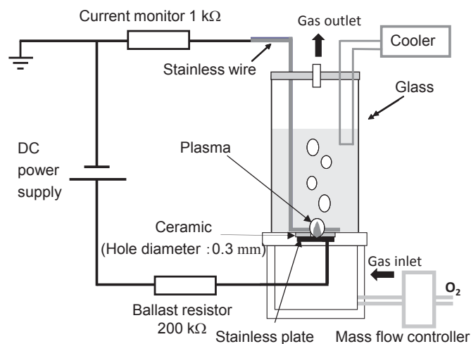
Fig. 1 Schematic diagram of plasma reactor.
