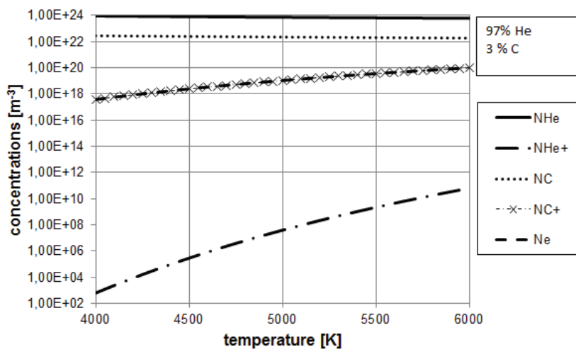
Fig.2. Concentration of plasma components for helium-carbon plasma for 3% amount of carbon.
