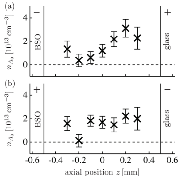
Fig. 4: Axial A^3\Sigma_u^+, v=0 density profiles for the (a) positive and (b) negative half cycle in the filamentary mode at 500 mbar, 5 kHz, 12.50 kV pp , and 30 \mu s after zero-crossing of the voltage.
