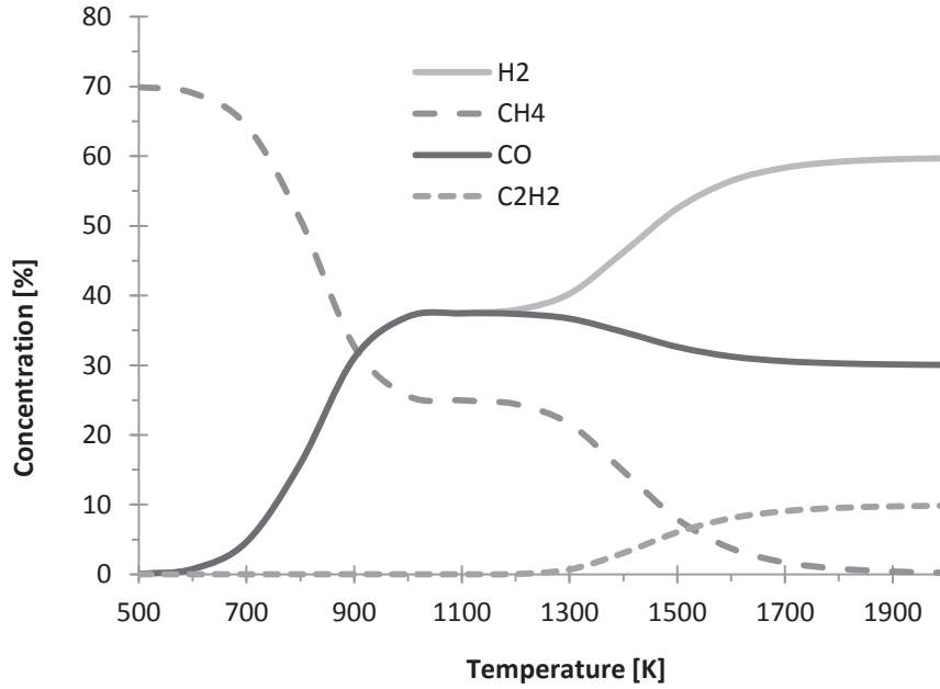
Fig. 6. Concentrations of \text{CH}_4 and its conversion products calculated for thermodynamic equilibrium.
