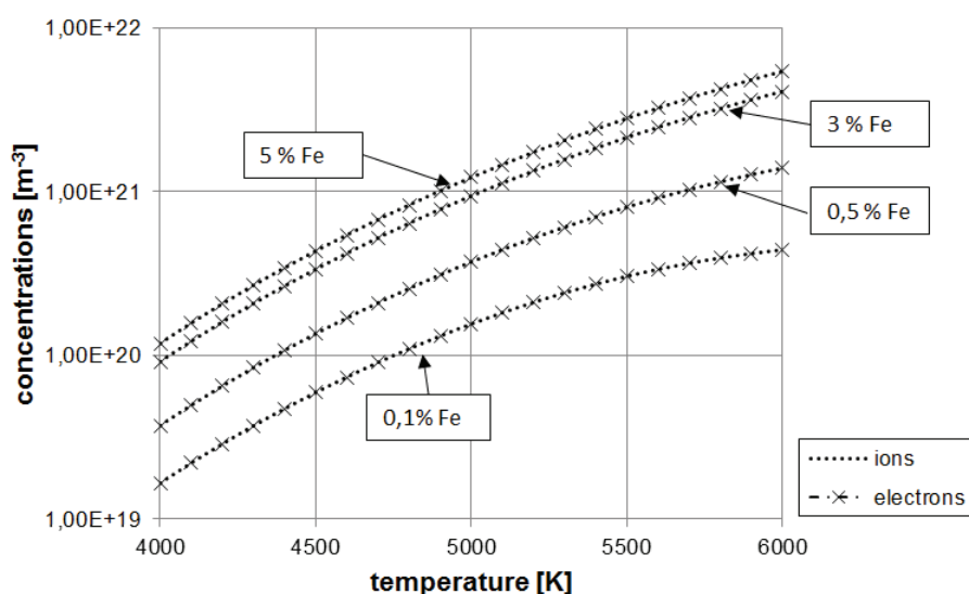
Fig. 4. Comparison of electrons and ions densities for different amounts of iron.
