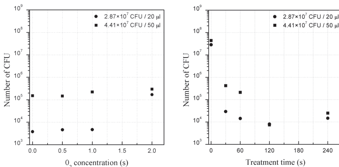
Fig. 3. The influence of the O 2 admixture (a) and treatment time (b) on the Escherichia coli deactivation. Ar flow rate of 10 l/min. In (b) the admixture of O 2 0.5 %. (●) The initial number of colony forming units was 2.87 \times 10^7 per sample droplet volume of 20 \mu l. The incident microwave power 68 W, the reflected microwave power 41 W. (■) The initial number of colony forming units was 4.41 \times 10^7 per sample droplet volume of 50 \mu l. The incident microwave power 72 W, the reflected microwave power 42 W.
