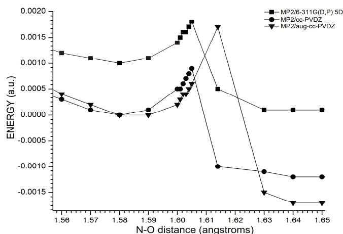
Figure 3. Potential energy vs. N-O distance for the reaction of O 3 with NO modeled using the MP2 level of theory with three basis sets, 6-311G(d,p), cc-pVDZ and aug-cc-pVDZ.
