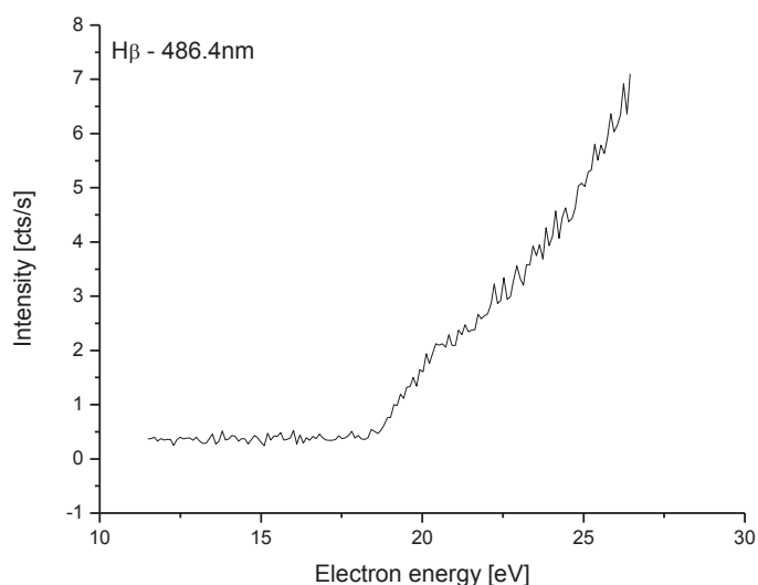
Fig. 2. Example of the measured excitation curve for H_{\beta} line.
