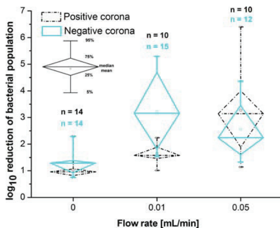
Fig. 5. Reduction of bacterial population on teeth by corona discharges with water electro-spraying for various flow rates (exp. time 5 min)
