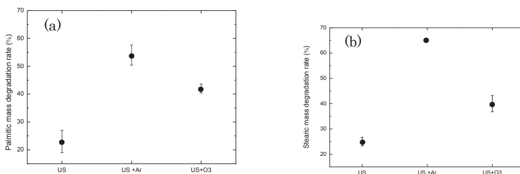
Figure 2: Percent of palmitic acid (a) and stearic acid (b) mass degradation rate under various treatment procedure: sonication only (US), sonication simultaneously with argon bubbles (US + Ar) and sonication simultaneously with ozone bubbles (US + \text{O}_3 ).
