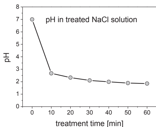
Fig. 3. The pH of NaCl solution dependent on plasma treatment time
