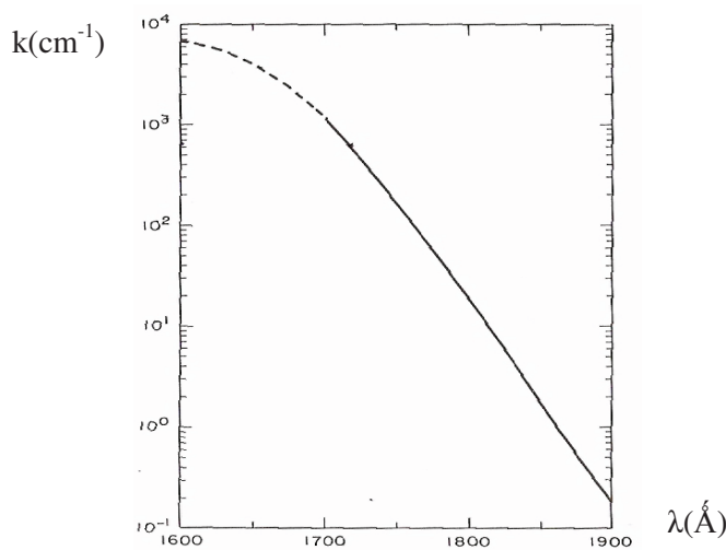
Fig.1. Absorption coefficient of distilled water [9].
