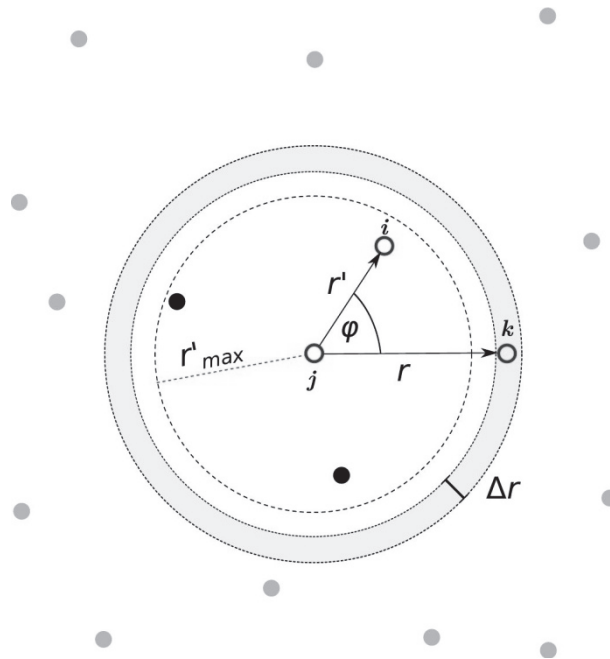
Fig. 2.: Graphical representation of the Triple Correlation Function (TCF). The distances r' and r and the angle \varphi of any filament triple (i,j,k) are determined. Filaments within a distance r'_{\text{max}} are considered for calculation of both r and r' relative to j , others are solely used for calculation of r relative to j .
