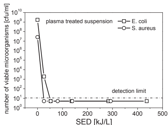
Fig. 7. Inactivation of E. coli and S. aureus in direct plasma treatment as a function of SED
