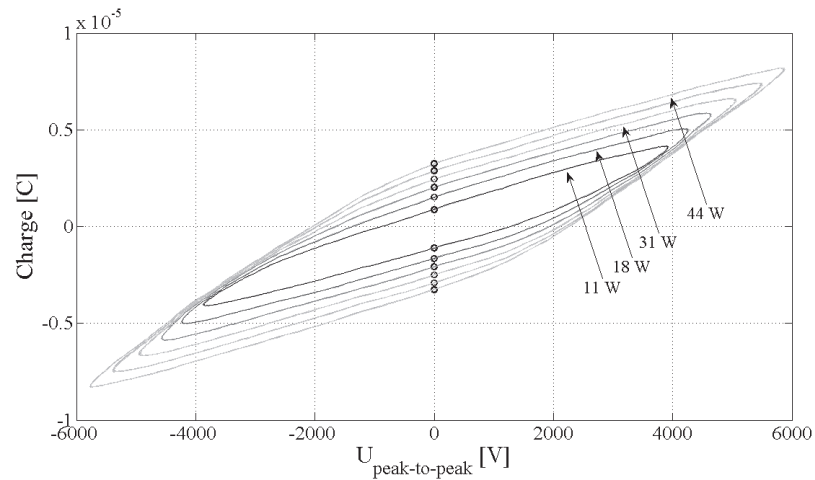
Fig. 2. Lissajous curves for alternating reactor power levels.
