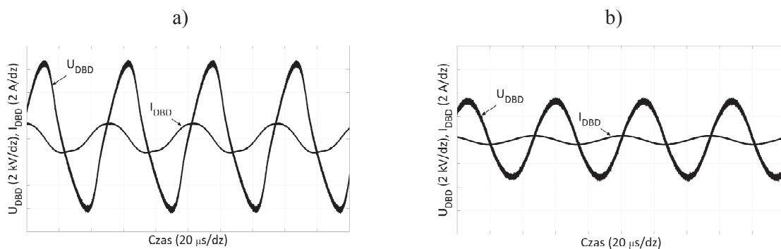
Fig. 8. DBD reactor voltage and current waveforms for two different delay angles: a) \alpha = 17,2^\circ ; b) \alpha = 46^\circ .
