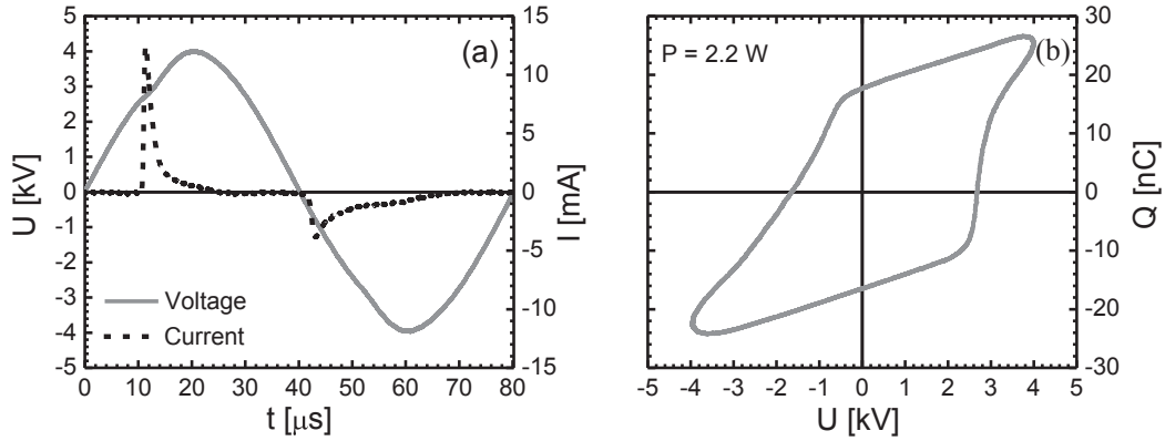
Fig. 2. (a) Current and voltage signals of the plasma jet operating in the bullet mode. (b) Lissajous figure (Q-U plot) showing dissipated power.
