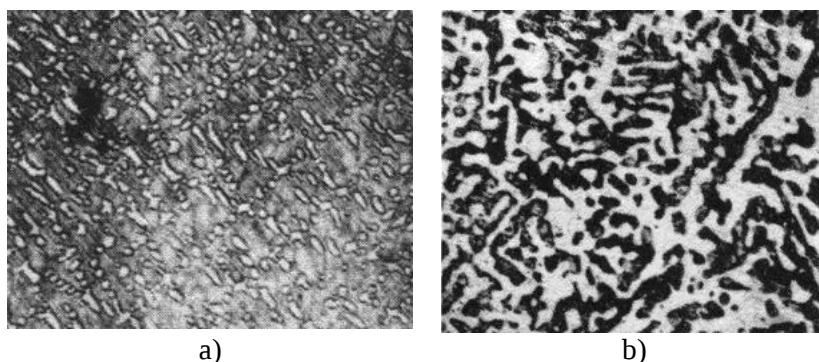
Fig. 4.5. Microstructure ( \times 200 ) of sub-eutectic alloy, sample no. 7 (markings according to Tab. 4.6); a) after normalising; b) after annealing at 1273 K, 350 h
