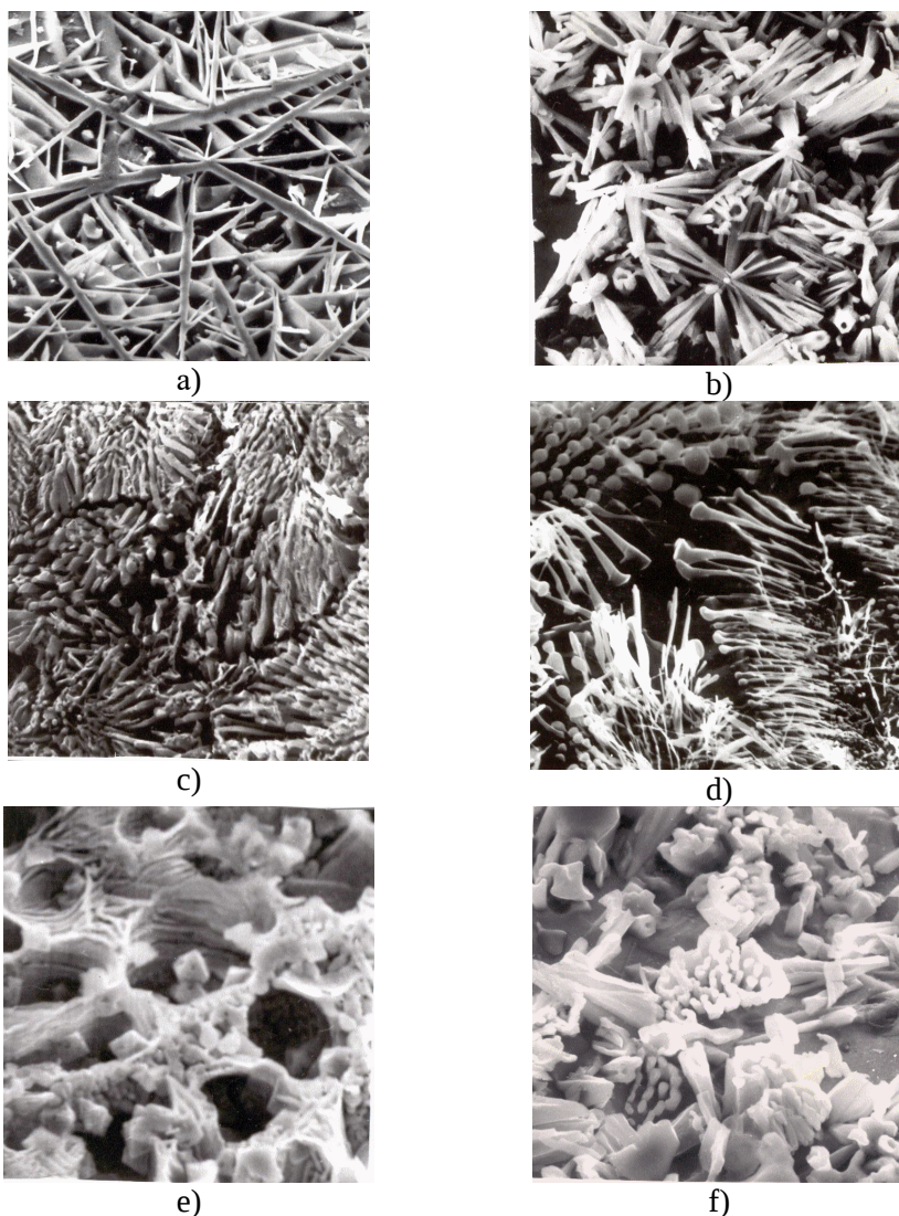
Fig. 1.4. The quasi-binary eutectic alloys colonial structures due to the cooperative phases growth. Scanning electron microscopy. a) Fe-ZrB 2 , x 500; b) Fe-TiB 2 , x 1500; c) Fe-VC, x 3000; d) Mo-TiN, x 3000; e) the iron-based alloy VTiNi, x 2000; f) Fe-TiC-TiB 2 , x 1500
