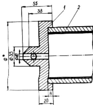
Fig. 3.18. Sealing flange for fixing a steel blank: 1 – flange; 2 – blank
