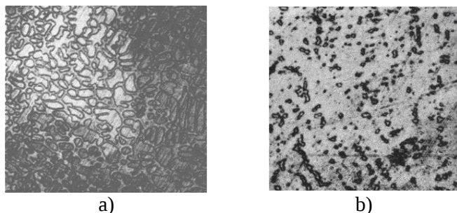
Fig. 4. 4. Microstructure ( \times 200 ) of the examined Fe 3 C-Fe 3 B-‘Fe 1.2 Mn’ quasi-ternary intersection alloys (markings according to Tab. 4.5): a) sample no. 13, sub-eutectic alloy after normalising; b) solid solution, sample no. 20, after annealing at 1273 K, 350 h
