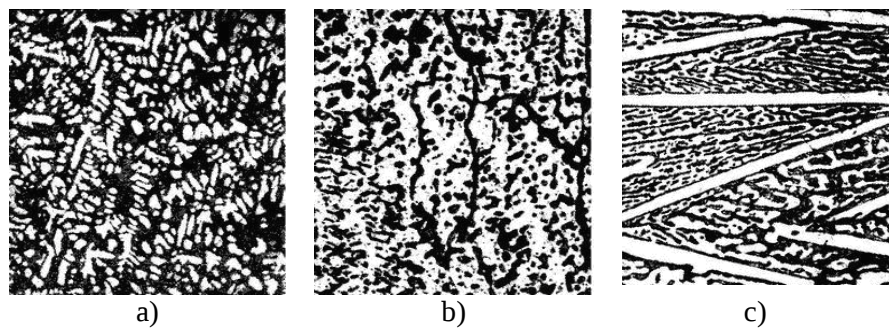
Fig. 4. 2. Microstructure ( \times 200 ) of the examined samples (markings according to Tab. 4.3), hyper-eutectic alloy [a, b] sample no. 3] and solid solution [c] sample no. 5]; a) after normalising; b, c) after annealing (at 1273 K, 350 h)
