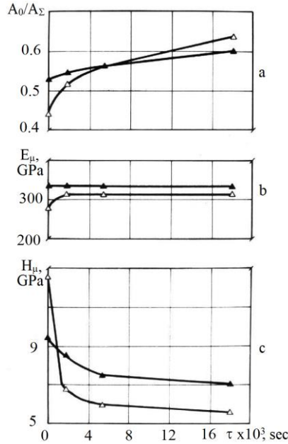
Fig. 2.10. Change of properties of light areas ( \Delta ) and colonial structures ( \blacktriangle ) of VTiNi plasma coating depending on annealing time ( T = 0.75T_{\text{melt}} ): a) ductility, A_0/A_\Sigma ; b) modulus of elasticity, E_\mu ; c) microhardness H_\mu
