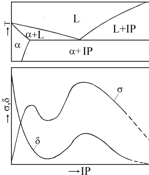
Fig. 1.5. Dependence of the alloys strength ( \sigma ) and ductility ( \delta ) vs. interstitial phase content (IP)
