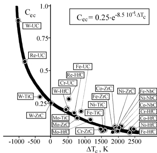
Fig. 1.1. The dependence of quasi-binary metal-carbide eutectic alloys composition ( C_{ec} ) on the difference between the melting points of the carbide and the metal matrix ( \Delta T_c )
