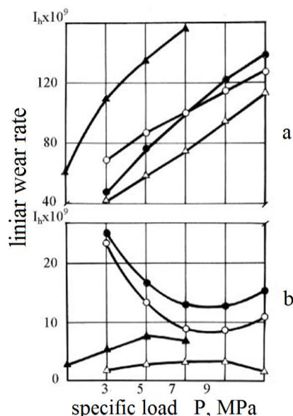
Fig. 2.11. Linear wear rate vs. specific load (sliding speed 0.25 m/sec): a) counterface (hardened steel 1080); b) plasma coating VTiNi. \blacktriangle – as-deposited coating; \Delta, \circ, \bullet – annealed coatings for 18 \times 10^2 , 54 \times 10^2 , 18 \times 10^3 sec respectively
