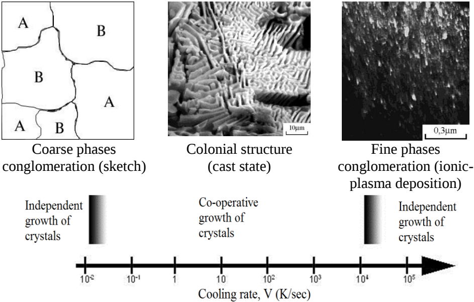
Fig. 2.1. Schematic representation of the three mechanisms of eutectic crystallization depending on the cooling rate of VTiNi alloy and the corresponding structures (in accordance with A. Bochvar)
