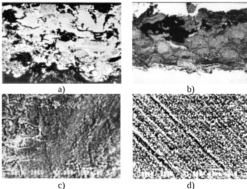
Fig. 3.7. Microstructure a, b) of plasma VTiNi-powder coating, \times 200 , and c, d) wear scar, \times 500
