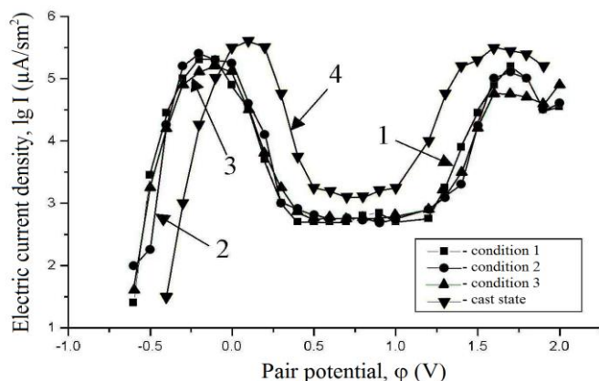
Fig. 2.8. Potentiostatic curves of the detonation eutectic coatings and the standard sample: 1 – VTiNi; 2 – 12Cr18Ni9 (standard sample); 3 – CrVC; 4 – CrTiNi
