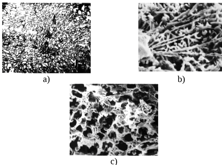
Fig. 3.1. Microstructure of a, b) TiNi and c) CrTiNi eutectic coatings: a – \times 312 ; b, c – \times 2700
