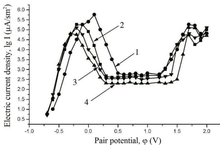
Fig. 2.6. Potentiostatic curves of the plasma eutectic coatings and the standard sample 1 – VTiNi; 2 – 12Cr18Ni9 (standard sample); 3 – CrVC; 4 – CrTiNi
