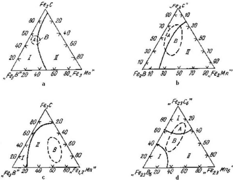
Fig. 4.1. Phase areas (I, II, A, B) in quasi-ternary intersections: a) Fe_3C - Fe_3B - Fe_3Mn , b) Fe_2C - Fe_2B - Fe_2Mn , c) Fe_3C - Fe_3B - Fe_{1.2}Mn , d) Fe_{23}C_6 - Fe_{23}B_6 - Fe_{23}Mn_6
