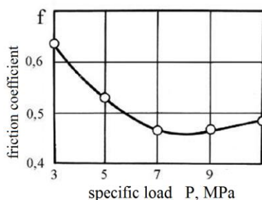
Fig. 2.16. Friction coefficient of VTiN detonation coating (annealed for 18 \times 10^2 sec) vs specific load
