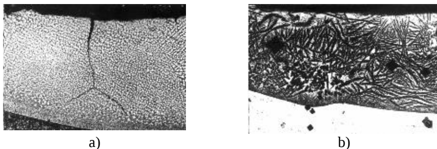
Fig. 3.11. Microstructure of alloyed layer produced using the following paste: amorphous boron+ \text{B}_4\text{C} : a) steel 1080, \times 200 ; b) steel 12Cr18Ni9Ti, \times 200
