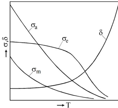
Fig. 1.6. Dependences of metal strength ( \sigma_m ), metal based alloys ( \sigma_a ) and quasi-binary eutectic alloys with interstitial phases ( \sigma_e ) (with the same basic metal) vs. temperature
