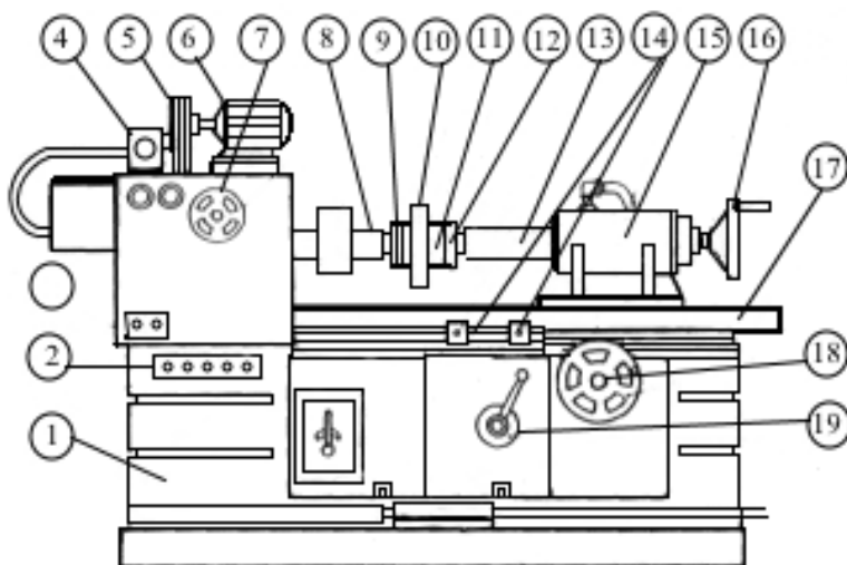
Fig. 3.17. Lathe of ZA250 model, re-equipped for centrifugal bimetalization with induction heating: 1 – frame; 2 – control panel; 3 – buttons for switching on and off the heating; 4 – tachometer; 5 – the pulley belt drive; 6 – electric motor; 7 – flywheel of variator; 8 – spindle of machine tool; 9,12 – sealing caps; 11 – heated sleeve; 10 – circular inductor; 13 – quill of tailstock; 14 – end stops for switching the reciprocating movement; 15 – tailstock; 16 – mechanism of pressing the sleeve; 17 – table of the machine tool; 18 – handwheel of table manual movement; 19 – handle for turning on the reciprocating motion of the table
