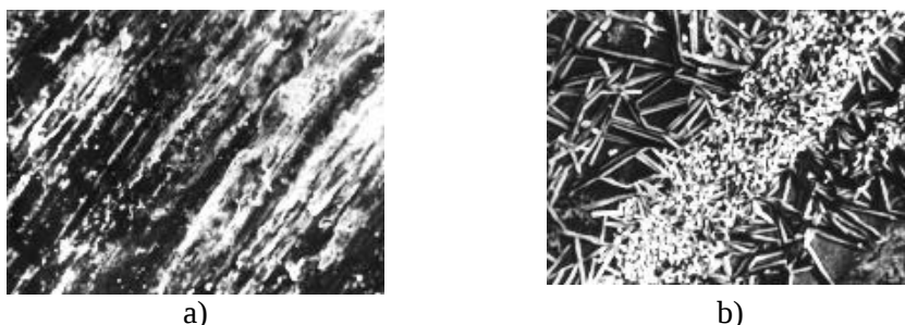
Fig. 3.9. Microstructure of wear tracks of remelted VTiNi eutectic plasma coating at temperatures: a) 850 °C, \times 43 ; b) 850 °C, \times 750
