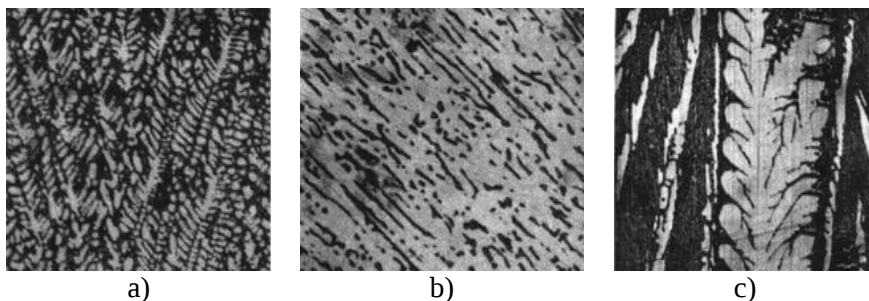
Fig. 4.3. Microstructure (×200) of the examined ‘Fe 2 C’–Fe 2 B–‘Fe 2 Mn’ quasi-ternary intersection alloys (markings according to Table 4): a, b) sample no. 3, c) sample no 10; a, c) after normalisation; b) after annealing at 1273 K, 350 h
