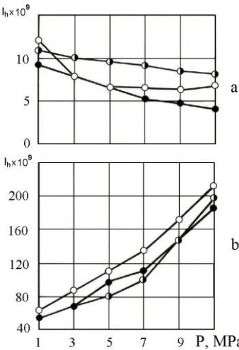
Fig. 2.13. Linear wear rate vs. specific load (sliding speed 0.25m/sec): a) detonation coating CrTiNi; b) counterface (hardened steel 1080). The coatings were annealed for: ○ – 18 \times 10^2 , ◐ – 54 \times 10^2 , ● – 18 \times 10^3 sec respectively
