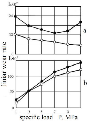
Fig. 2.12. Linear wear rate vs. specific load (sliding speed 0.25m/sec): a) detonation coating VTiNi; b) counterface (hardened steel 1080). ● – as-deposited coating; ○ – annealed coating for 54 \times 10^2 sec
