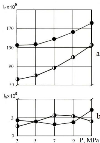
Fig. 2.14. Linear wear rate vs specific load (sliding speed 0.25m/sec): a) counterface (hardened steel 1080); b) detonation coating CrVC.
