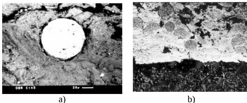
Fig. 3.6. Microstructure of VTiNi plasma coating: a) surface general view (steel 1045); b) cross section, substrate – steel 1080 ( \times 500 )
