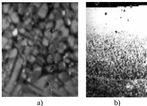
Fig. 3.8. Microstructure of laser melted VTiNi plasma coating: a) substrate – steel 12Cr18Ni9Ti, \times 300 ; b) substrate – carbon steel 1080 (double remelting), 500
