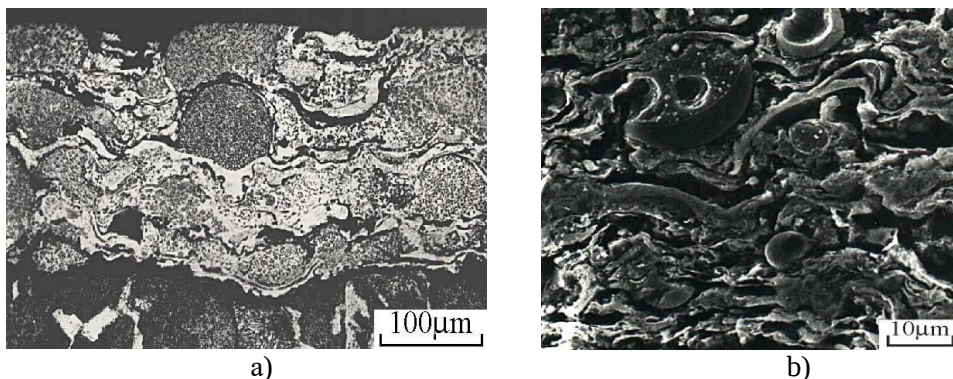
Fig. 2.7. Microstructure of the sprayed detonation eutectic coating CrVC (etched metal matrix): a) light microscope; b) SEM, etched metal matrix
