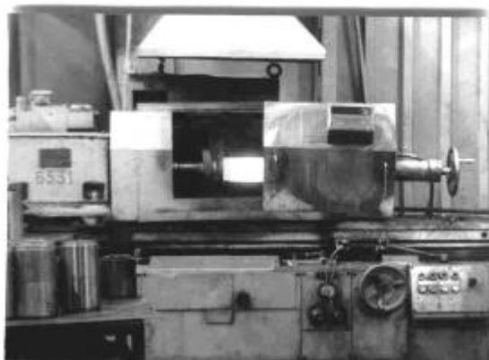
Fig. 3.15. Installation for centrifugal metallization with induction heating
