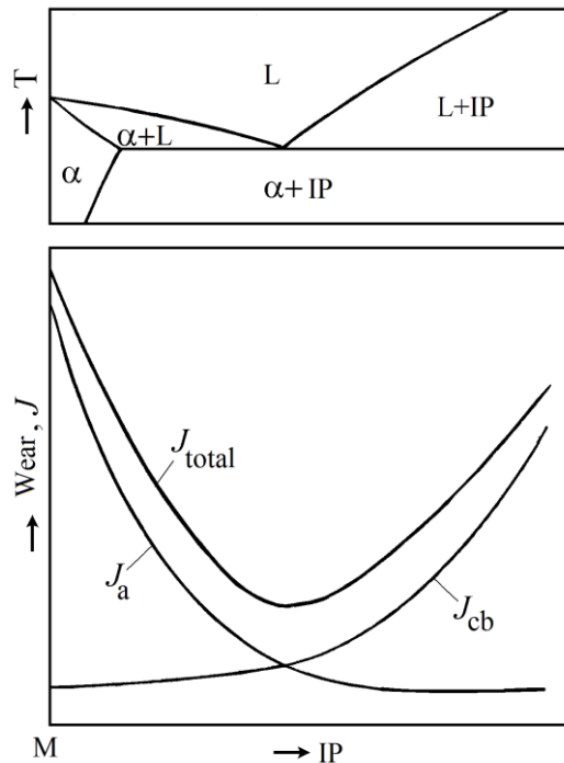
Fig. 1.7. Dependence of the alloy wear loss versus interstitial phase content (IP). J_a – alloy wear loss, J_{cb} – counterface wear loss, J_{total} – total wear loss of friction couple
