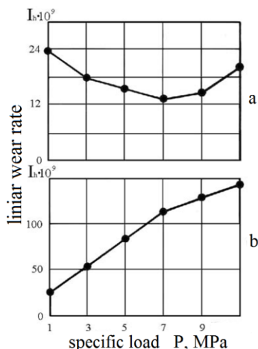
Fig. 2.9. Dependence of the linear wear rate on the specific load (slippage speed 0.25 m/sec): a) detonation coating VTiNi; b) counterbody (hardened steel 1080)
