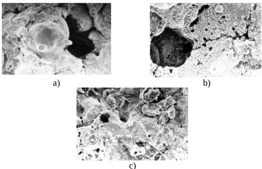
Fig. 3.14. Microfractures of coating surface after cavitation test during 10 hours, \times 600 : a) 12Cr18Ni9Ti-TiB 2 (plasma sprayed); b) 12Cr18Ni9Ti-TiB 2 -CrB 2 (laser treated); c) 12Cr18Ni9Ti-TiB 2 -CrB 2 (electro-spark alloying)
