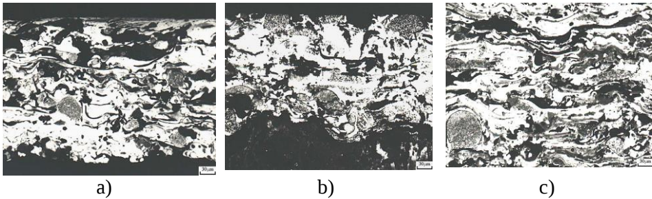
Fig. 2.4. Structures of plasma eutectic coatings (cross sections): a) VTiNi; b) CrTiNi; c) CrVC
