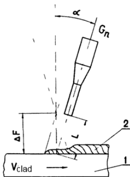
Fig. 3.23. Layout of laser cladding with the supply of powder in the direction of sample motion: 1 – sample; 2 – roller being cladded
