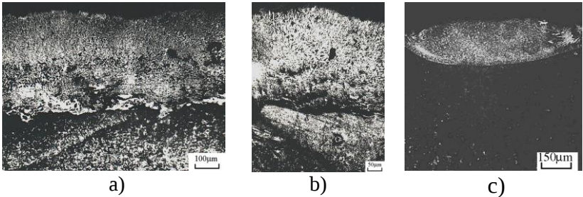
Fig. 2.18. Microstructure of laser melted gas-thermal coatings CrTiNi: a) plasma coating, the middle zone; b) plasma coating, the transition area; c) detonation coating
