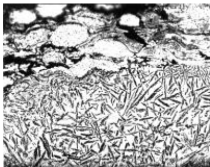
Fig. 3.12. Microstructure of bilayer coating on steel 12Cr18Ni9Ti (alloyed boride layer and plasma CrTiNi coating), \times 156
