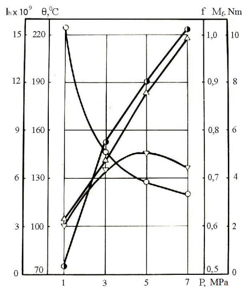
Fig. 2.5. Dependence of linear wear rate, I_h (∇); maximum temperature in contact, \theta (°C); friction factor, f (o), and friction moment, M_f (Δ) on the specific load. Material – plasma eutectic coating VTiNi (load conditions: V = 0,25 m/sec, counterface – hardened steel 1080)
