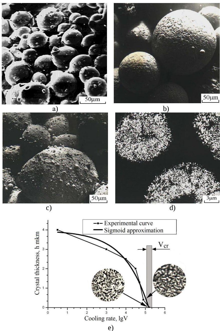
Fig. 2.3. The appearance of the eutectic powders formed by spraying with argon and nitrogen and the dependence of the structure on the cooling rate (e): a) VTiNi, argon; b) CrVC, nitrogen; c) VTiN, nitrogen; d) VTiN, argon
