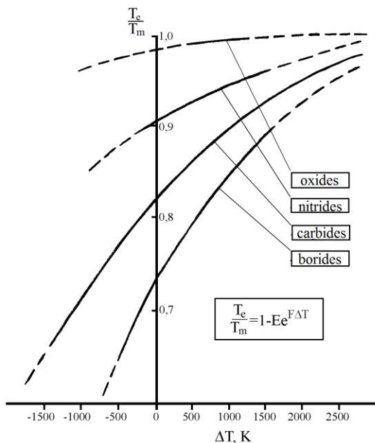
Fig. 1.3. The dependence of the quasi-binary metal-interstitial phase eutectic alloys melting point on the difference between the melting points of interstitial phase and the metal matrix
