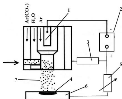
Fig. 3.20. Layout of plasma cladding using metallic powders: 1 – tungsten electrode; 2 – power supply; 3 – impedance resistance; 4 – coating; 5 – ballast resistance; 6 – the product; 7 – powder
