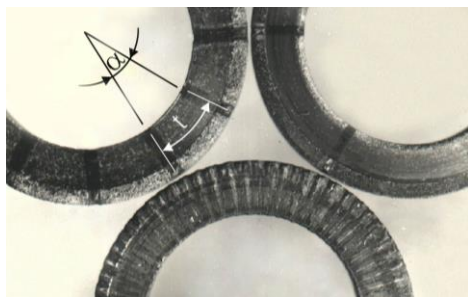
Fig. 2.17. The location and geometry of molten zones: t – the arc length between molten zones; \alpha – central angle between molten zones
