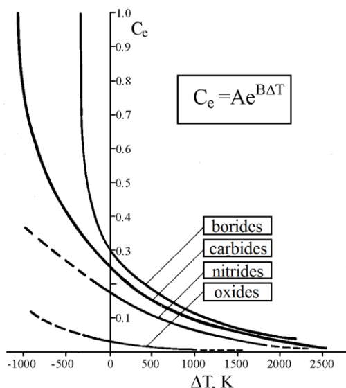
Fig. 1.2. The dependence of the quasi-binary metal-interstitial phase eutectic alloys composition ( C_e ) on the difference between the melting points of interstitial phase and the metal matrix ( \Delta T )
