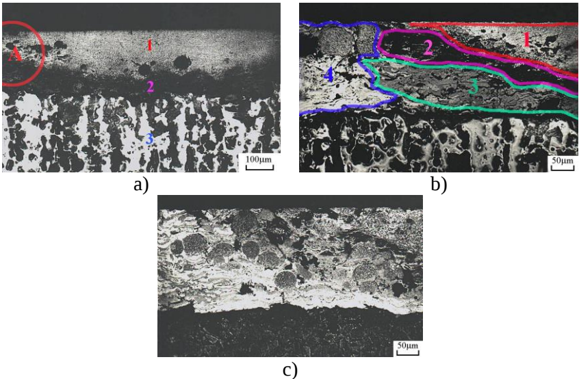
Fig. 2.19. Microstructure of remelted plasma coatings: a) VTiNi, 1 – zone of remelting, 2 – transition zone, 3 – substrate; b) VTiNi region A, 1 – zone of remelting, 2 – transition zone, 3 – heat affected zone, 4 – untreated coating; c) CrWSi coating
