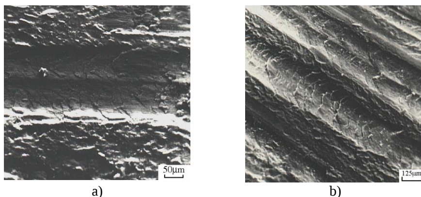
Fig. 2.15. Traces of plastic deformation on friction surface of annealed detonation coating VTiNi: a) annealing 18 \times 10^2 sec; b) annealing 18 \times 10^3 sec. SEM
