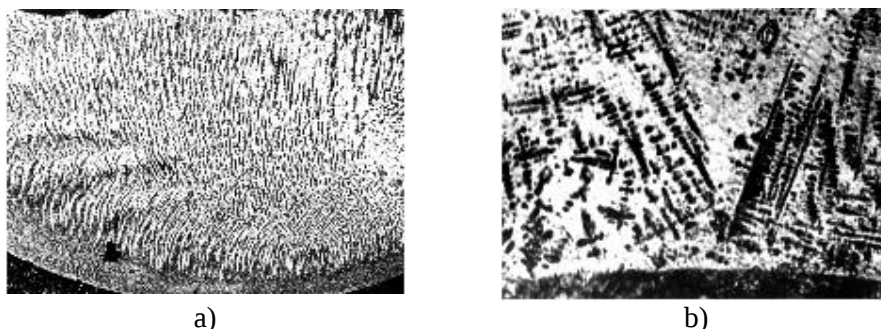
Fig. 3.3. Microstructures of laser clad coatings a) TiNi and b) VTiNi, \times 156
